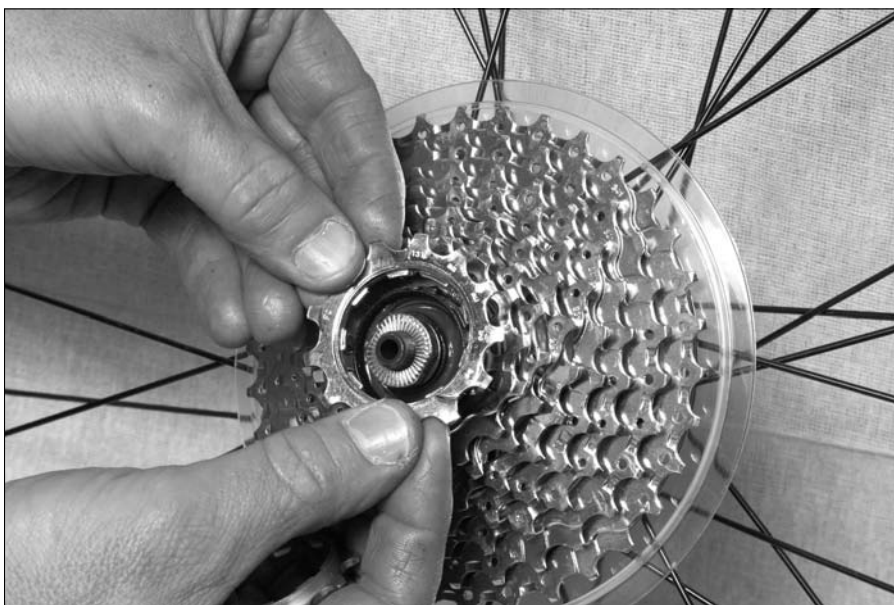
Figure 11-5: Removing the cogs on a cassette
