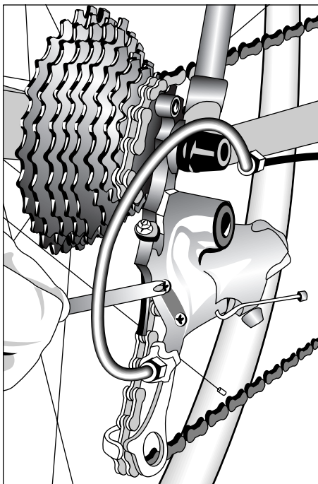
Figure 4-6: The H-limit screw.
