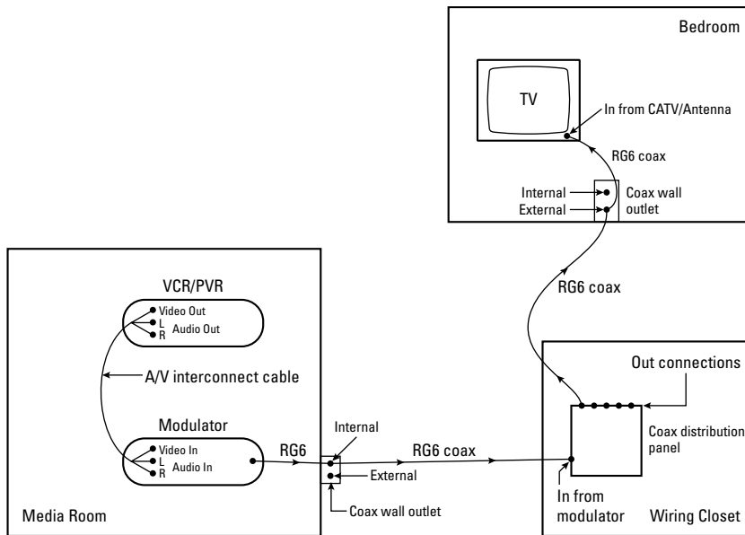
Figure 7-3: Watching a VCR or PVR in another room.
