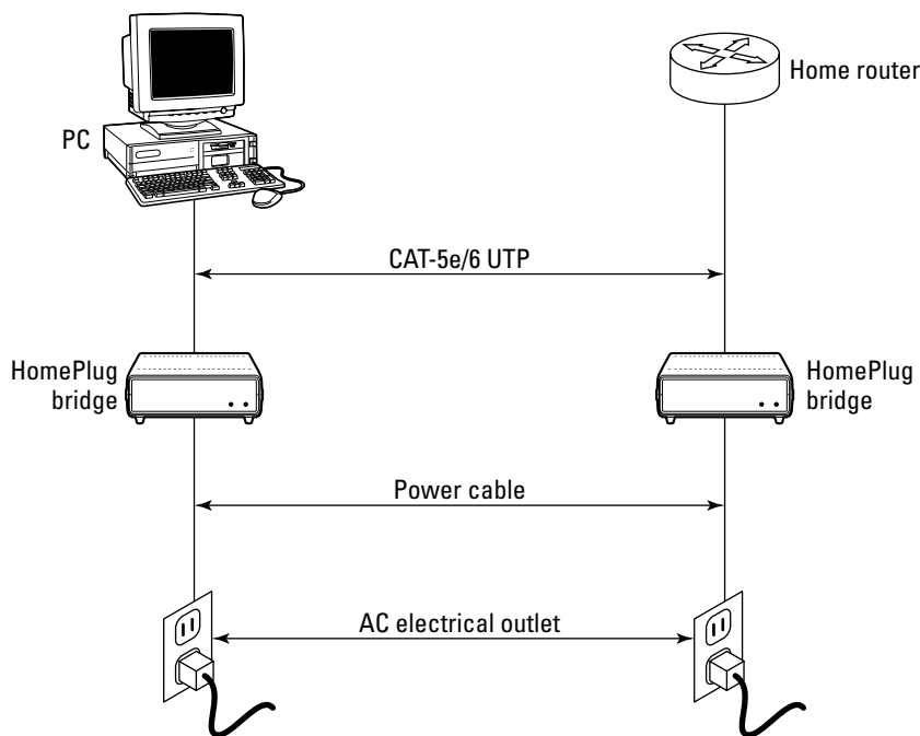
Figure 16-3: Plugging your computer into the wall — and that's all.
