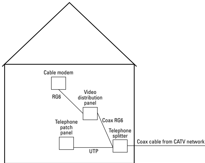
Figure 10-2: A voice- over-cable network.
