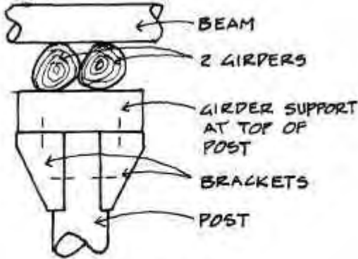
DRAWING ABOVE SHOWS ONE METHOD OF SUPPORTING 2 GIRDERS WITH SINGLE POST. NOTE: WOOD IS ACCEPTABLE MATERIAL FOR BRACKETS AND GIRDER SUPPORT.
