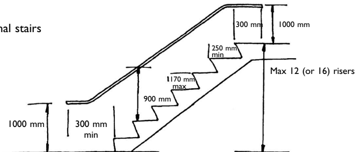
Figure 14.2 Other options for vertical circulation within the building.
