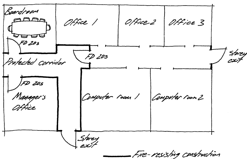
Figure 4.7 Dead-end corridor.
