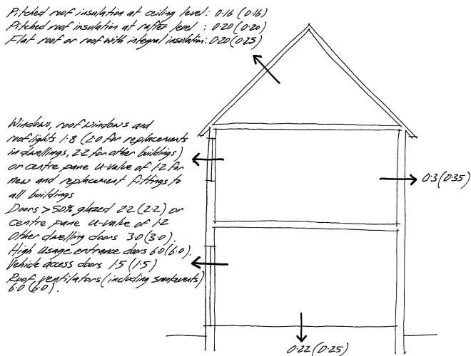
Figure 13.2 U-value standards for new and replacement thermal elements and controlled fittings in existing dwellings and buildings other than dwellings ( \text{W/m}^2\text{K} )
