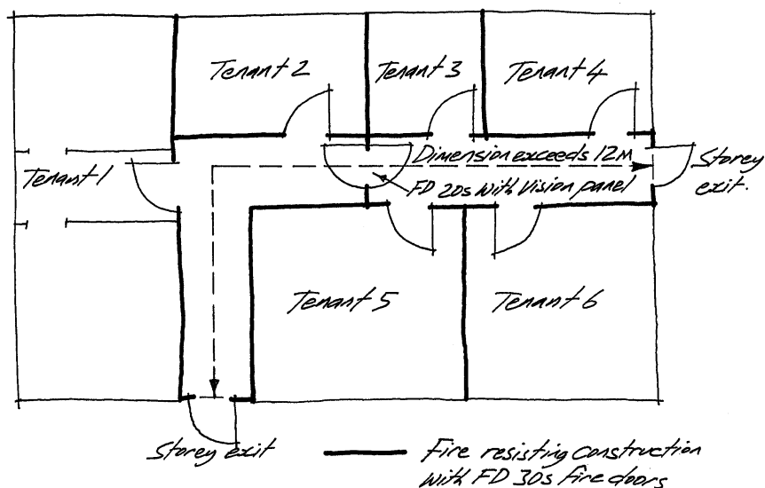
Figure 4.6 Protected corridor.
