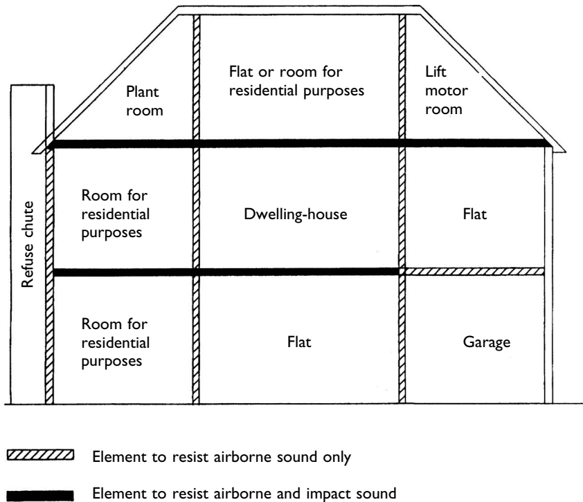
Figure 7.2 Walls and floors required to offer sound resistance (Requirement E1).
