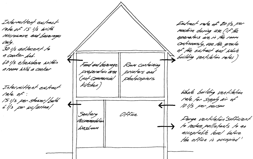
Figure 8.2 Ventilation rates for offices.
