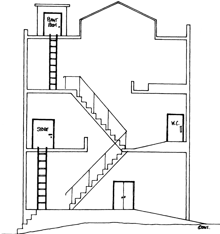
Figure 12.1 Application of stair and ramp provisions.
