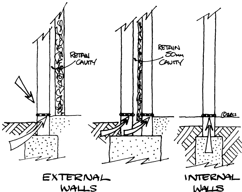
Figure 5.4 Provisions for walls.
