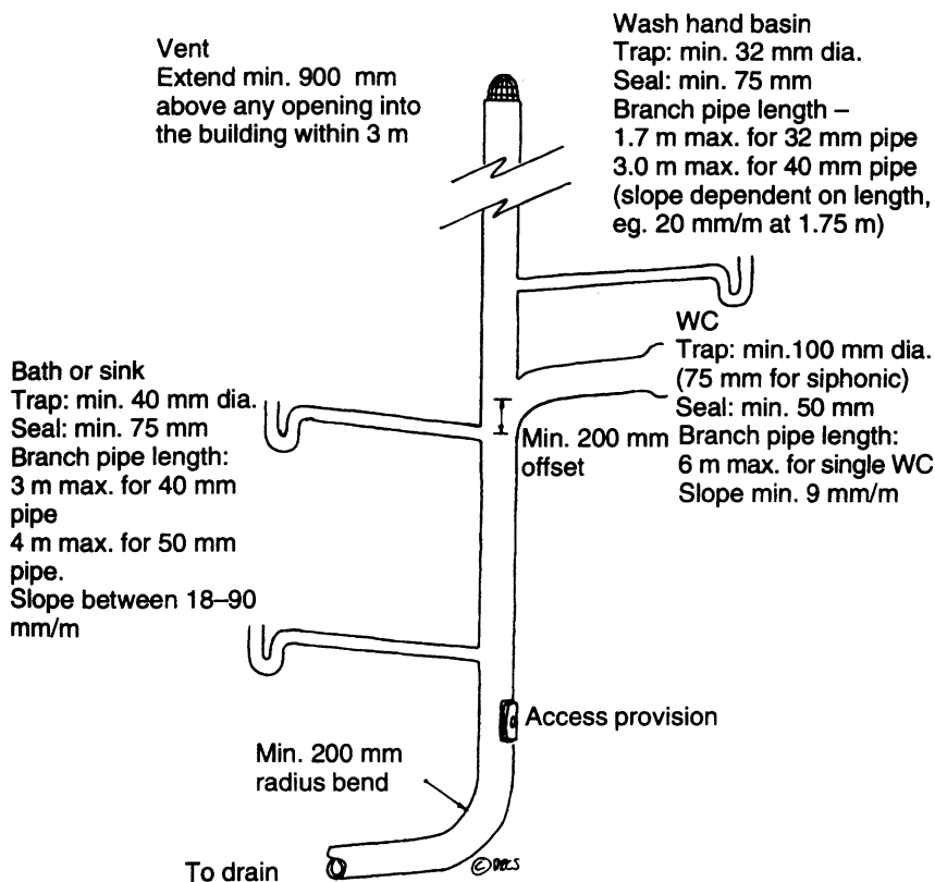
Figure 10.1 Discharge stack (S&VP) and branch pipes.
