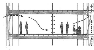
Fig. 7.2 GSW Headquarters: diagram showing cross-ventilation.
