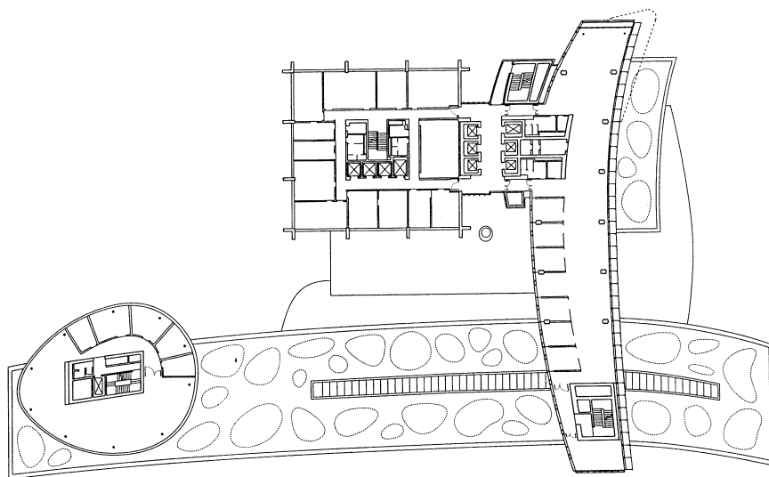
Fig. 7.1 GSW Headquarters: third floor plan.
