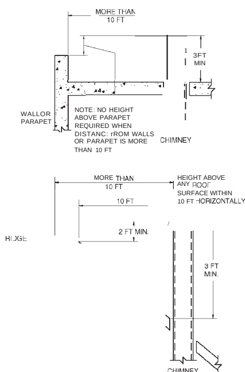
S. TERMINATION MORE THAN 10 FT FROM RIDGE, WALL, OR PARAPET
