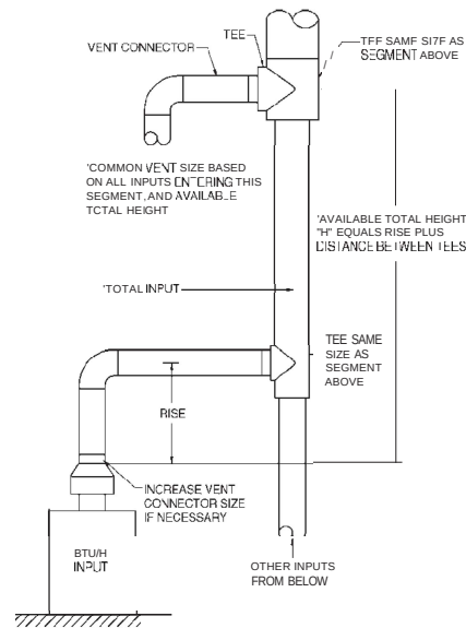
Vent connector size depends on: • Input • Rise • Available total height " H " • Table 504.3(1) connectors Common vent size depends on: • Combined inputs • Available total height " H " • Table 504.3(1) common vent
