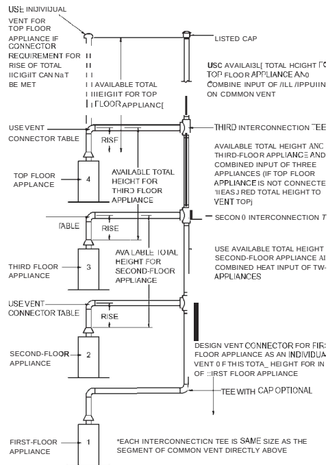
Principles of design of multistory vents using vent connector and common vent design tables (see Sections 504.3.11 through 504.3.17).
