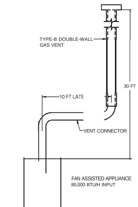
FIGURE 8-16 (EXAMPLE 2) SINGLE FAN-ASSISTED APPLIANCE
