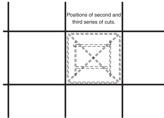
Figure 5.31 Diagram to illustrate removal of damaged historic tiles.
