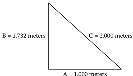
Structure 2-6
