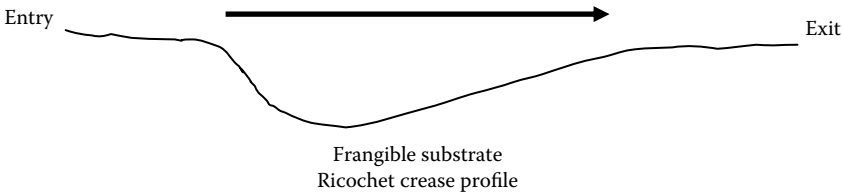
Structure 10-8
