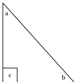
Structure 2-4
