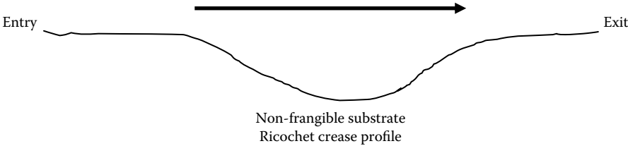
Structure 10-7
