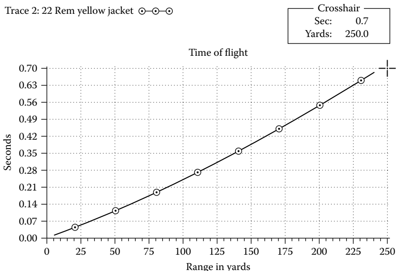
Figure 15.8 Ballistic Explorer graph of time of flight. (Courtesy of Forensic Science Associates. With permission.)
