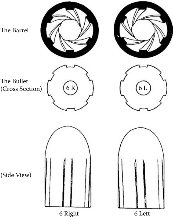
Figure 3.2 Cut rifling.
