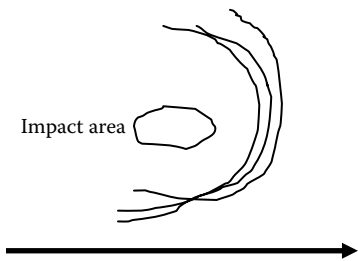
Structure 10-9
