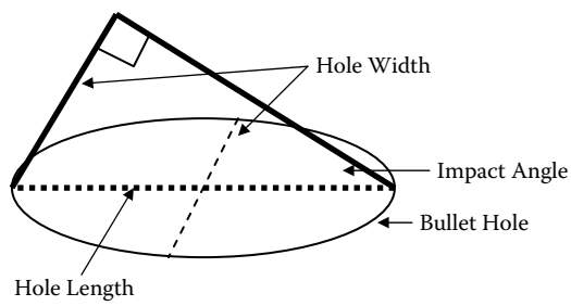
Structure 2-13
