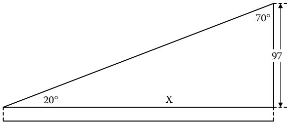
Structure 2-20
