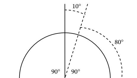
Structure 2-1
