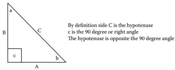
Structure 2-7
