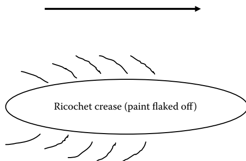
Structure 10-3
