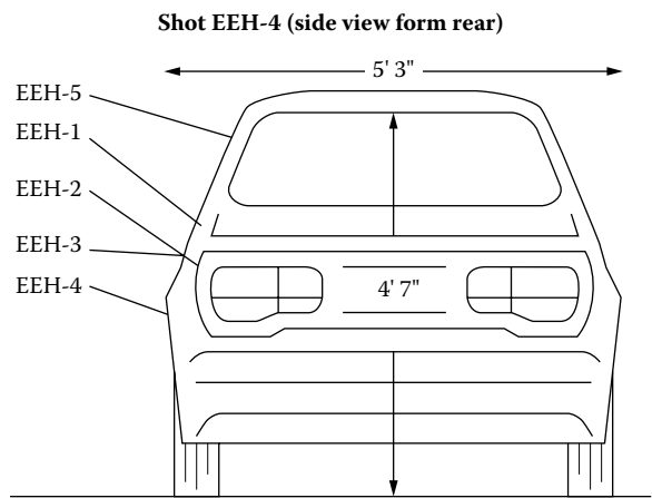
Figure 15.2 CADZone vehicle, profile view.
