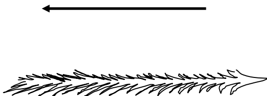
Structure 10-4
