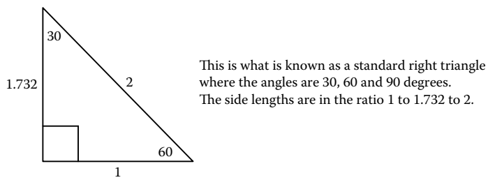
Structure 2-8
