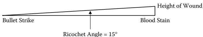
Structure 2-15
