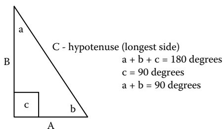
Structure 2-5
