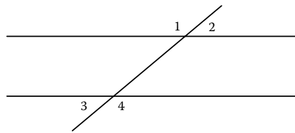
Thus, angles 1 & 3 are equal and angles 2 & 4 are equal
