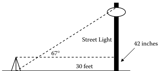
Structure 2-17
