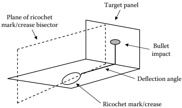
Structure 10-11
