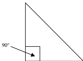
Structure 2-3
