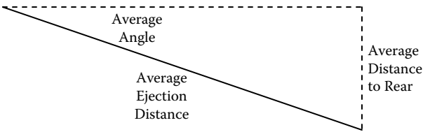
Structure 2-22
