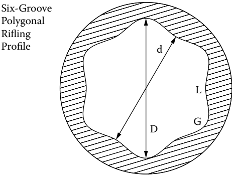
Figure 3.3 Polygonal rifling.
