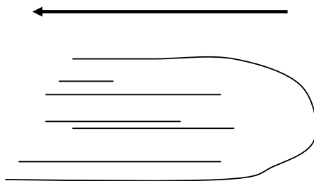
Structure 10-5
