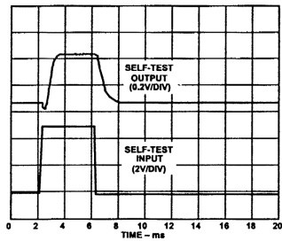
Figure 10. Typical Self-Test Response
