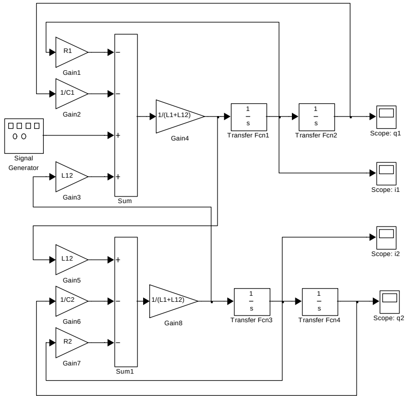
Figure 2.3.10. SIMULINK diagram
