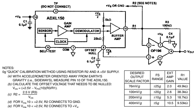
Figure 17. "Quick Zero g Calibration" Connection
