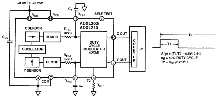
Figure 13. Block Diagram
