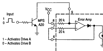
Figure 22. Digital Two Position Servo System
