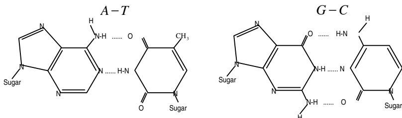
Figure 2.1.6. DNA pairing due to hydrogen bonds
