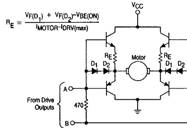
Figure 30. Power H-Switch Buffer
