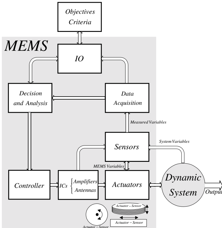
Figure 1.4.2. High-level functional block diagram of large-scale MEMS with rotational and translational actuators and sensors
