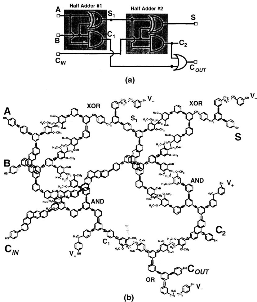
Figure 2.6.8. Molecular circuit and schematics of molecular full adder [2]
