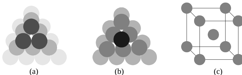
Figure 3.1.5. Close packing of metal atoms: a) cubic packing; b) hexagonal packing; c) body-centered cubic
