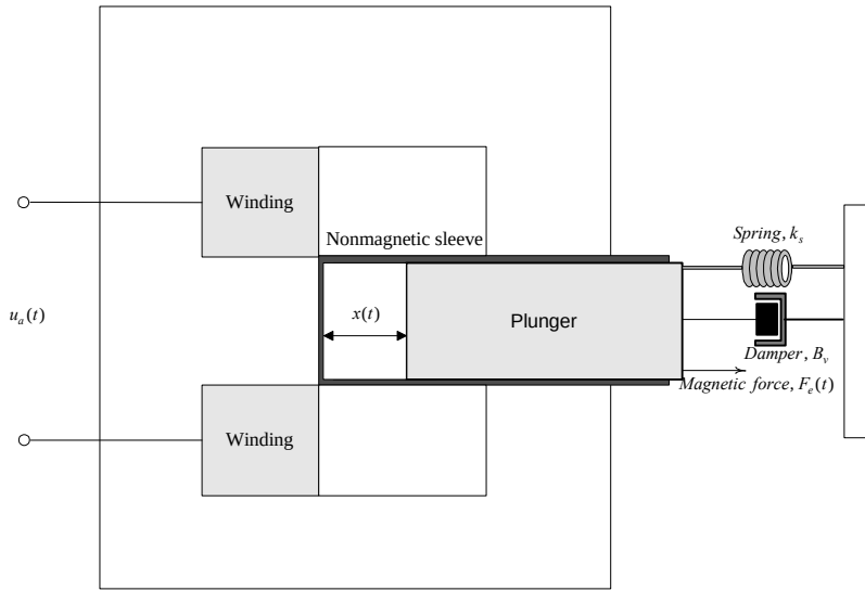
Figure 2.3.6. Schematic of a transducer
