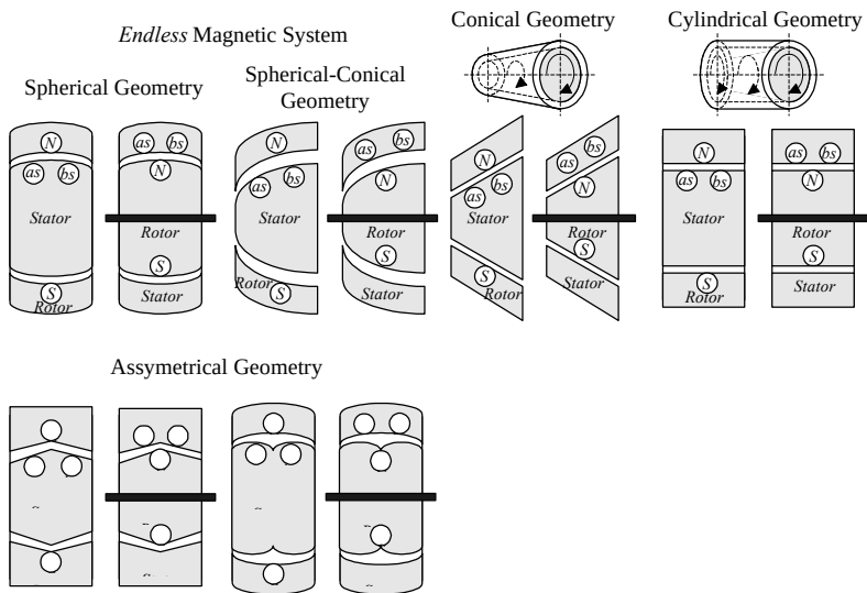
Figure 3.2.1. Synthesized microscale actuator/sensor geometry
