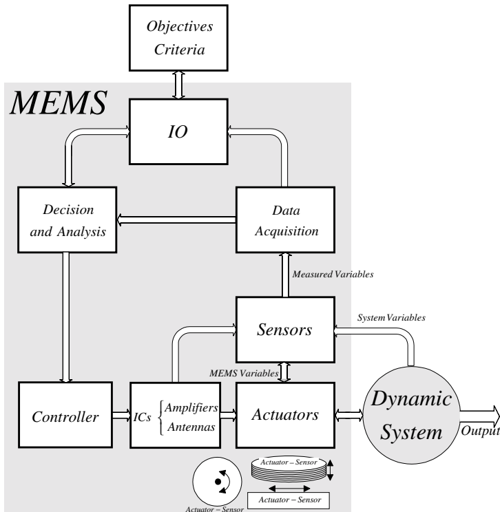
Figure 2.1.4. High-level functional block diagram of large-scale NEMS and MEMS
