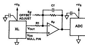
c. Single-Pole Post Filtering and Signal Amplification
