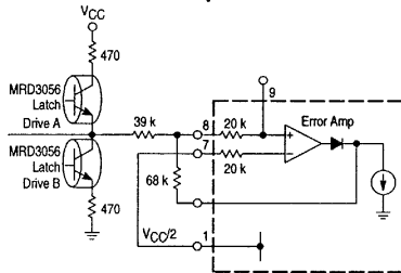
Figure 21. Infrared Latched Two Position Servo System
