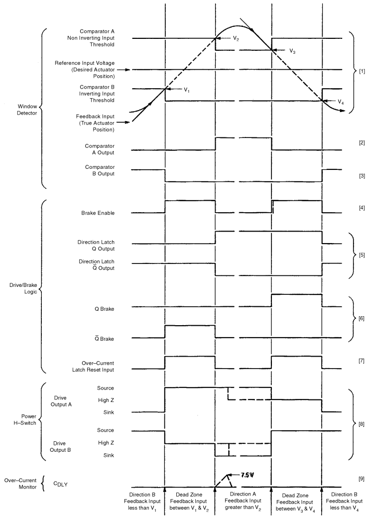
Figure 18. Timing Diagram
