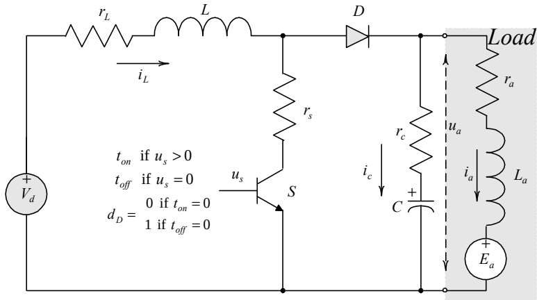
Figure 2.3.13. Boost converter
