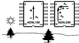
Figure 2. Output Polarity
