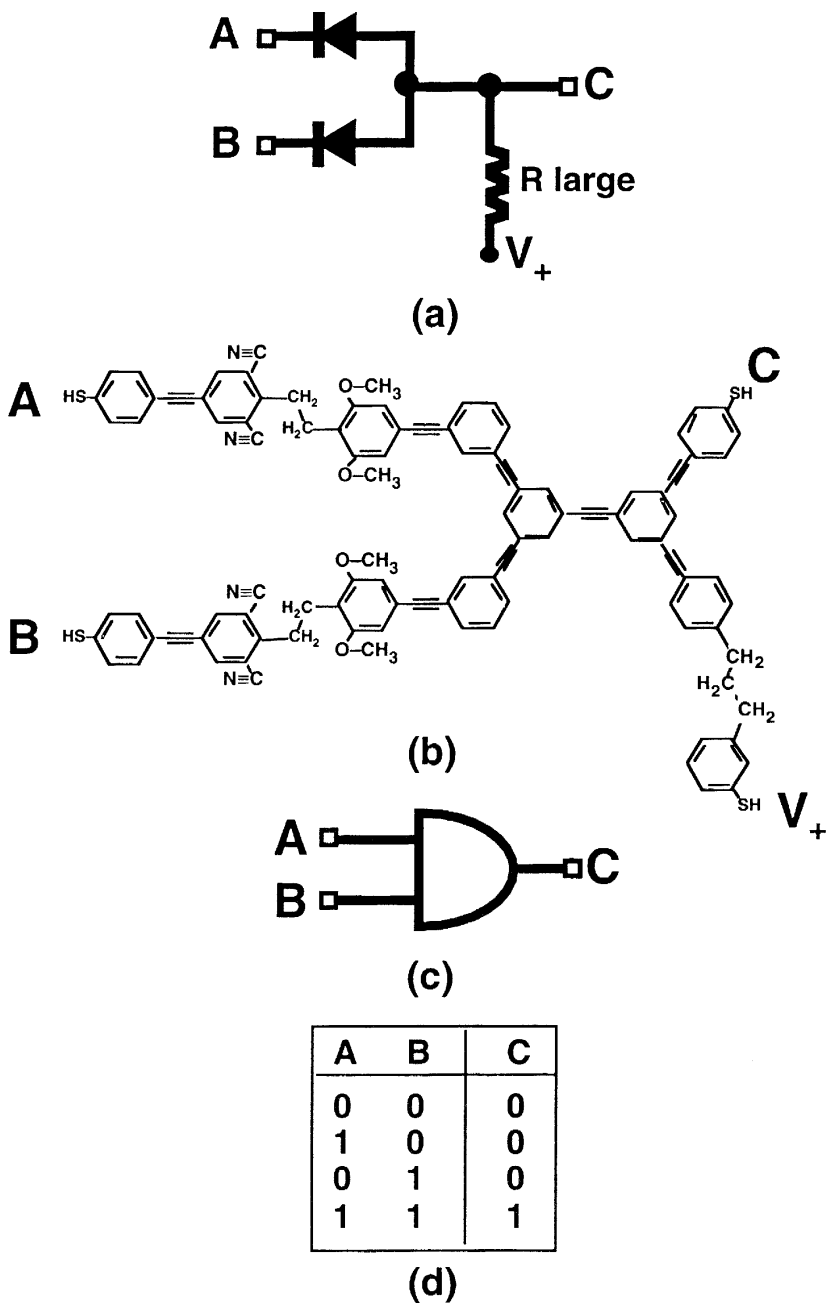
Figure 2.6.4. Molecular circuit and schematics of AND molecular gate [2]
