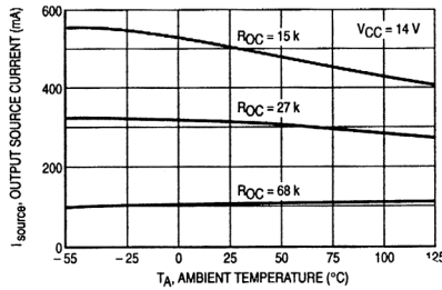
Figure 9. Output Source Current–Limit versus Temperature
