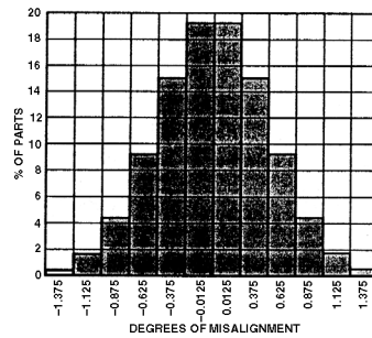
Figure 11. Rotational Die Alignment
