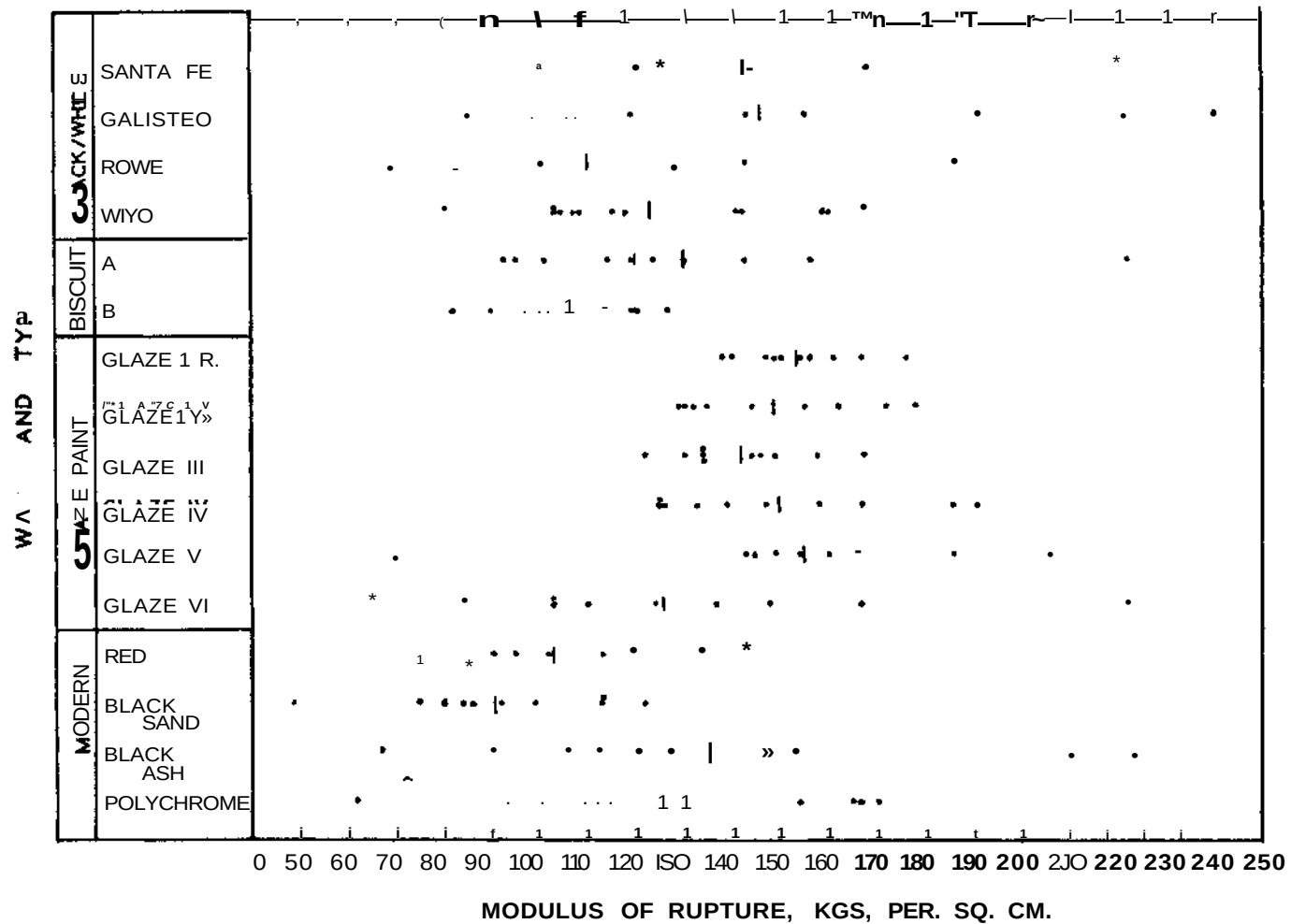
FIG. 14- DATA ON TRANSVERSE BREAKING, STRENGTH OF POTTERY TYPES FROM PECOS, NEW MEXICO
