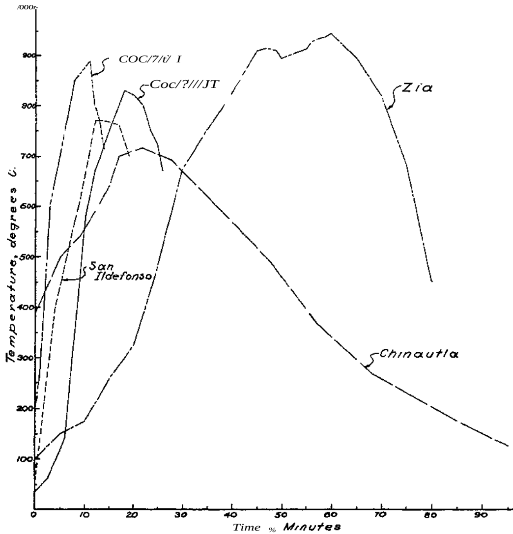
FIG. S-TEMPERATURE CURVES FOR FIRING OF OXIDIZED WARE
