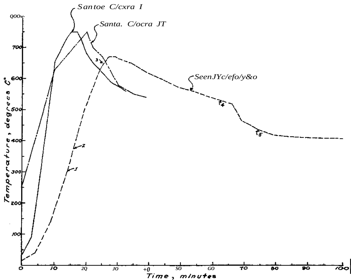
FIG. 6—TEMPERATURE CURVES FOR FIRING OF PUEBLO SMUDGED WARE
