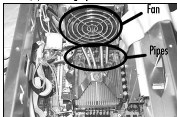
Figure 6.28 The Shuttle Heatpipe Cooling System
