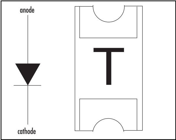
Figure 12.2 Schematic Symbol and Physical Outline of an LED
