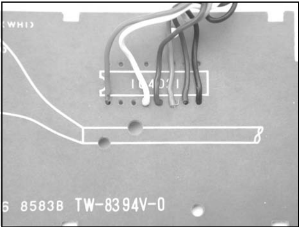
Figure 7.19 Wiring Complete
