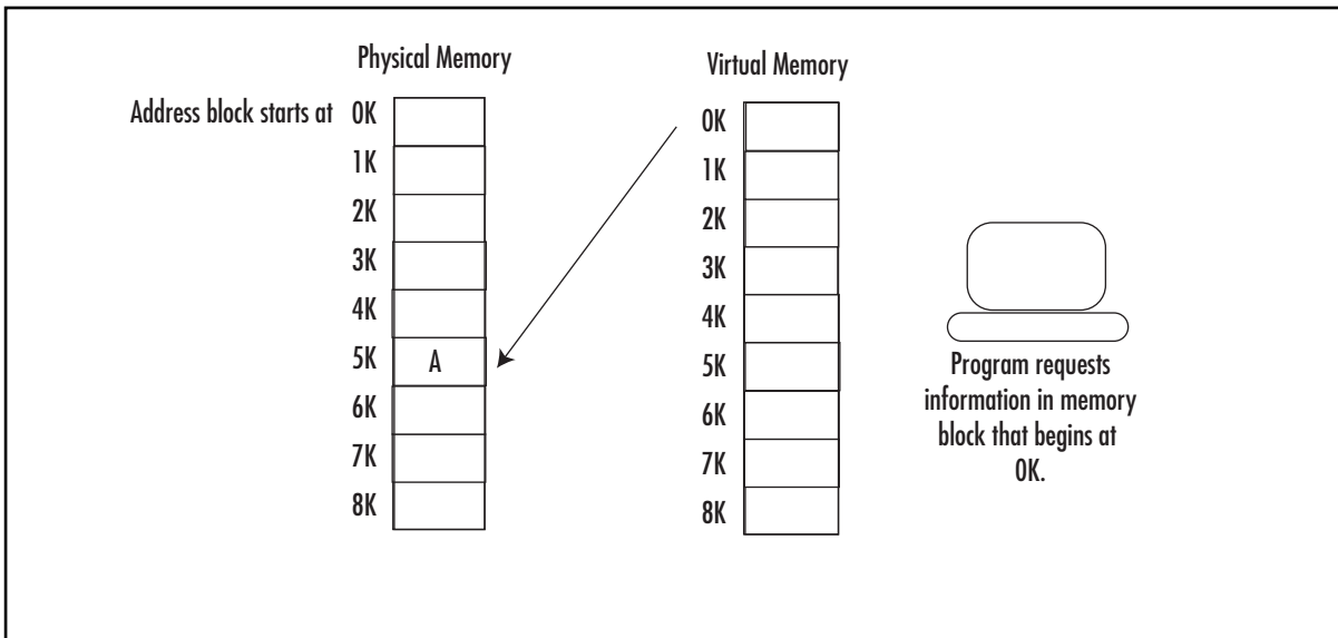
Figure 14.2 Memory Management with Virtual Memory
