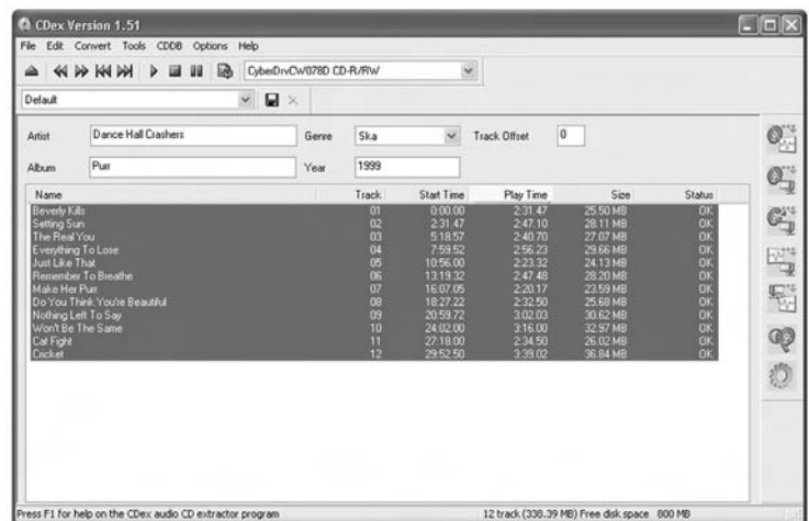
Figure 6.17 The CDex Main Interface Page
