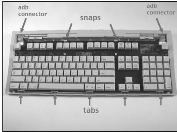
Figure 5.22 Removing the Keyboard Mechanism
