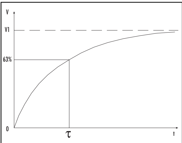
Figure 2.14 Capacitor-Charging Curve
