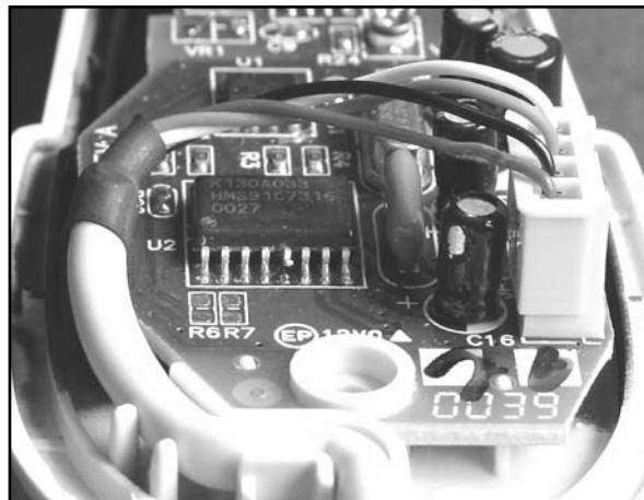
Figure 3.37 Hack Complete: Pin 5 of Microprocessor Lifted (Close-Up)
