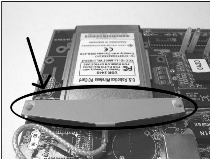
Figure 10.15 Before Removing the Card ... See the Metal Brace?
