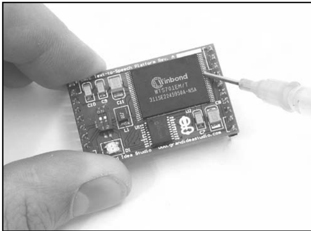
Figure 2.35 Applying Flux to the Leads
