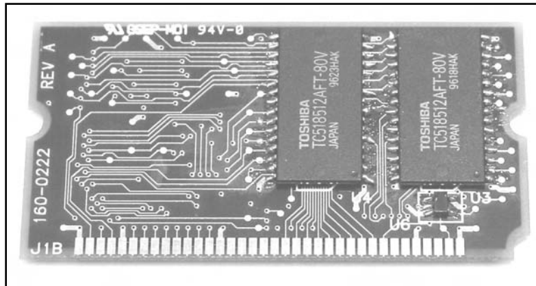
Figure 13.21 Hacked PalmPilot Professional Memory Card With 2MB RAM, Back
