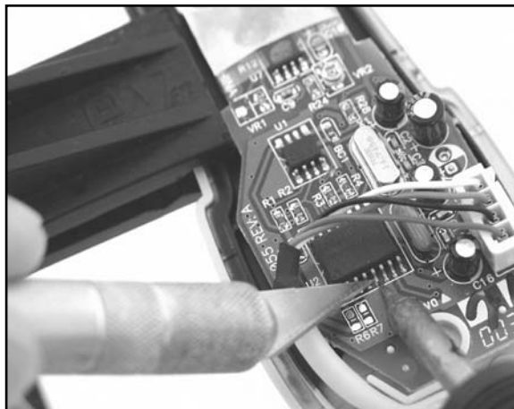
Figure 3.36 Heating and Lifting the Pin of the Microprocessor
