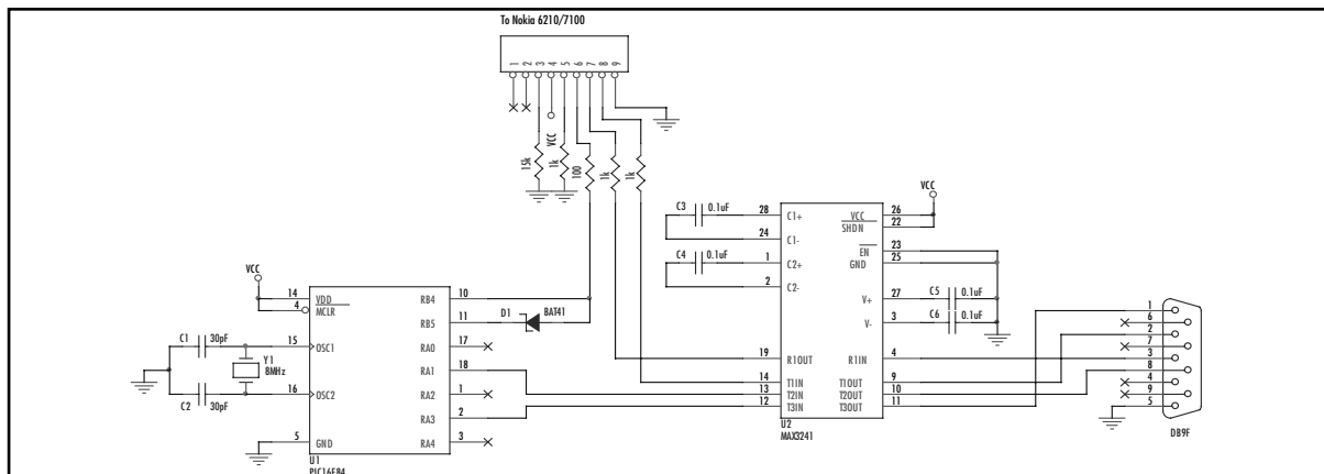
Figure 12.25 Schematic for a DLR-3P Cable by Adrian Dabrowski, www.atrox.at/datacable
