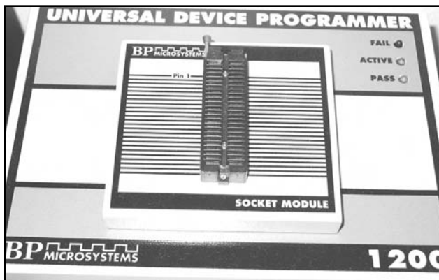
Figure 1.12 Device Programmer
