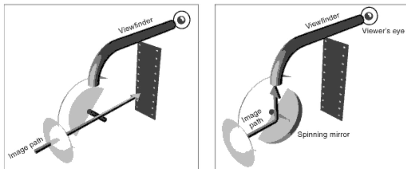
FIGURE 6.16 The film camera spinning mirror shutter open (left) and closed (right).
