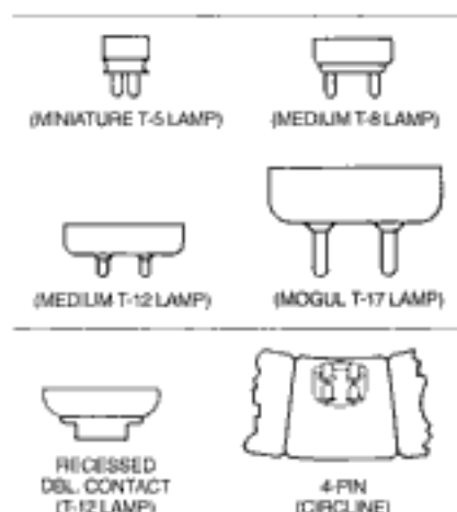
FIGURE 11.7 Bases for fluorescent lamps. (Courtesy of GTE-Sylvania Lighting.)
