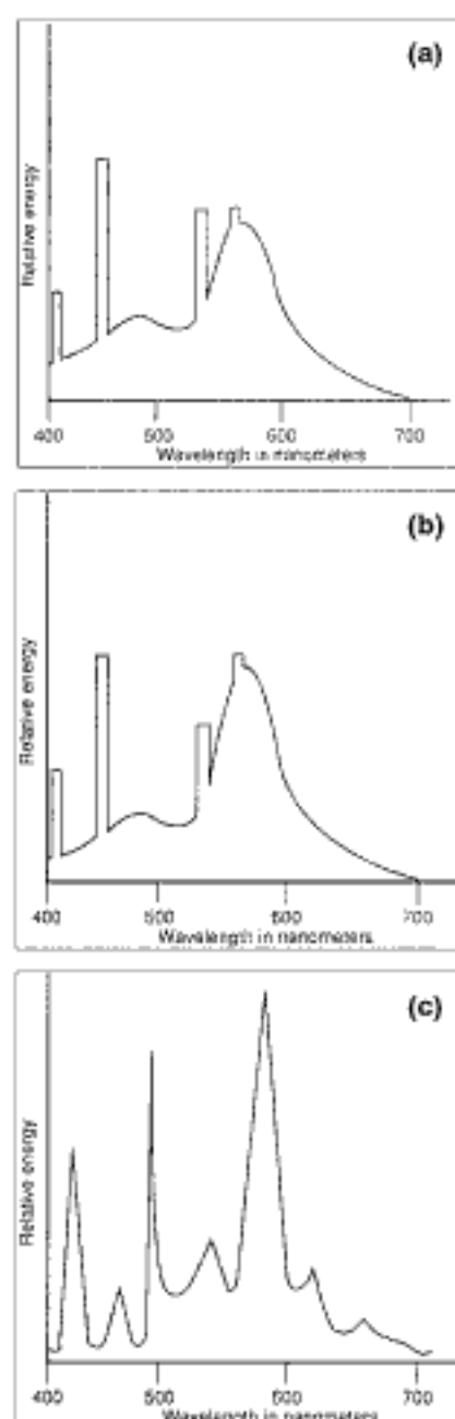
FIGURE 11.9 (a) SED (spectral energy distribution) of a cool white fluorescent. (b) Warm white fluorescent SED. (c) Warm white deluxe fluorescent.
