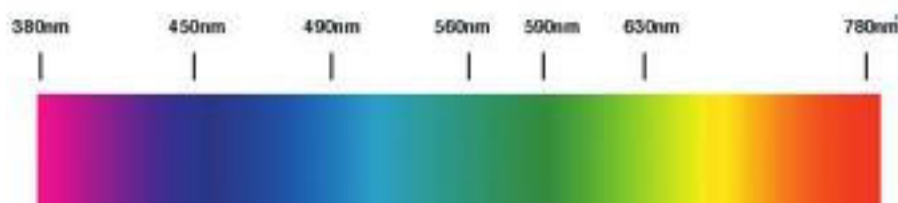
FIGURE 7.1 The naturally occurring color spectrum and respective wavelengths in nanometers.
