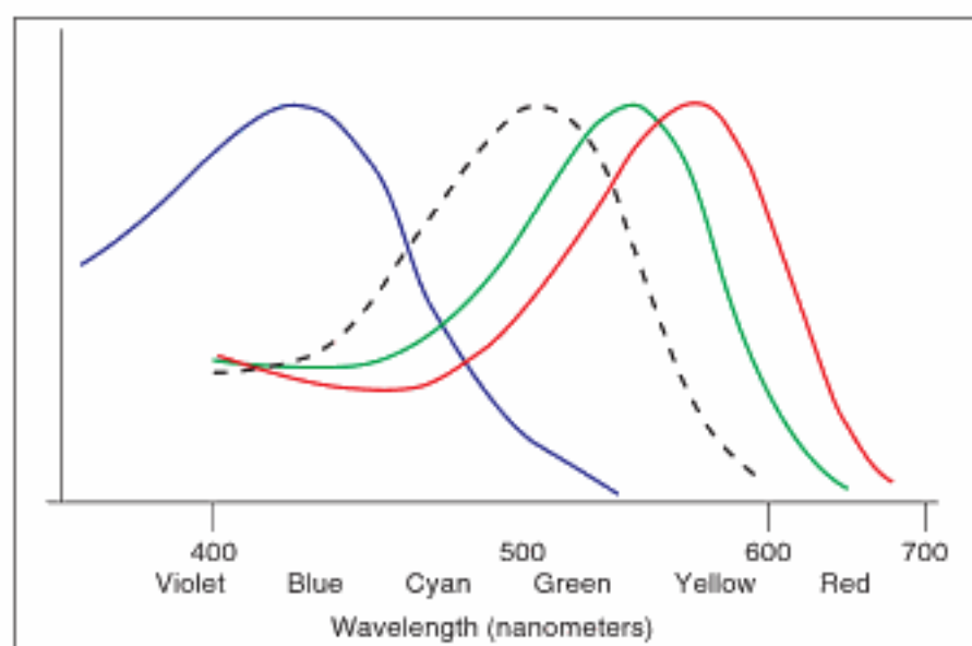
FIGURE 7.4 Color response of the red, green, and blue cones in the eye. The dashed line represents the response of the rods.
