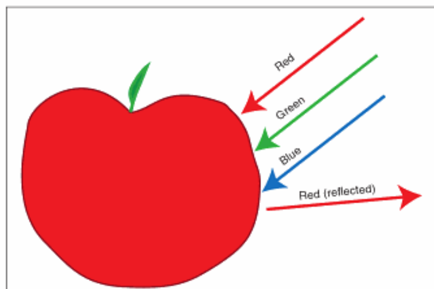
FIGURE 7.2 The color of an object is determined by what parts of the spectrum it reflects.
