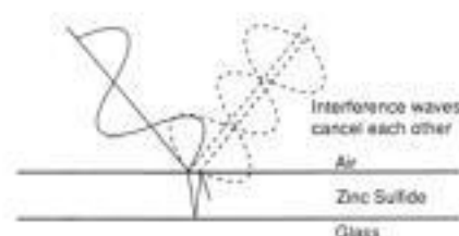
FIGURE 11.11 Dichroic filter operating principles.
