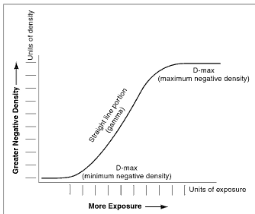
FIGURE 6.6 The Hurter and Driffield D \log E curve for negative density.
