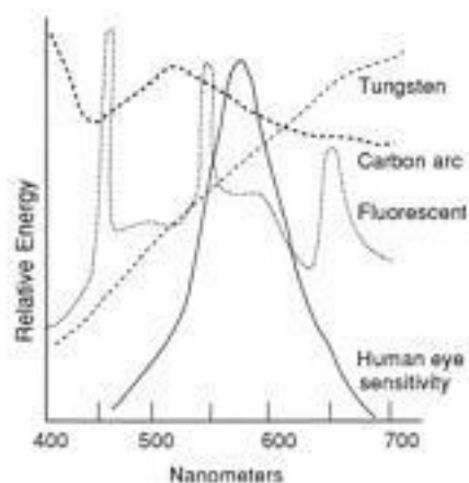
FIGURE 11.1 SED of typical sources.
