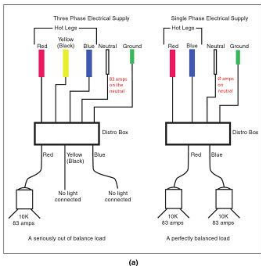
FIGURE 8.10 (a) Balanced and unbalanced loads. One is single-phase and the other three-phase for purposes of illustration only: the same principles apply to both systems. (b) Distribution plan for a studio shoot.
