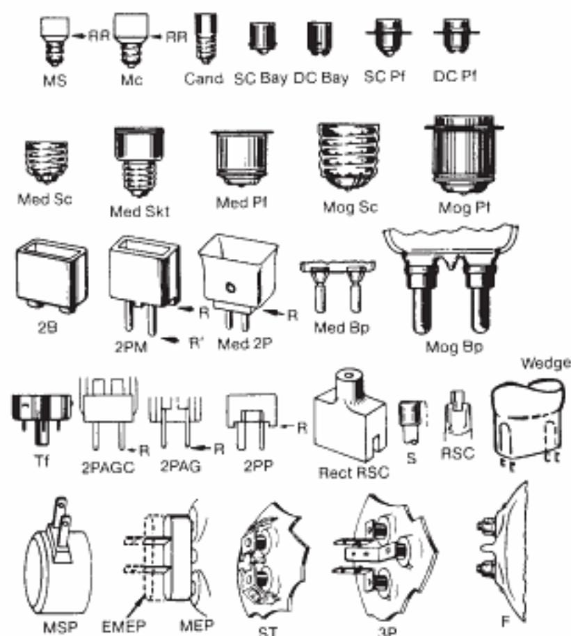
FIGURE 11.5 Bulb base codes. (Courtesy of General Electric.)
