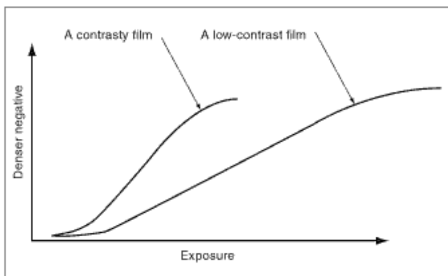
FIGURE 6.8 Differences between a high-contrast and a low-contrast film.
