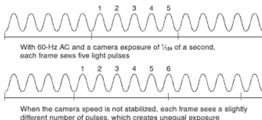
FIGURE 12.1 When the relationship of the shutter and the light output varies, each film frame sees a slightly different number of pulses.
