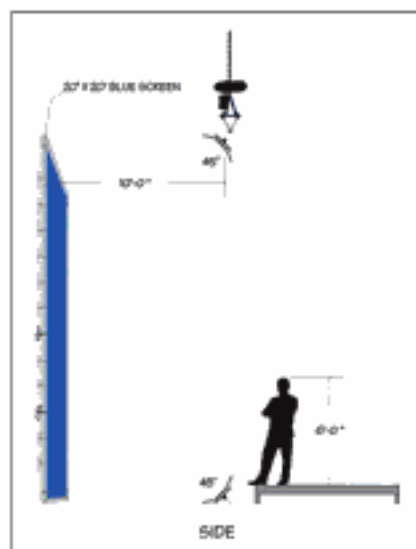
FIGURE 12.8 Kino Flo's recommendations for lighting process shot backgrounds; a 20 x 20 background is just an example. It is important to have the largest background possible for any particular shot. This keeps the foreground subject as far away from the background as possible in order to prevent backslash, which gets the background color onto the edges of the subject—a real problem. (Courtesy of Kino Flo, Inc.)
