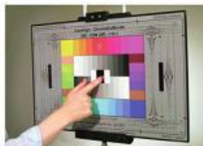
FIGURE 5.9 The Chroma du Monde test chart by DSC Laboratories. Its key features are two 11-step crossed grayscales in the middle, reference color chips, and in the center, the Cavi Black—a hole with black velvet behind it for true reference black. On each side of the Cavi Black are two 100 IRE white patches. (Photo courtesy of DSC Laboratories.)
