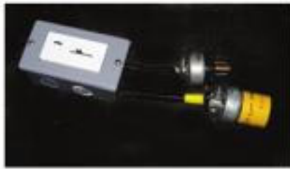
FIGURE 10.4 A hand-squeezer—a small dimmer for practical lamps, efx, and lights of 1000 watts or less.
