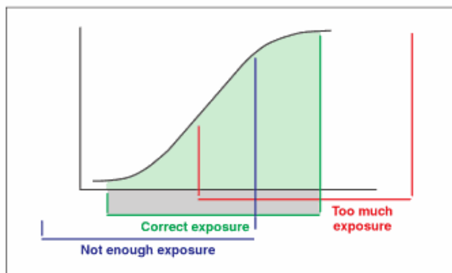
FIGURE 6.11 Changing exposure shifts the image up and down the curve; too much exposure pushes it off the shoulder, and too little crushes it into the toe.
