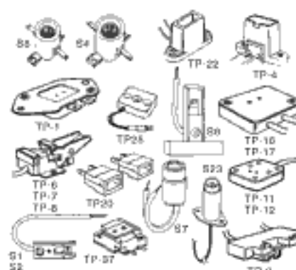
FIGURE 11.8 Typical lampholders for fluorescent lamps. (Courtesy GTE-Sylvania Lighting.)
