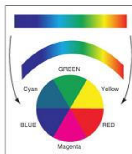
FIGURE 7.9 The derivation of the color wheel from the spectrum—as devised by Newton.
