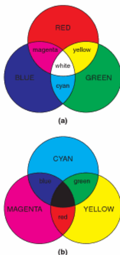
FIGURE 7.5 (a) Additive color. (b) Subtractive color.
