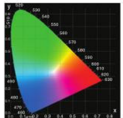
FIGURE 7.14 A diagram of the CIE color system.
