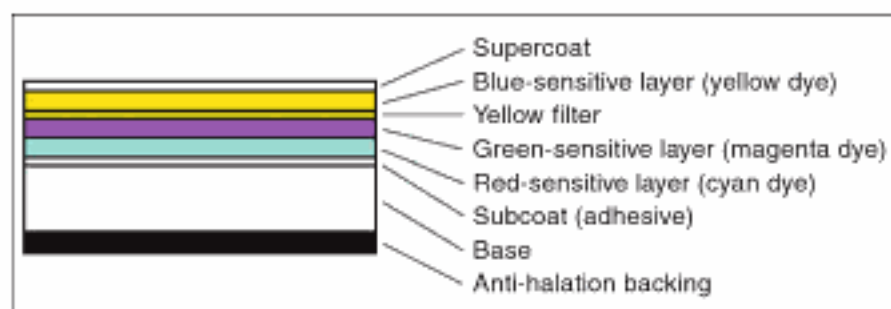
FIGURE 6.4 The layers of color negative film.
