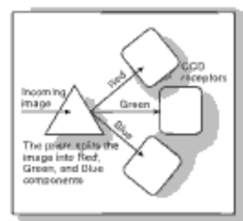
FIGURE 6.3 The image-capture section of a 3-chip video or HD camera.
