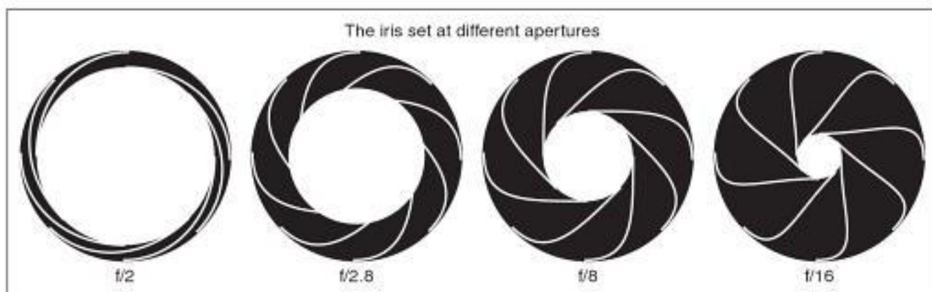
FIGURE 6.1 The aperture at various f/stops.
