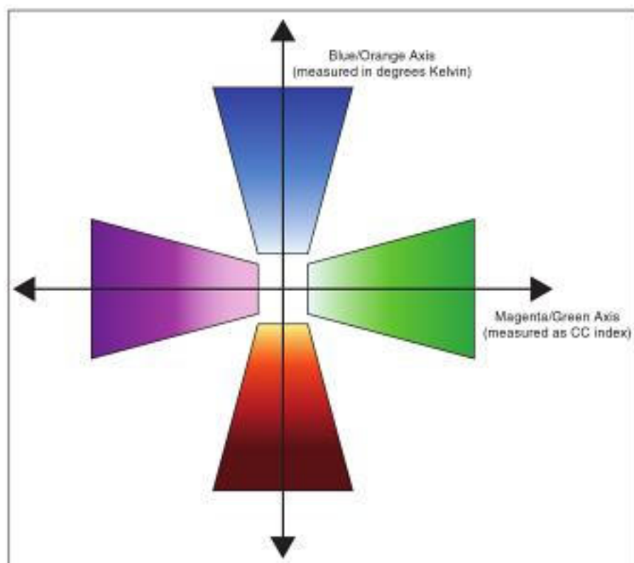
FIGURE 7.18 Color of light is measured along two independent axes—one for red/blue and another for green/magenta.
