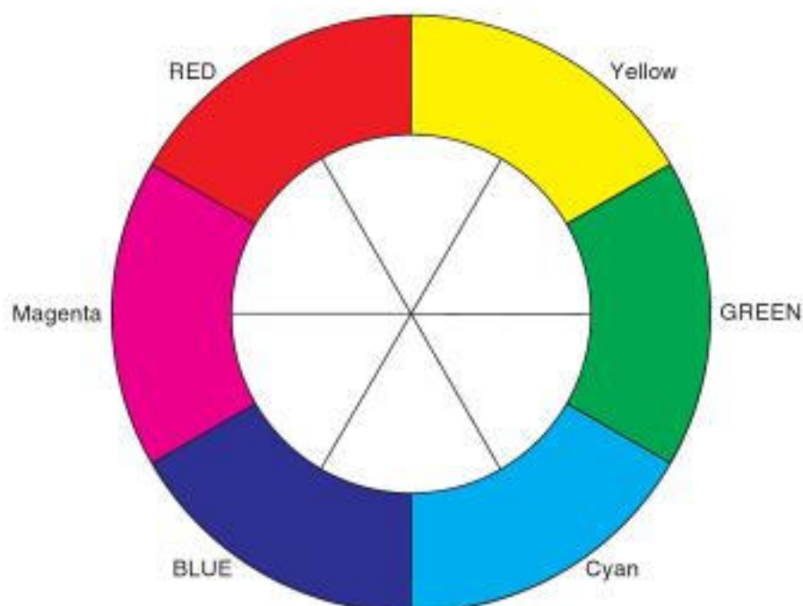
FIGURE 7.10 The primary and secondary colors arranged in the traditional color wheel.
