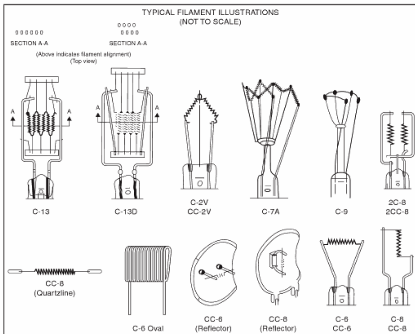
FIGURE 11.4 Common incandescent filament forms. (Courtesy General Electric.)
