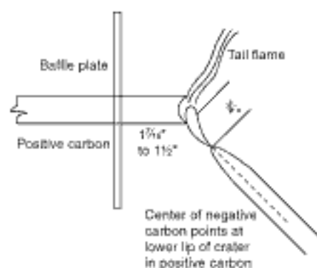
FIGURE A.1 Proper spacing of the carbons in an arc light.
