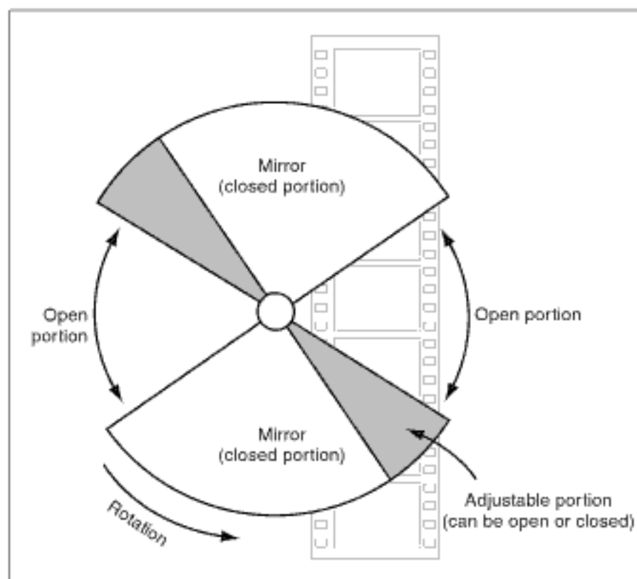
FIGURE 6.17 The spinning mirror shutter (butterfly type).
