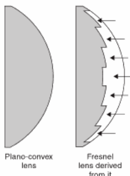
FIGURE 2.1 The derivation of the fresnel lens.
