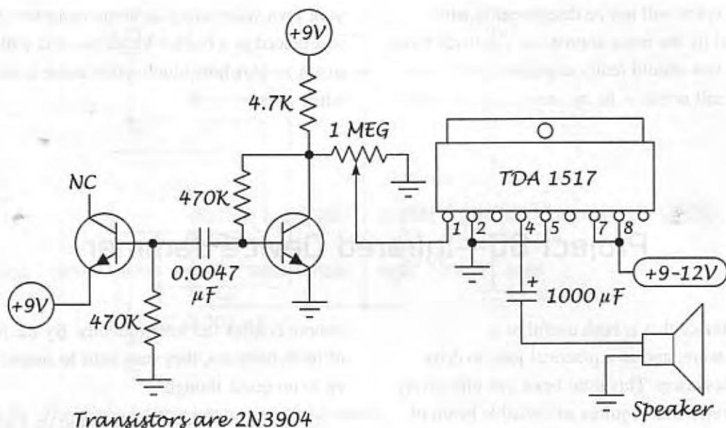
Figure 13-6 Schematic for a white noise generator with amplifier.
