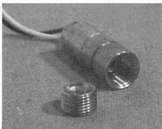
Figure 8-14 An 850-nanometer infrared laser module with adjustable lens removed.
