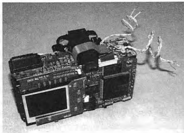
Figure 4-4 Wiring modifications for both the battery pack and trigger switch.
