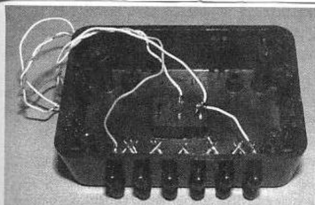
Figure 8-23 Infrared LED illuminator box and switch ready for installation.
