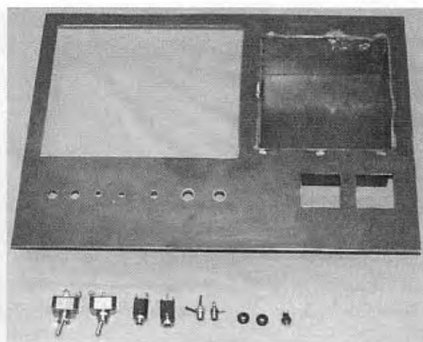
Figure 15-25 A dashboard made of steel sheet for the remote base station.
