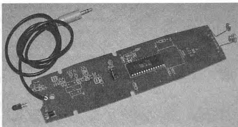
Figure 14-24 Replacing the infrared LED with a shielded signal cable and connector.
