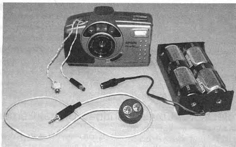
Figure 4-5 Wiring modifications completed for external power and trigger switch.
