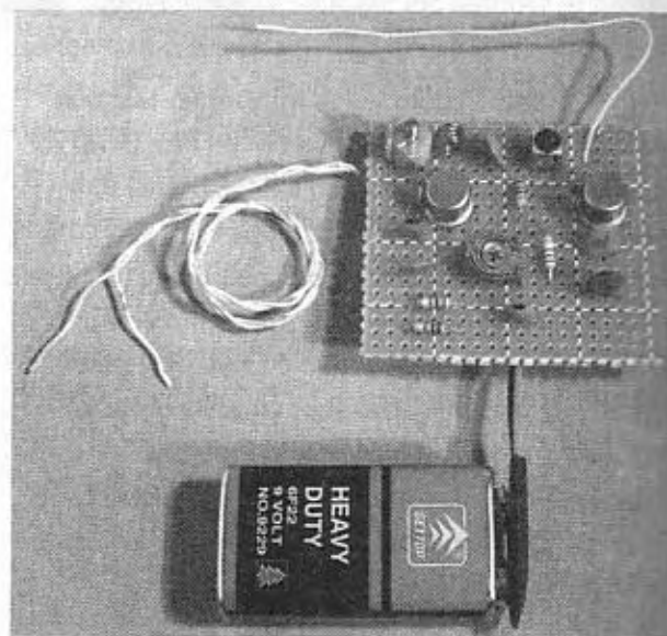
Figure 10-9 The audio video transmitter built on a \frac{1}{2} inch perf board for testing.
