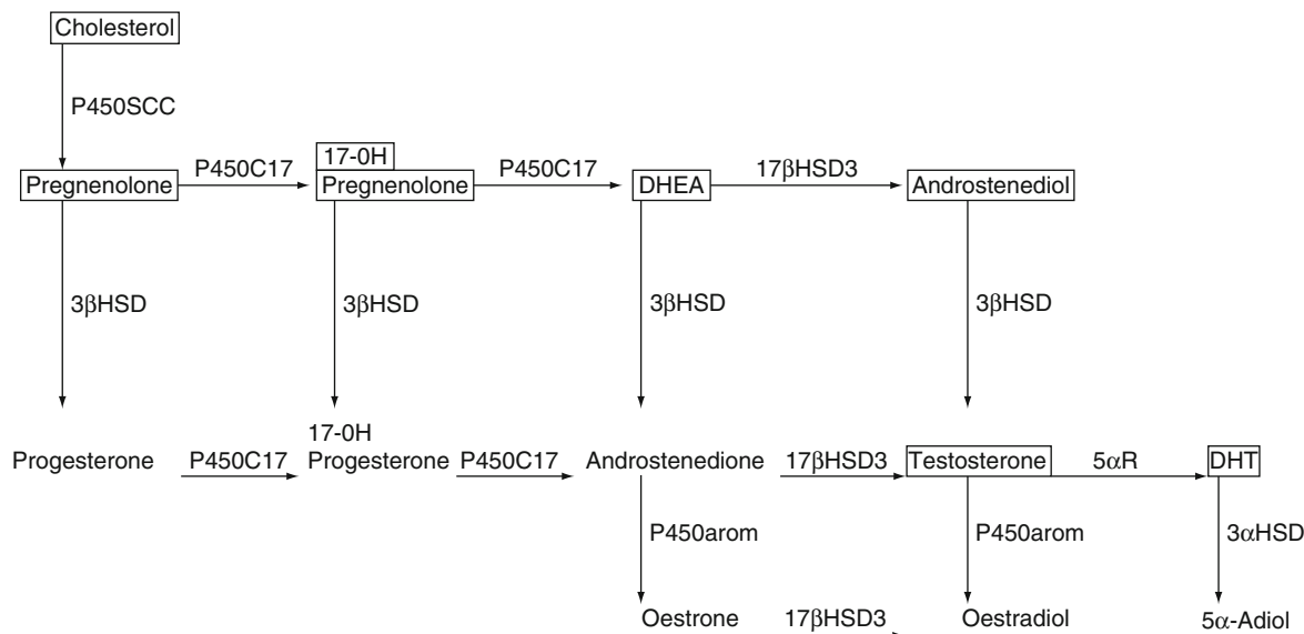
Fig. 3.1 The pathways for steroid hormone synthesis in the adrenal glands and gonads
