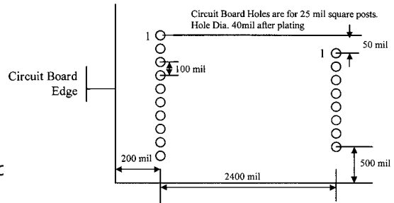
Figure A-6: Personality module connector
