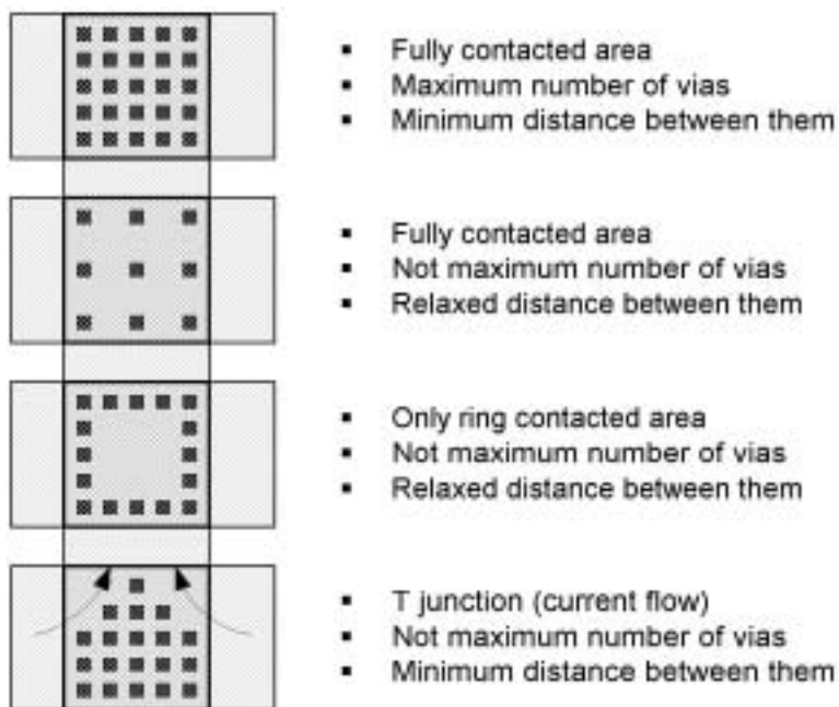
Figure 8.7 Via array configurations for circuit performance.
