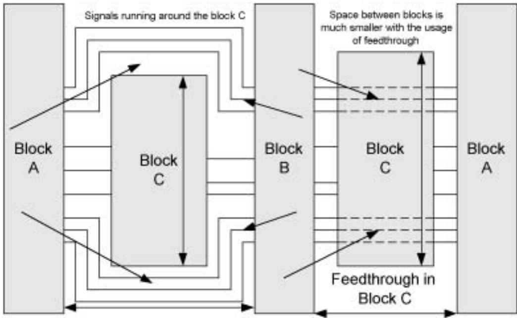
Figure 6.9 Feed-through example.
