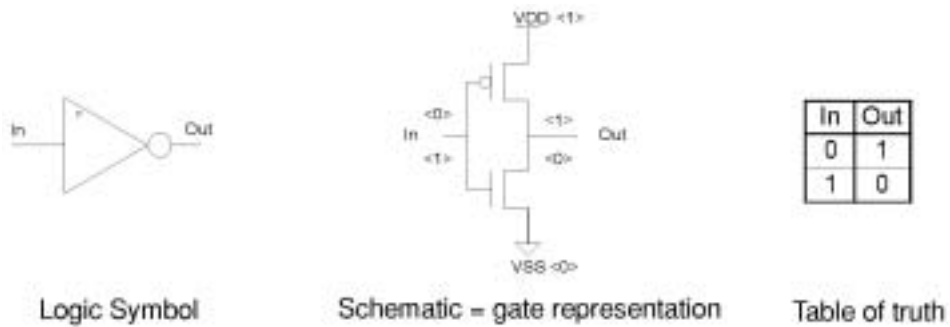
Figure 2.7 Inverter.
