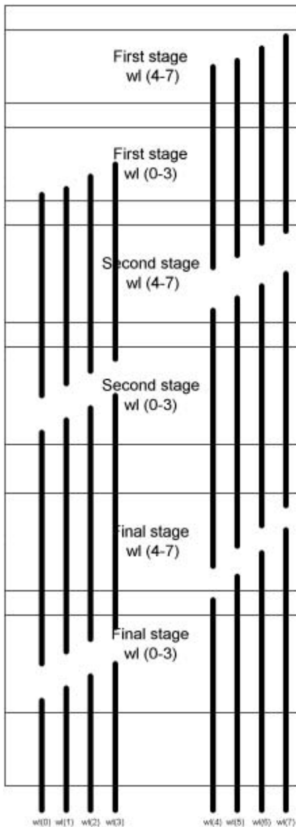
Figure 5.27 Example wordline driver floorplan.
