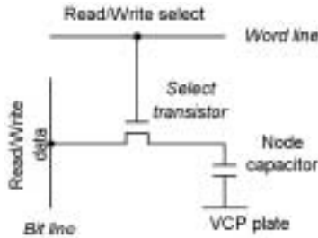
Figure 5.22 DRAM cell schematic.
