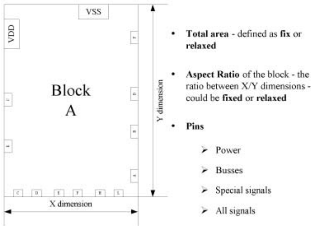
Figure 10.3 Block information needed for floorplan.
