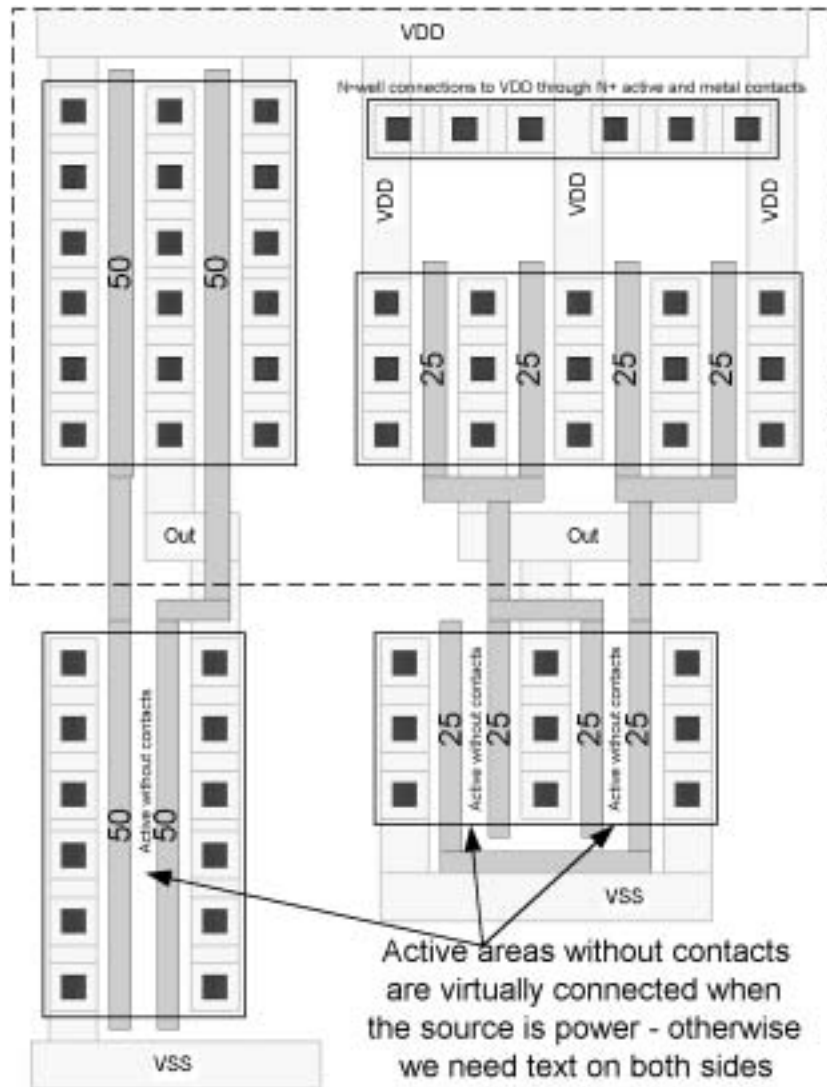
Figure 3.29 Example of fingering a NAND gate.
