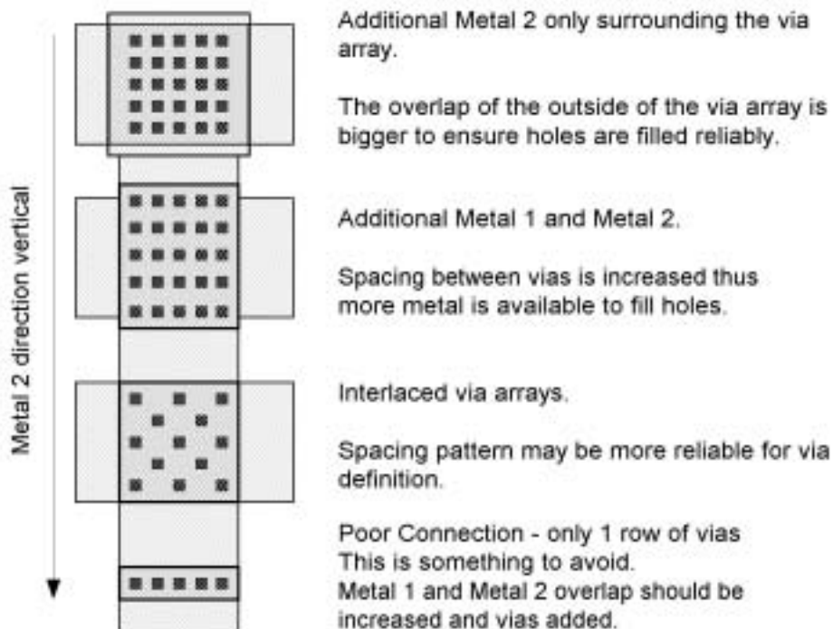
Figure 8.6 Via array configurations for process reliability.
