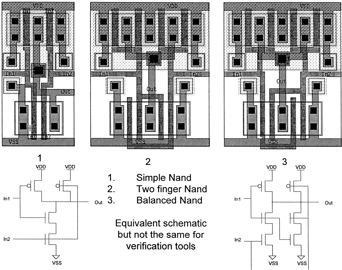
Figure 7.20 Balanced two-input NAND.
