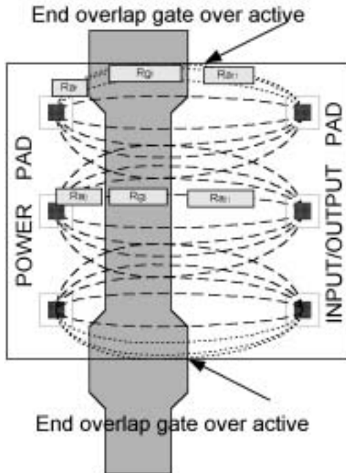
Figure 5.18 Output buffer end overlap rule.
