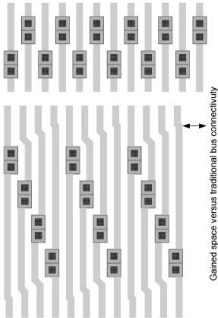
Figure 5.26 Examples of wordline strap layout.
