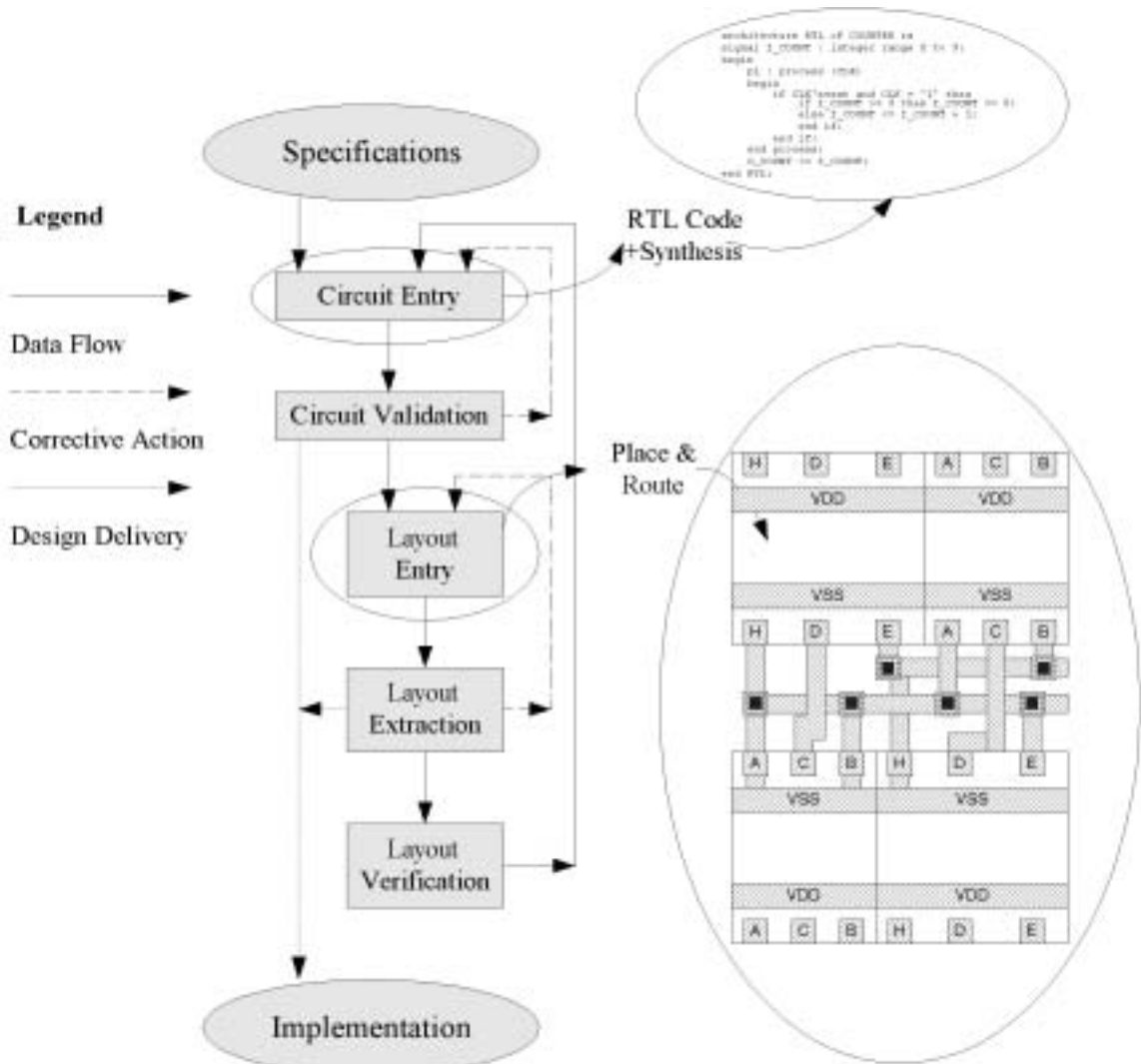
Figure 4.4 ASIC design flow.
