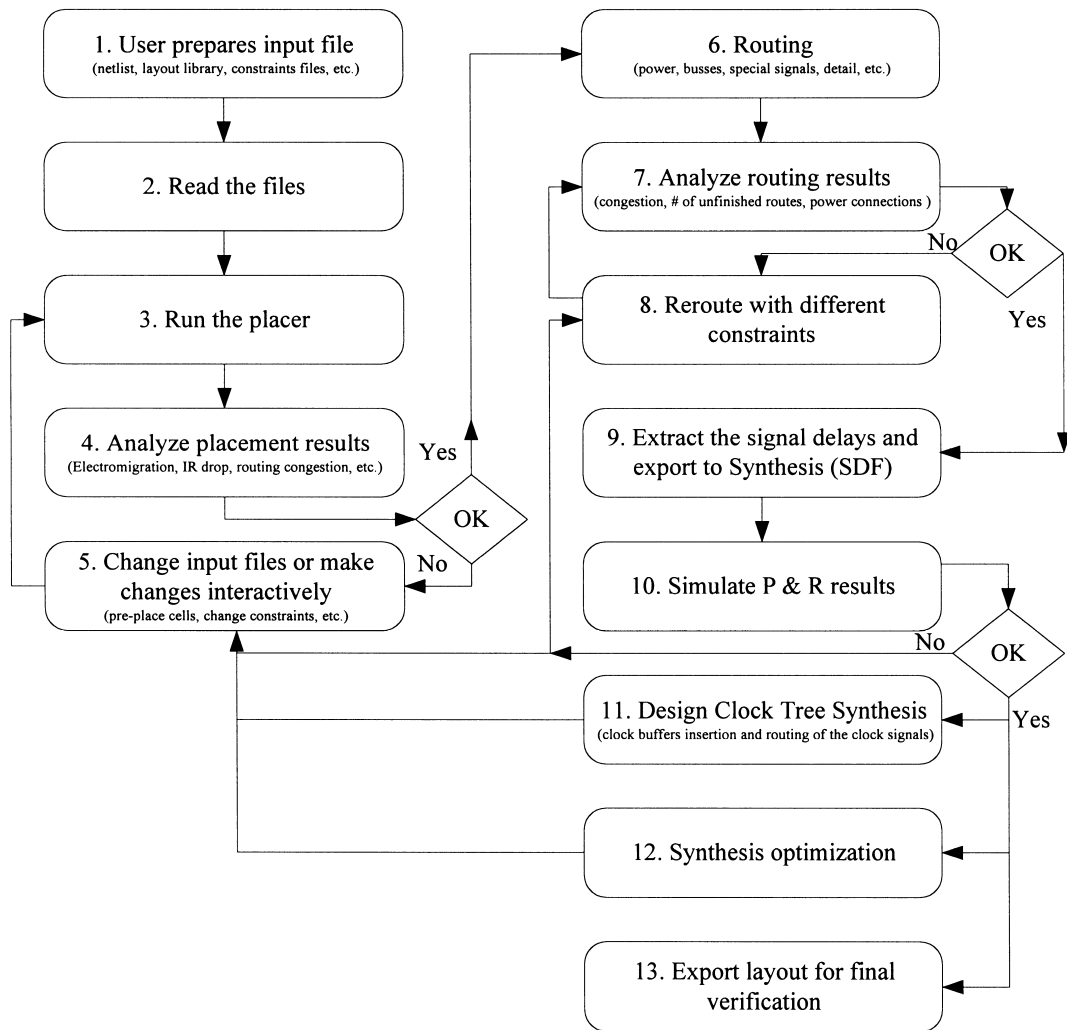
Figure 10.6 Example of ASIC place-and-route flow.
