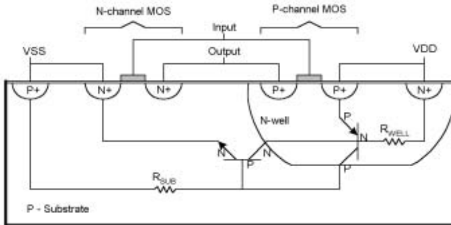
Figure 8.13 Inverter cross-section with latch-up circuit model.
