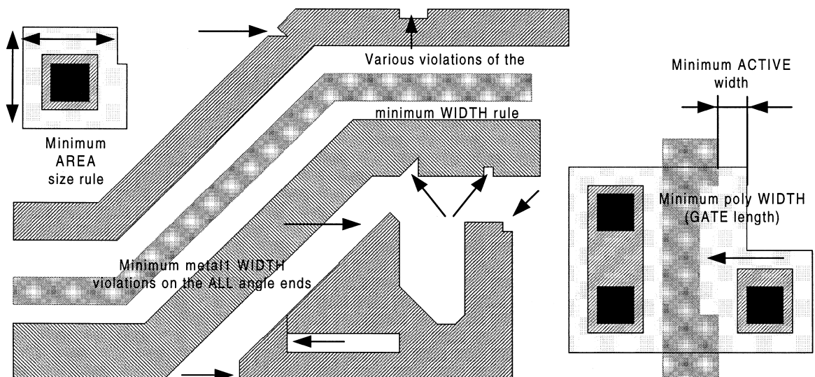
Figure 3.15 Examples of the width rule.
