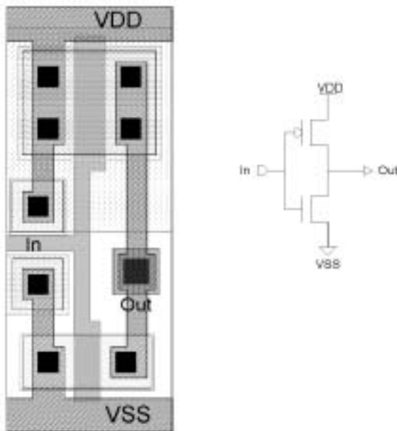
Figure 3.14 Inverter layout and transistor schematic.
