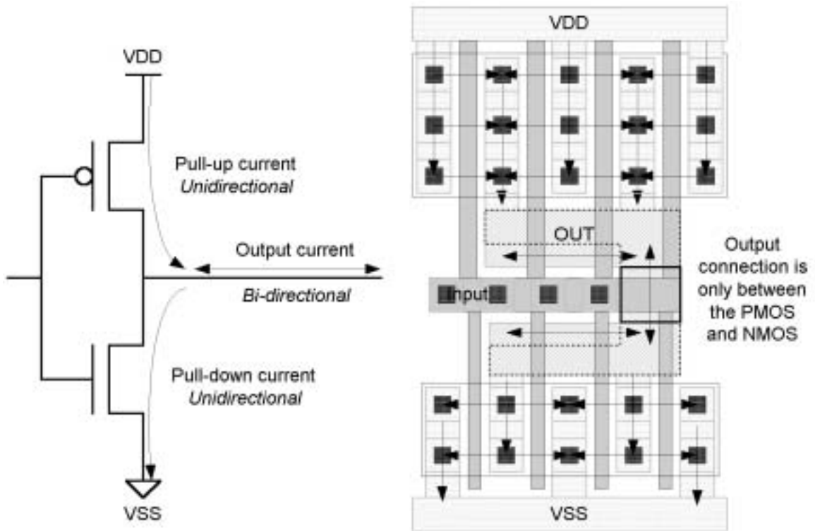
Figure 7.27 Electromigration currents.
