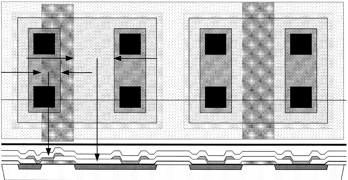
Figure 3.17 Another example of the space rule.
