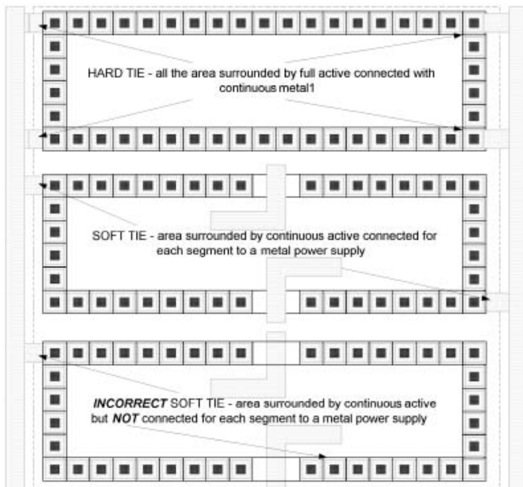
Figure 8.17 Examples of hard and soft ties.
