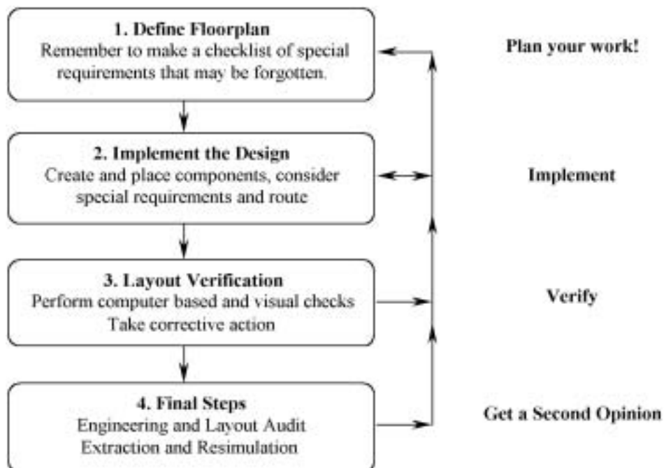
Figure 3.21 Layout design procedure.
