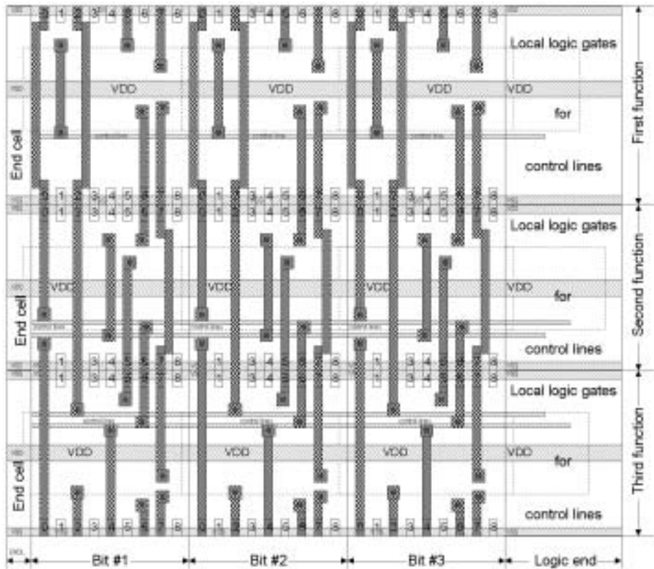
Figure 5.14 Three-bit datapath example.
