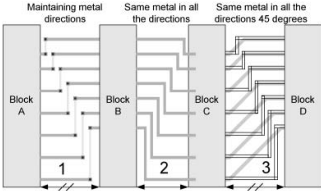
Figure 6.8 Cross-channel routing examples.
