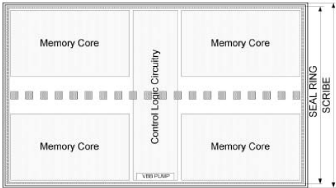
Figure 5.33 Seal ring.
