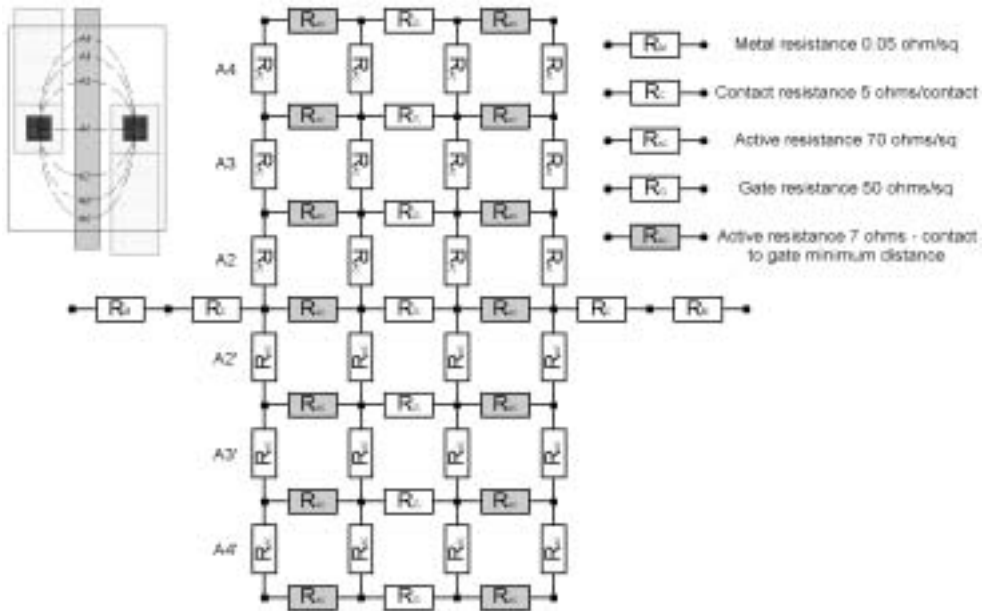
Figure 7.2 Basic transistor resistance model.
