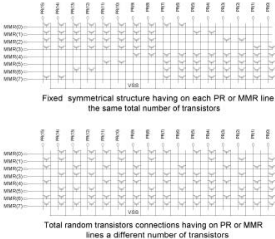
Figure 9.3 Decoder architectures.
