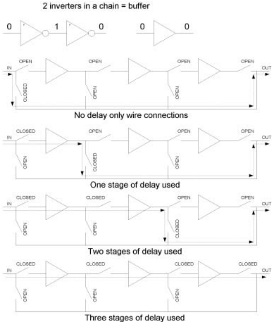
Figure 9.1 Example of a configurable delay chain.
