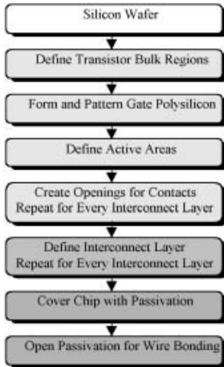
Figure 3.1 CMOS manufacturing process.
