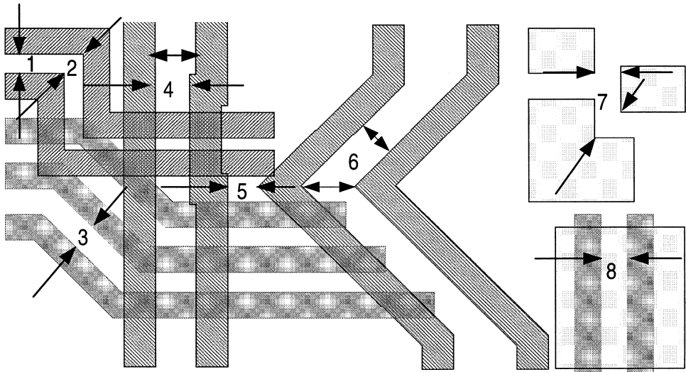
Figure 3.16 Examples of the space rule.
