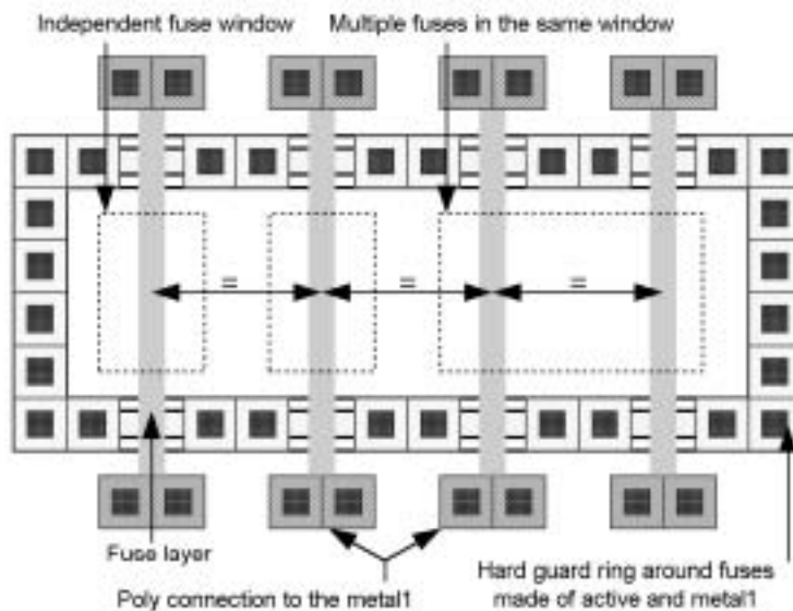
Figure 5.29 Laser fuse layout examples.
