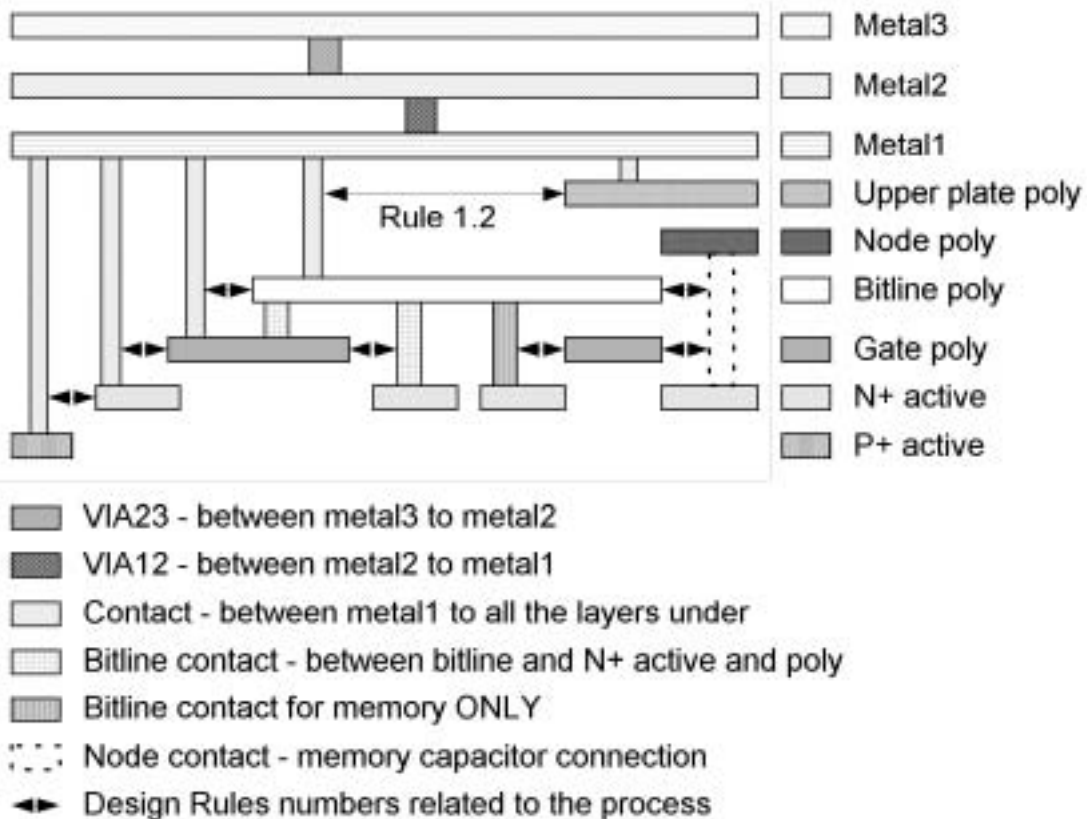
Figure 3.20 Vertical diagram of connectivity for a DRAM process.
