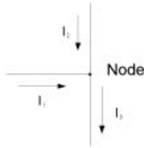
Figure 2.19 Node currents and Kirchhoff's law.
