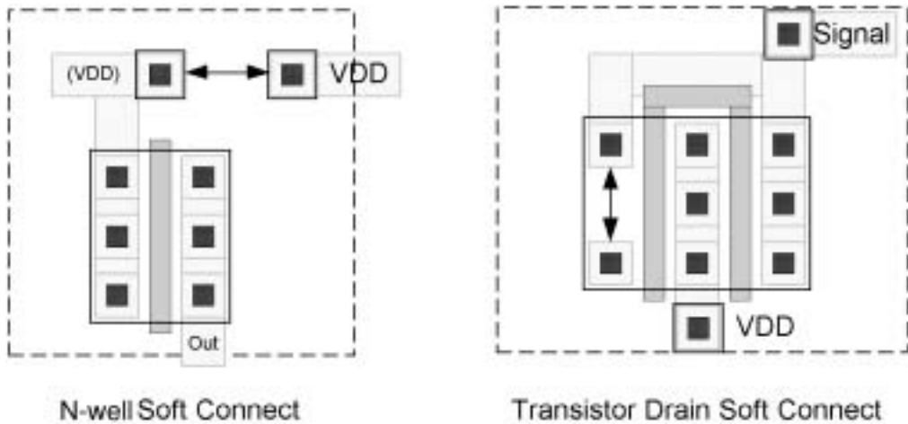
Figure 3.31 Example of soft connections.
