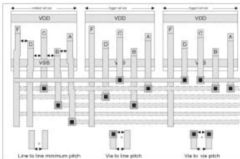
Figure 5.6 Examples of routing grid types.
