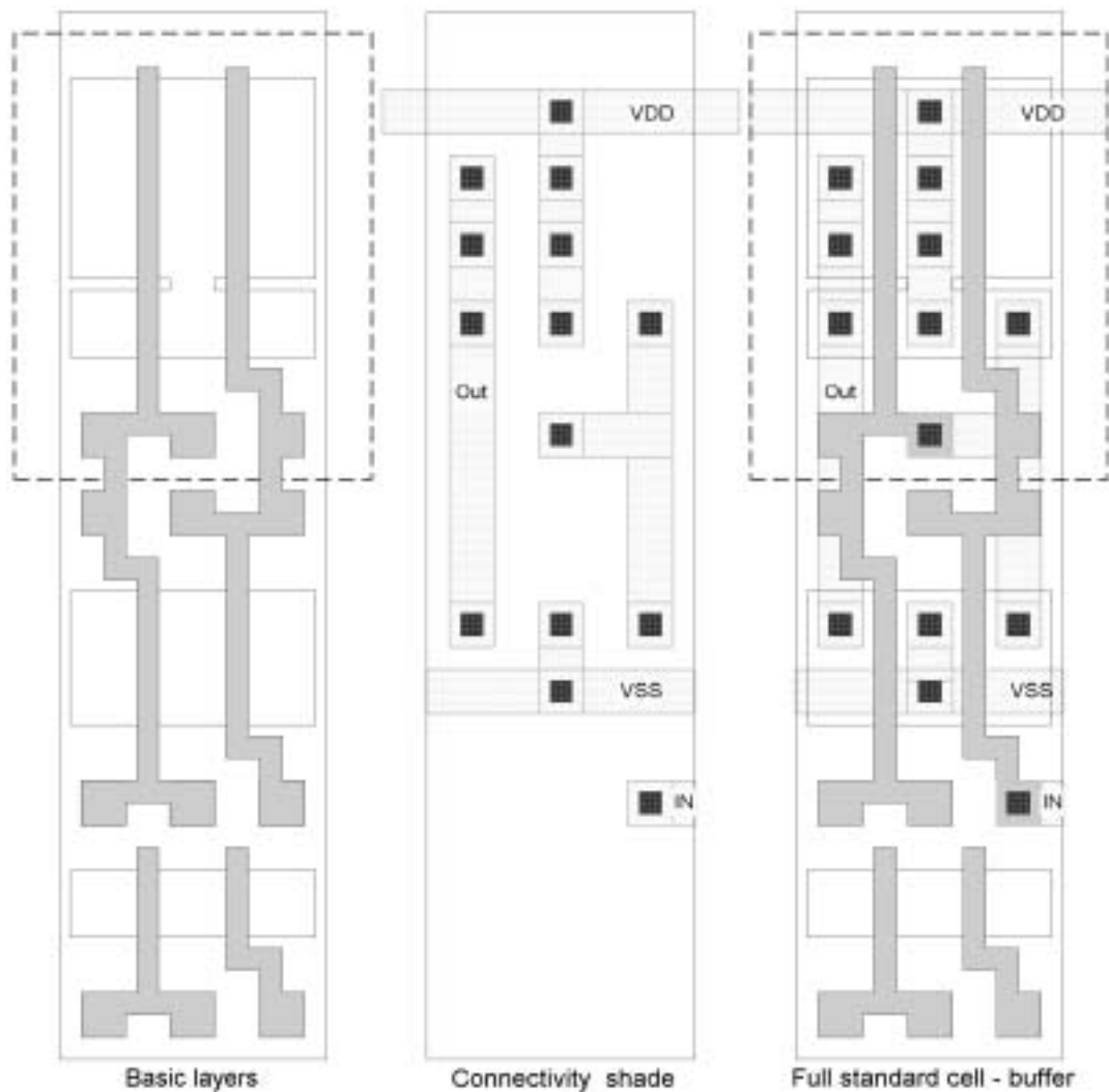
Figure 5.8 Examples of gate array standard cells.
