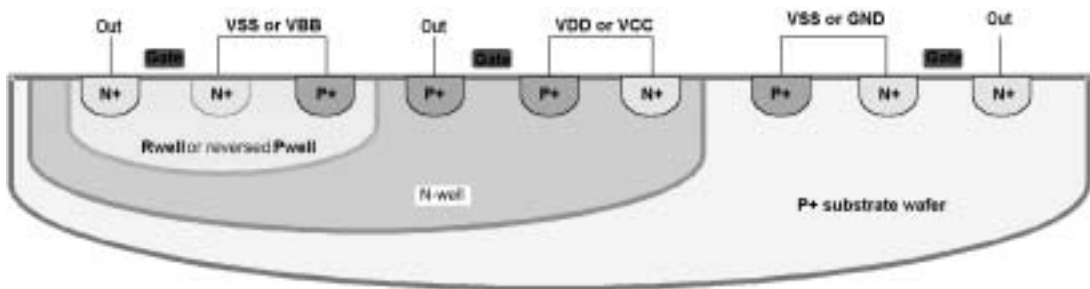
Figure 3.10 Wafer cross-section showing bulk connections.
