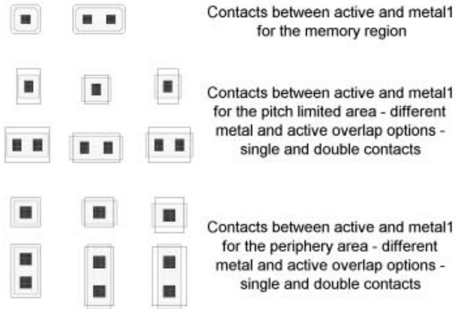
Figure 9.5 Contact examples.
