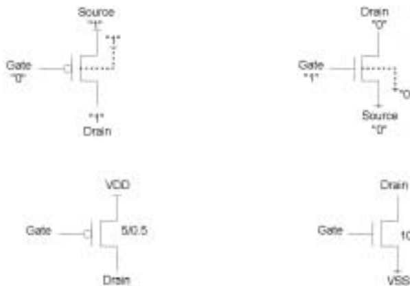
Figure 2.5 MOS transistors showing implied bulk connections.
