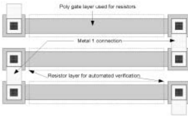
Figure 7.5 Typical resistors.
