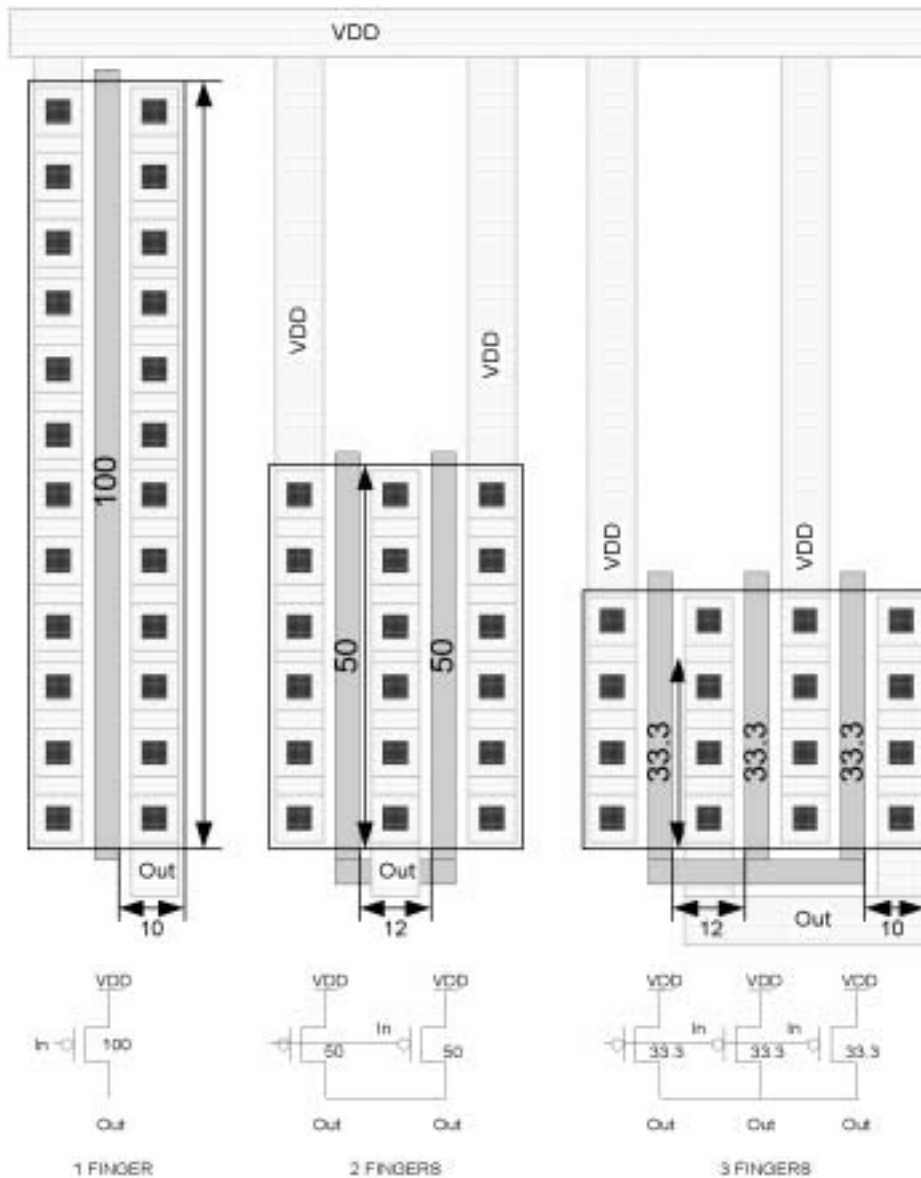
Figure 3.28 Fingering of transistors.
