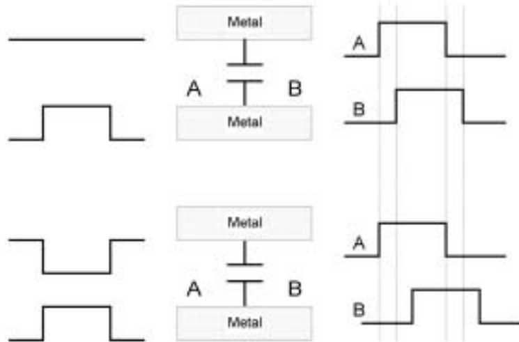
Figure 7.14 Coupling capacitance effect.
