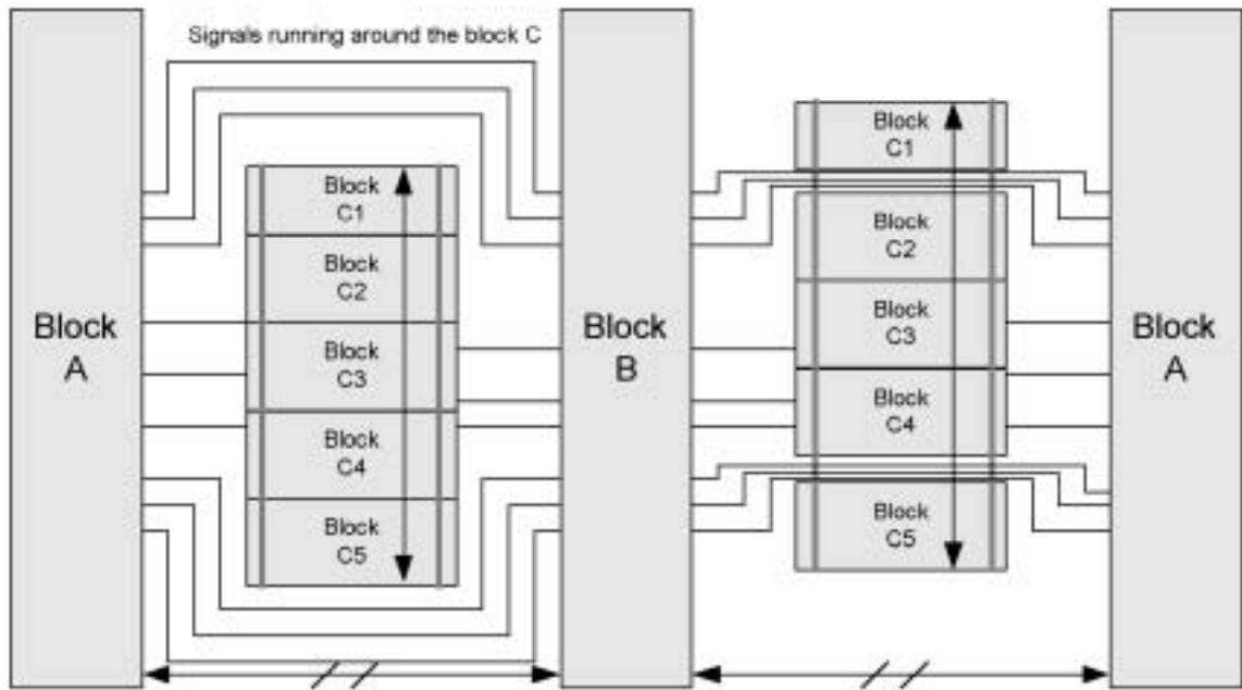
Figure 6.10 Block splitting for feed-throughs.
