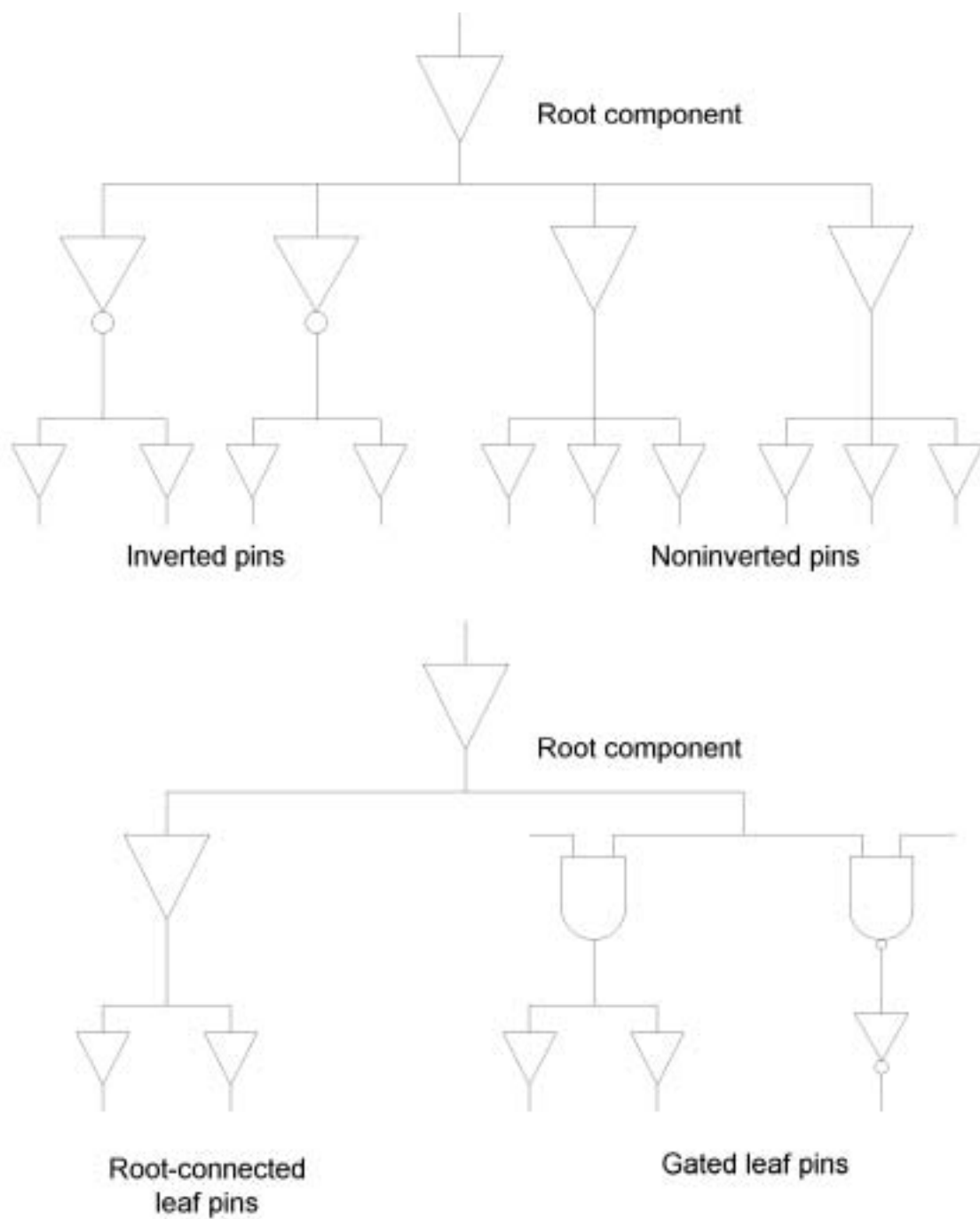
Figure 6.3 Clock tree examples.
