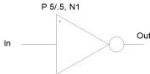
Figure 2.9 Inverter sizing.
