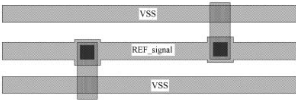
Figure 7.16 Simple shielding example.
