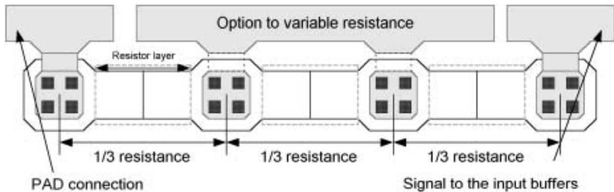
Figure 5.20 Input ESD protection resistor.
