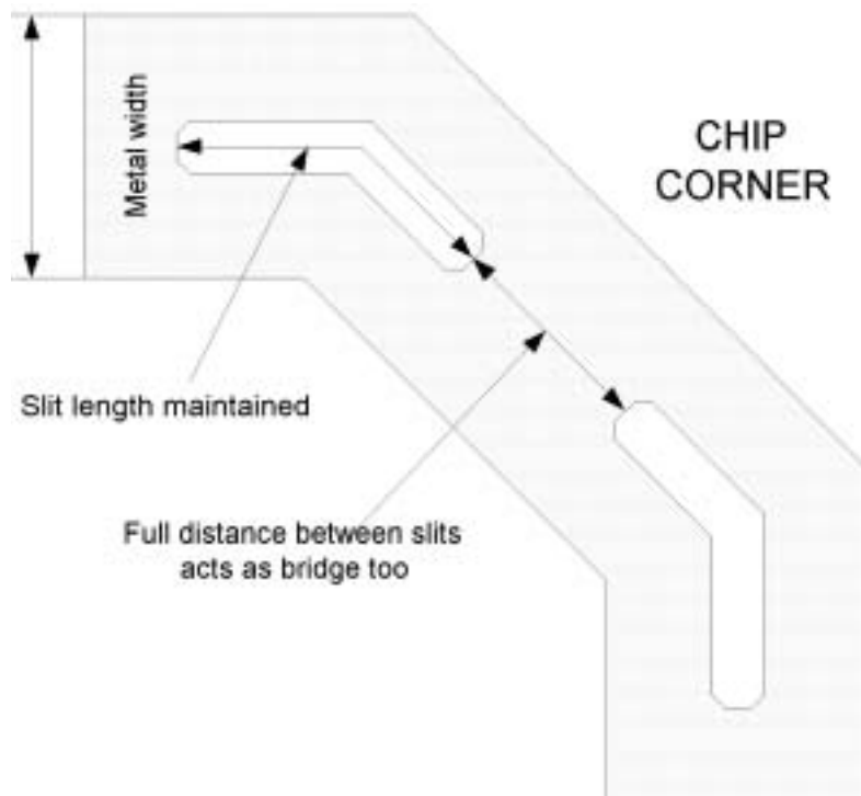
Figure 8.3 Corner routing power.
