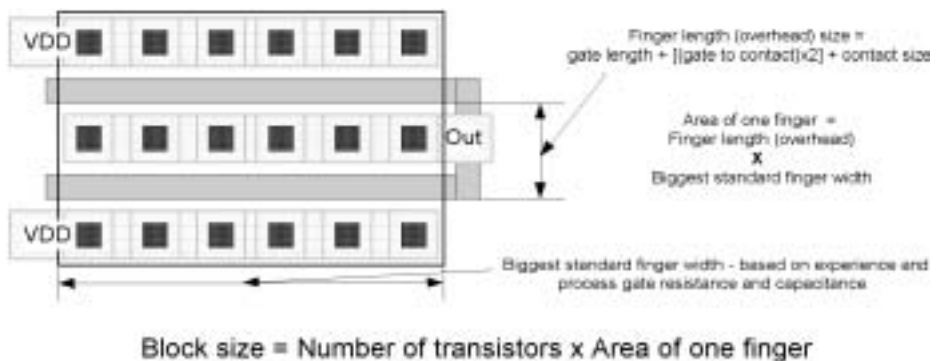
Figure 9.8 Basic calculation scheme for floorplanning.
