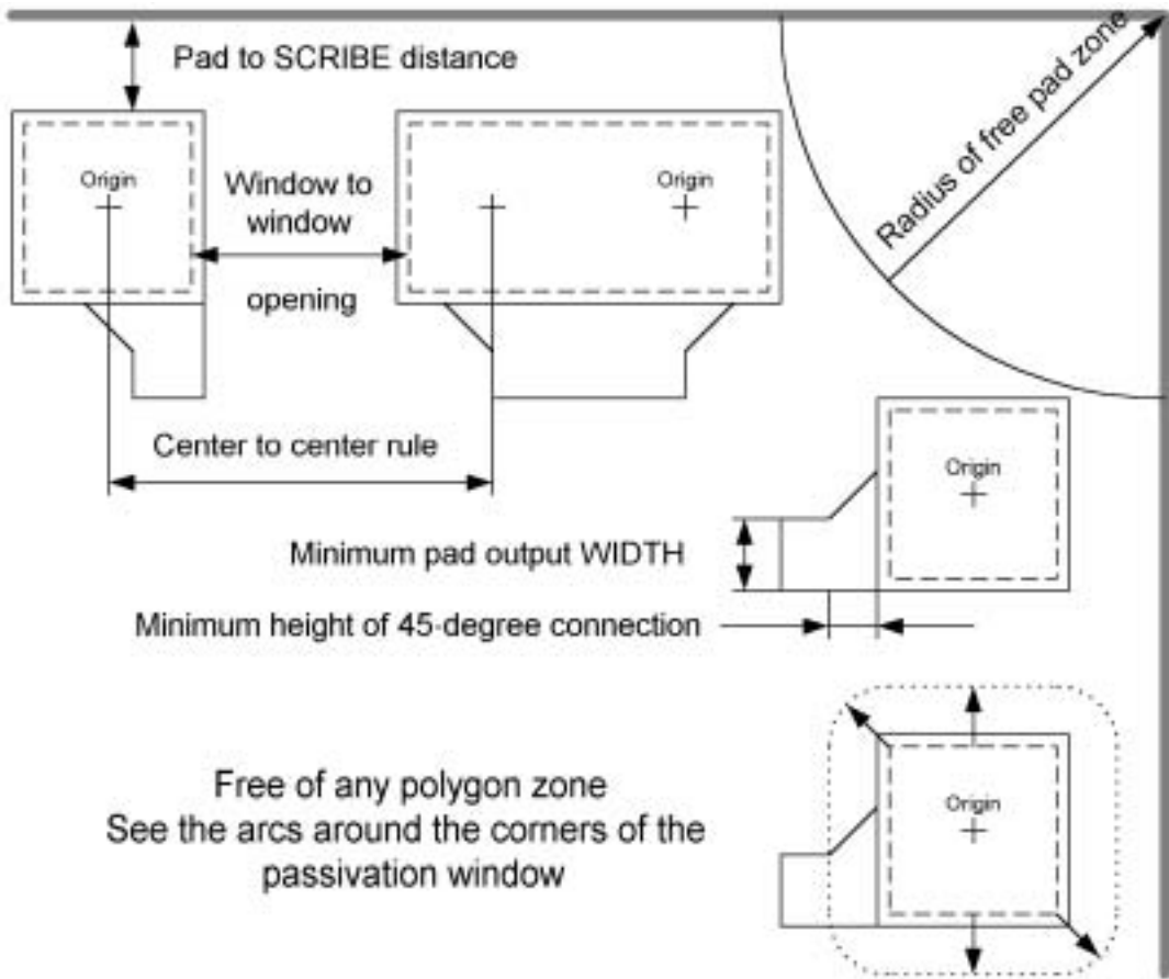
Figure 5.17 Examples of pad cell design rules.
