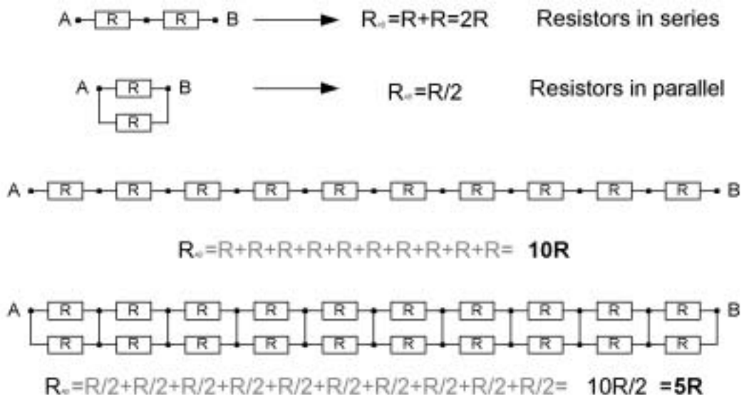
Figure 7.1 Examples of equivalent resistance.
