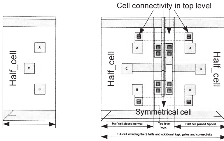
Figure 7.19 Symmetrical layout example.
