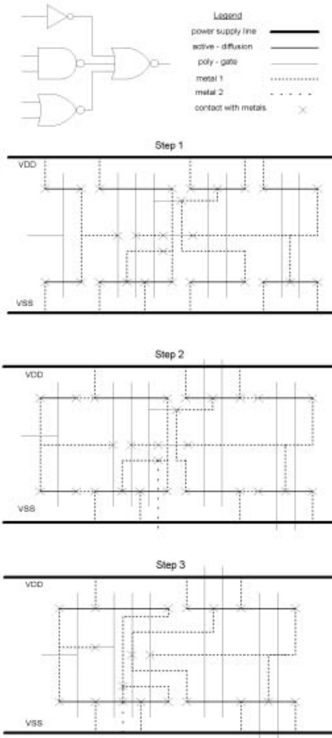
Figure 3.23 Example stick diagram layout.
