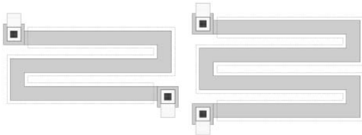
Figure 7.6 Efficient resistor styles.
