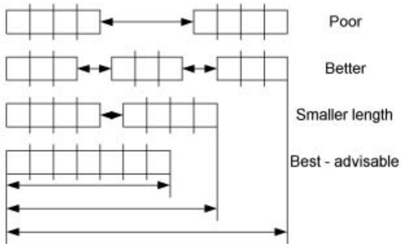
Figure 5.28 Fuse row and rules.
