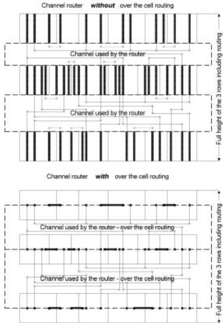
Figure 5.5 Comparison of routing styles.
