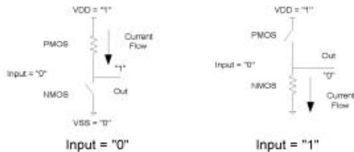
Figure 2.8 Inverter operation.
