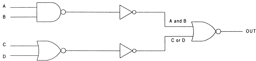
Figure 2.13 Complex logic.
