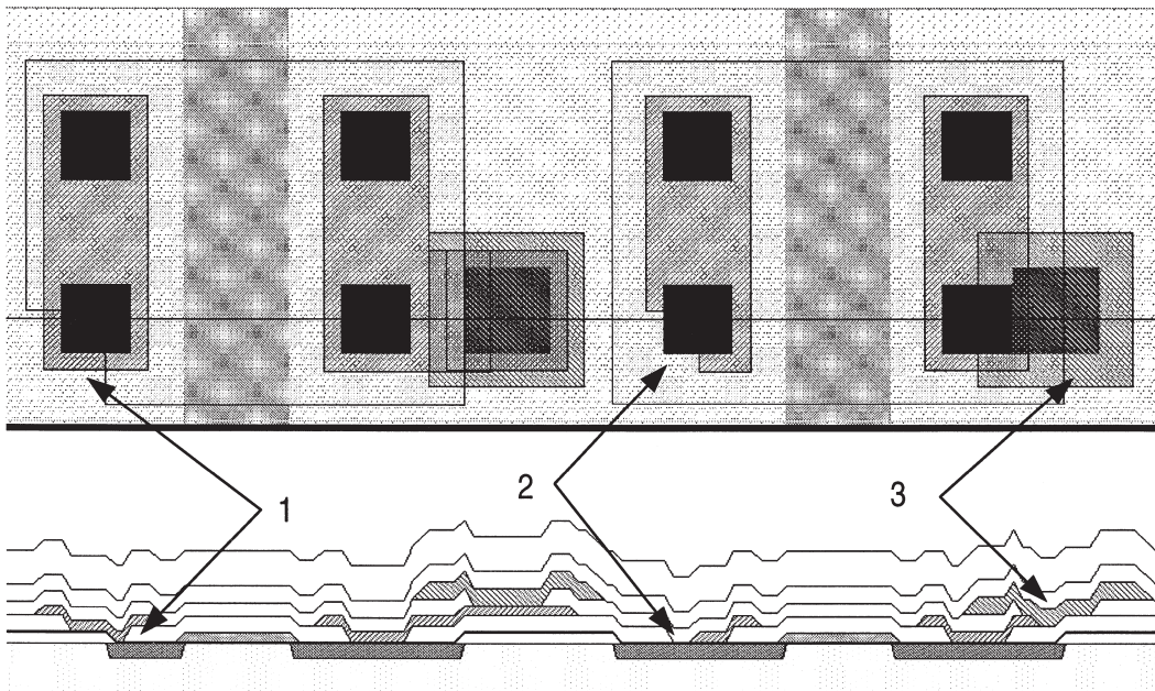
Figure 3.18 Example of the overlap rule.
