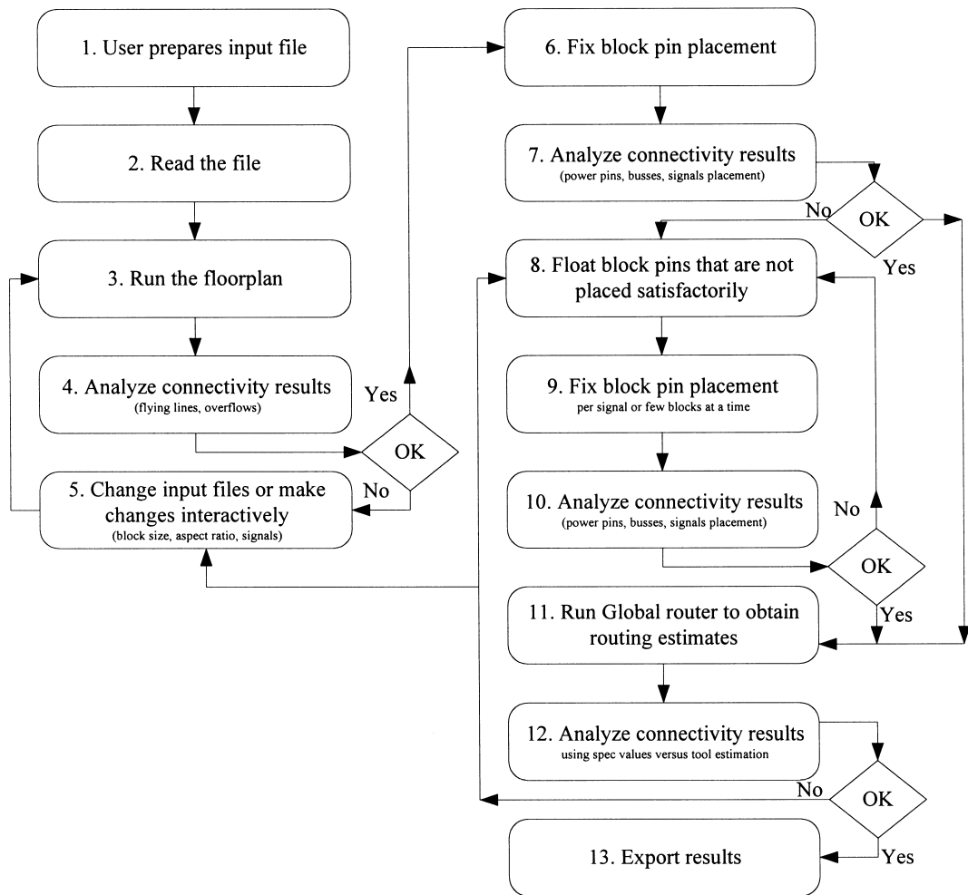
Figure 10.4 Floorplanning procedure.
