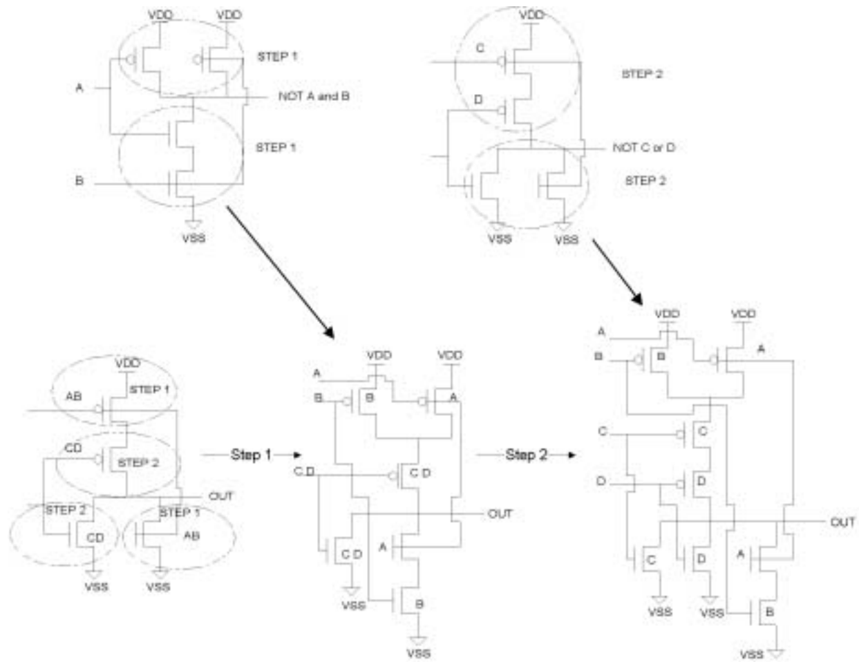
Figure 2.15 Complex gate solution.
