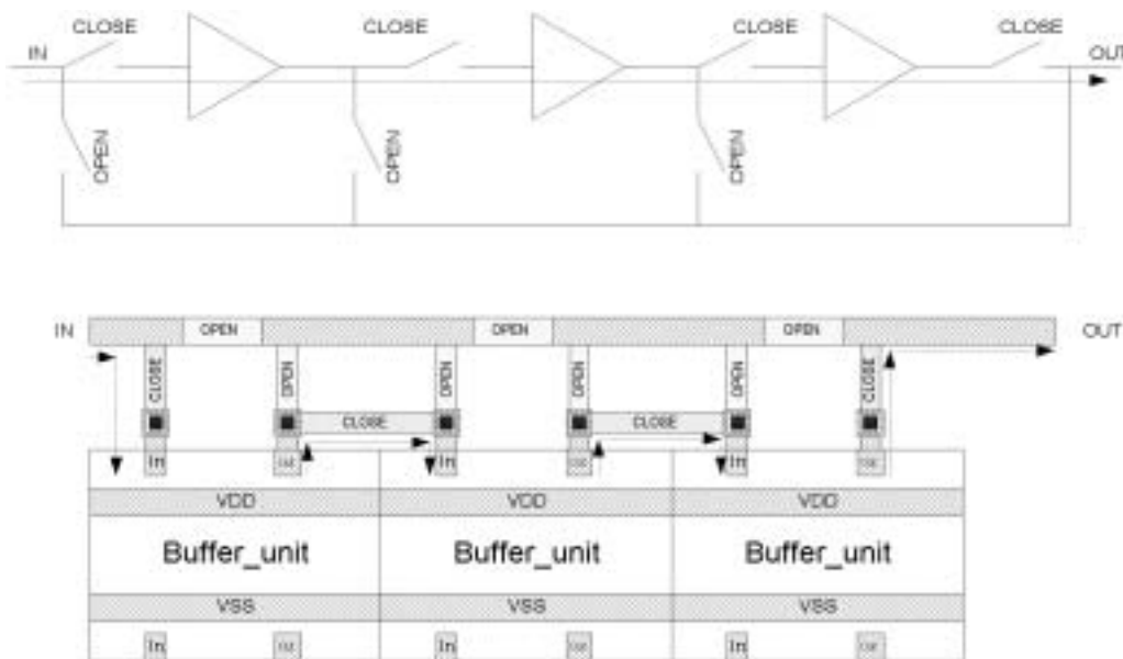
Figure 9.2 Delay chain layout.
