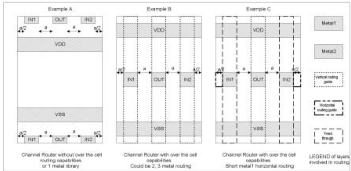
Figure 5.4 Comparison of cell interfaces.
