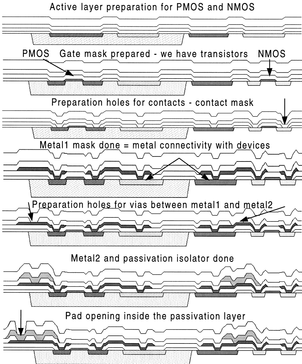
Figure 3.2 Example of cross-section process steps.
