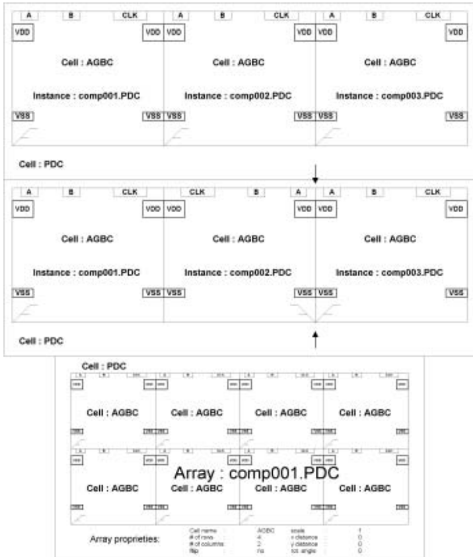
Figure 3.24 Examples of hierarchical designs.
