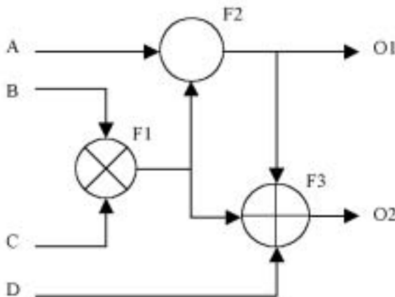
Figure 5.12 Single-bit data flow schematic.
