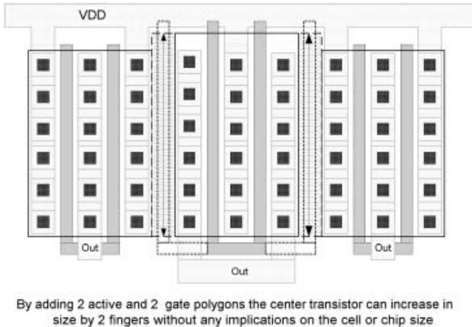
Figure 9.6 Drivers size adjustments.
