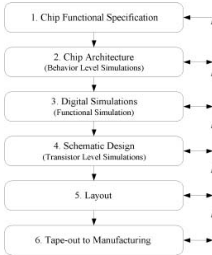
Figure 4.1 Full-custom flow for a microprocessor.
