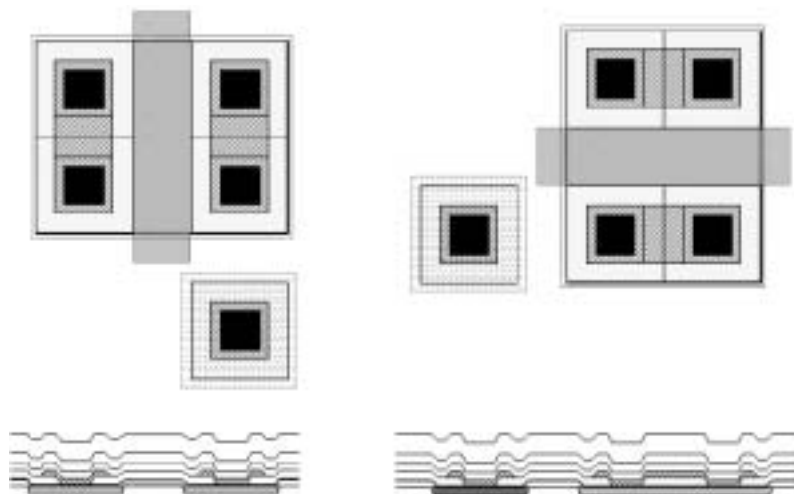
Figure 3.9 Simple NMOS transistor layout.
