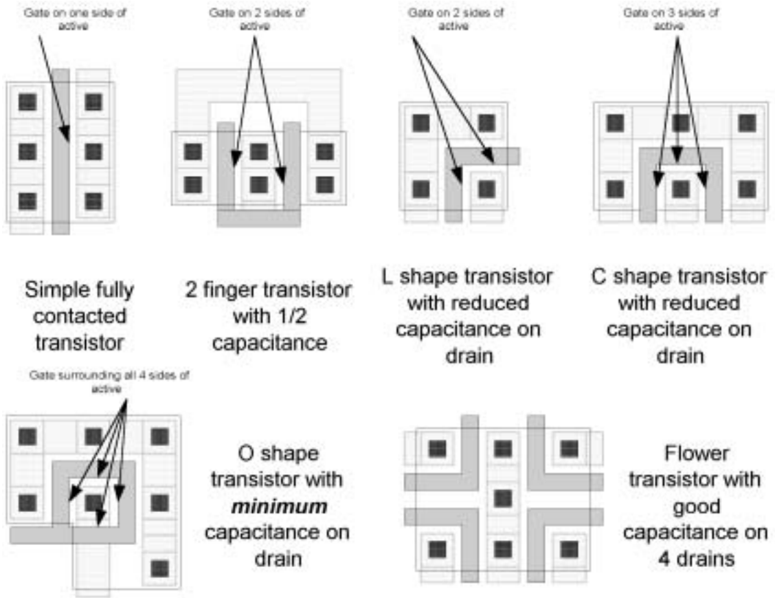
Figure 7.12 Minimum capacitance transistors.
