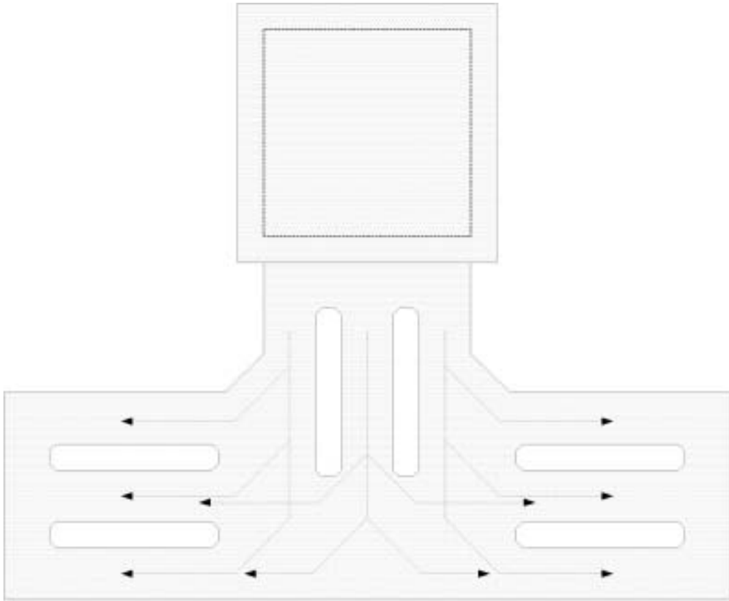
Figure 8.4 Pad connection with slits.
