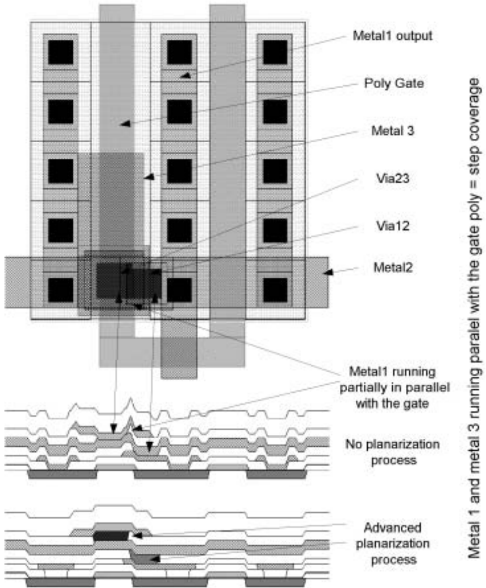
Figure 8.8 Step coverage problem.
