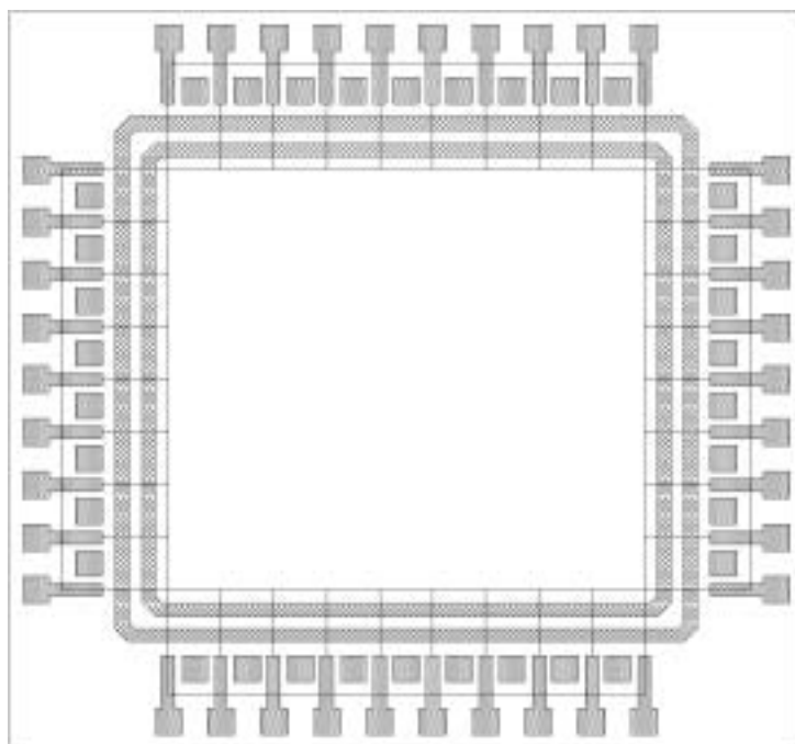
Figure 5.16 Pad frame example.
