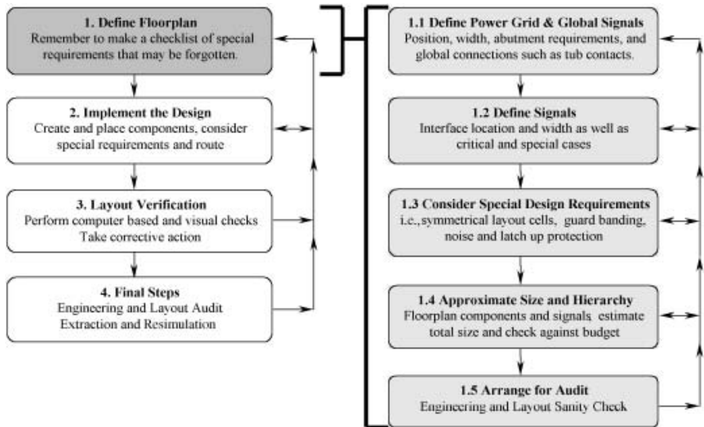
Figure 3.22 Layout planning procedure.
