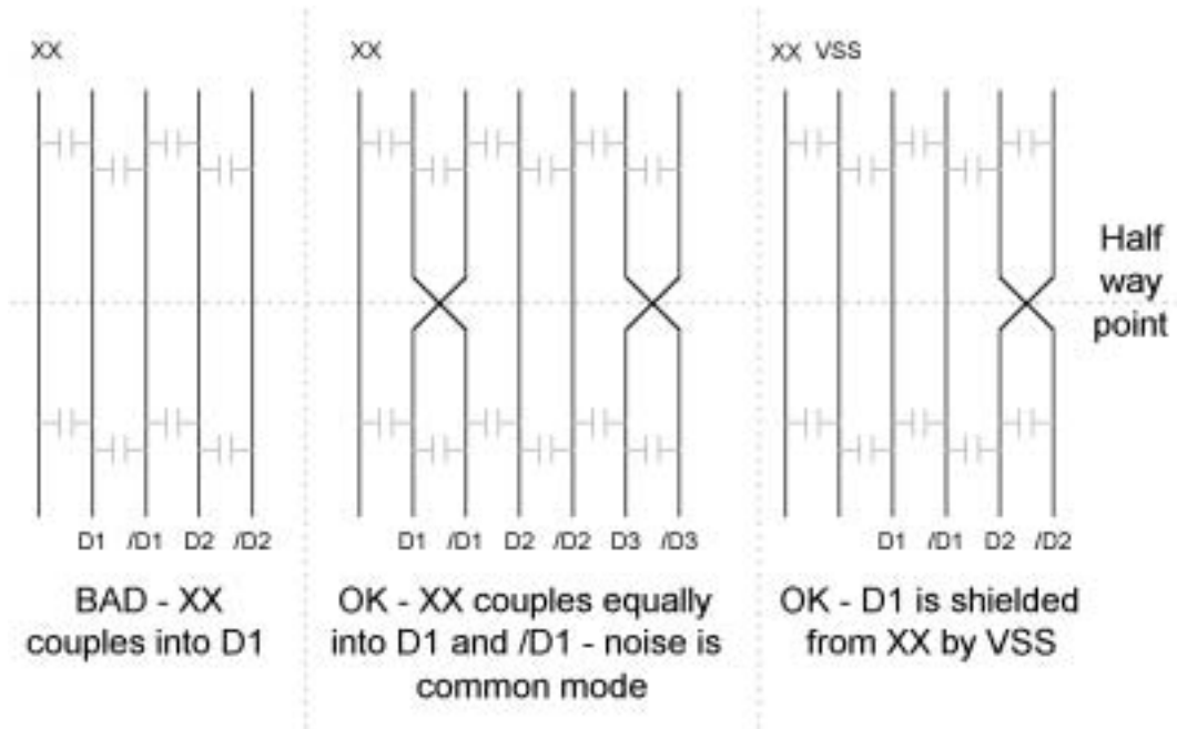
Figure 7.15 Differential pair twisting to reduce signal coupling.
