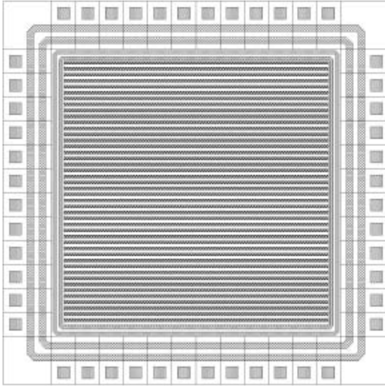
Figure 5.9 Example gate array master slice.
