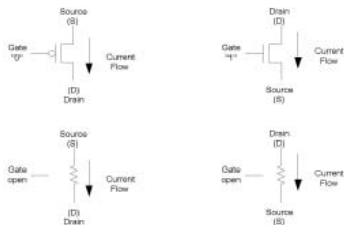
Figure 2.18 PMOS model (left) and NMOS model (right).
