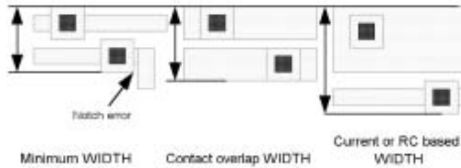
Figure 3.25 Routing line width considerations.
