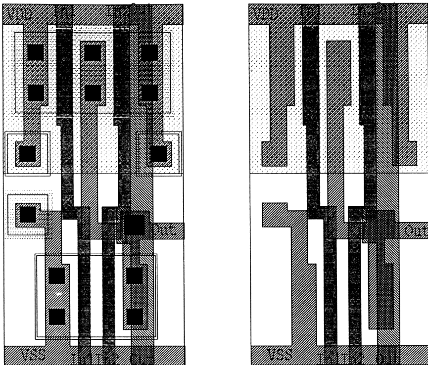
Figure 5.2 Example standard cell showing all layers.
