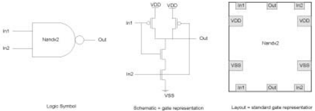
Figure 5.1 NAND example of standard cell.
