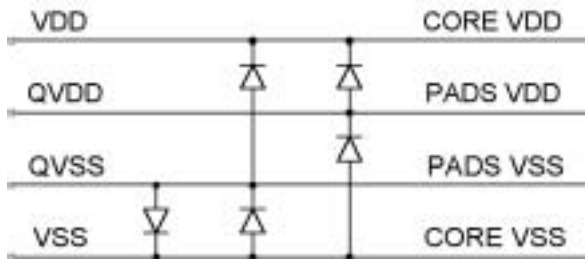
Figure 7.28 Power supply clamping diodes.
