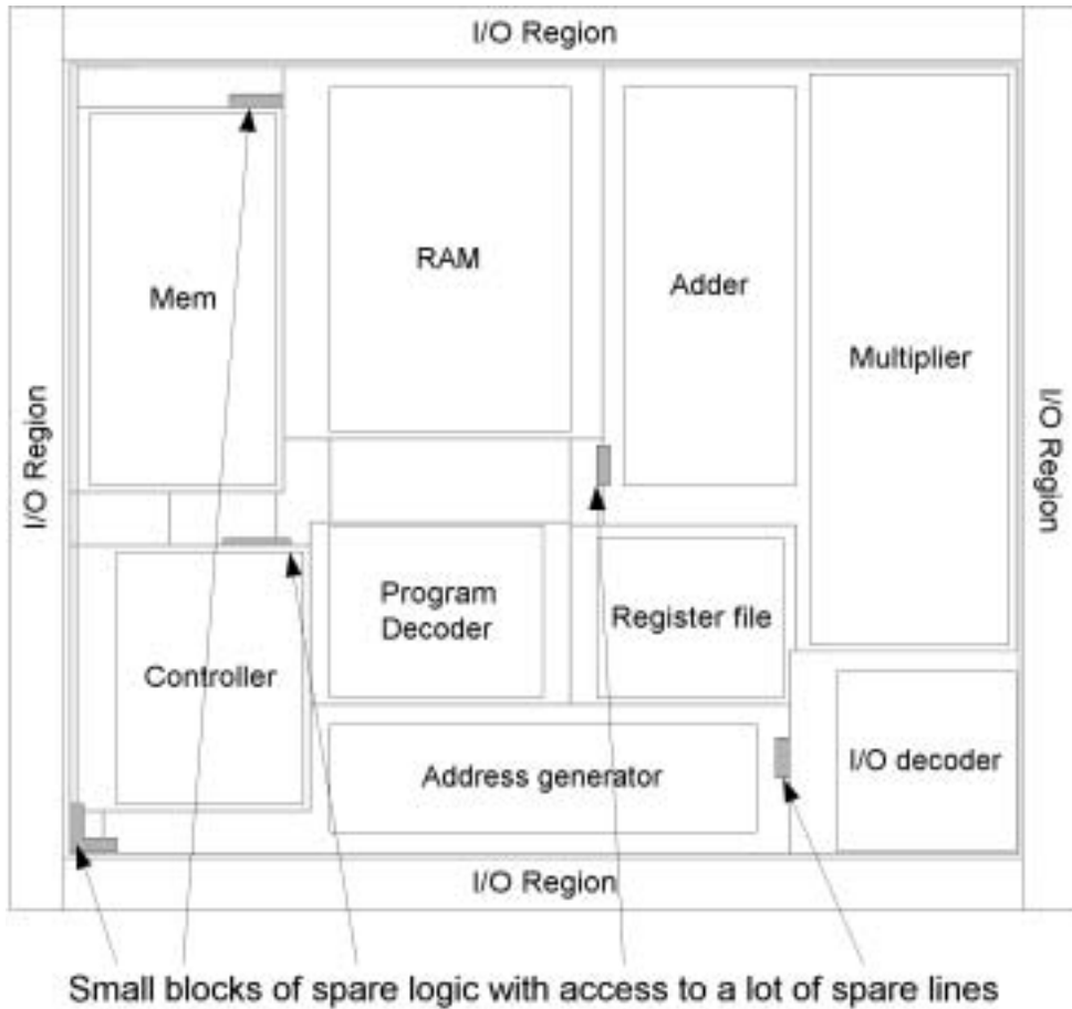
Figure 9.7 Spare logic and spare lines.
