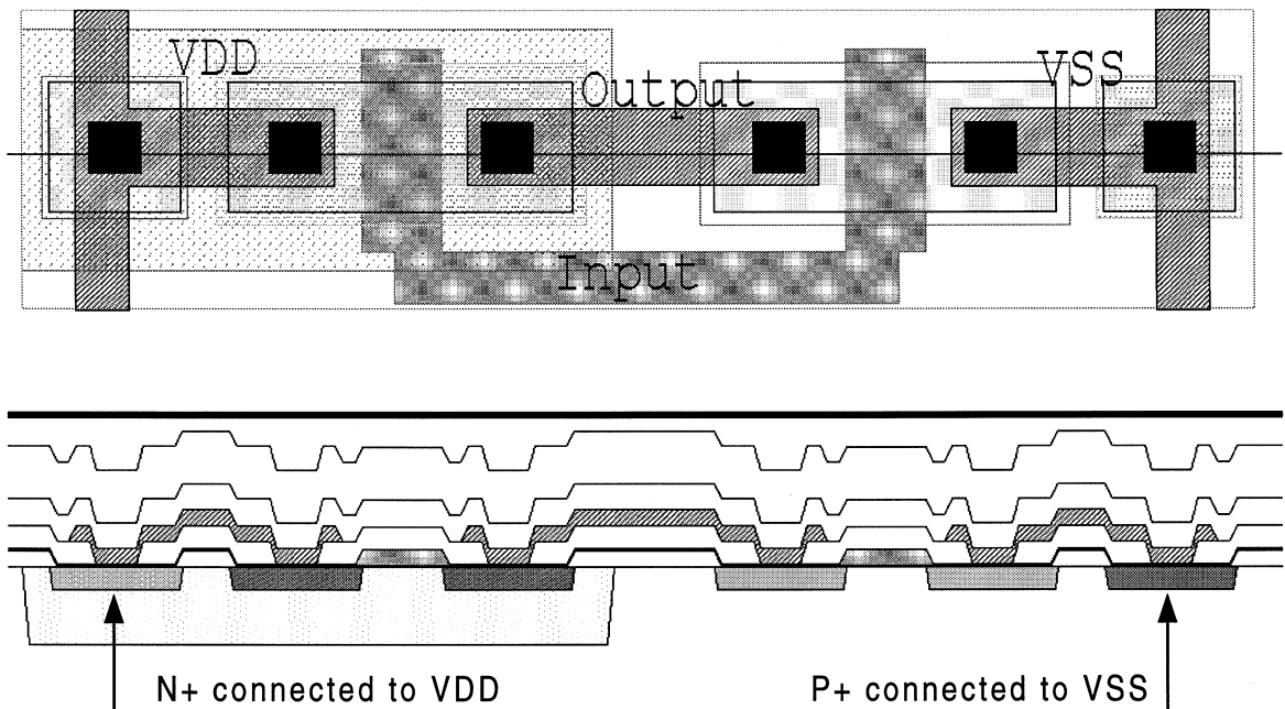
Figure 3.11 Cross-section inverter bulk connections.
