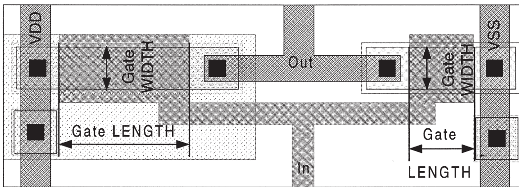
Figure 3.8 Weak feedback inverter.
