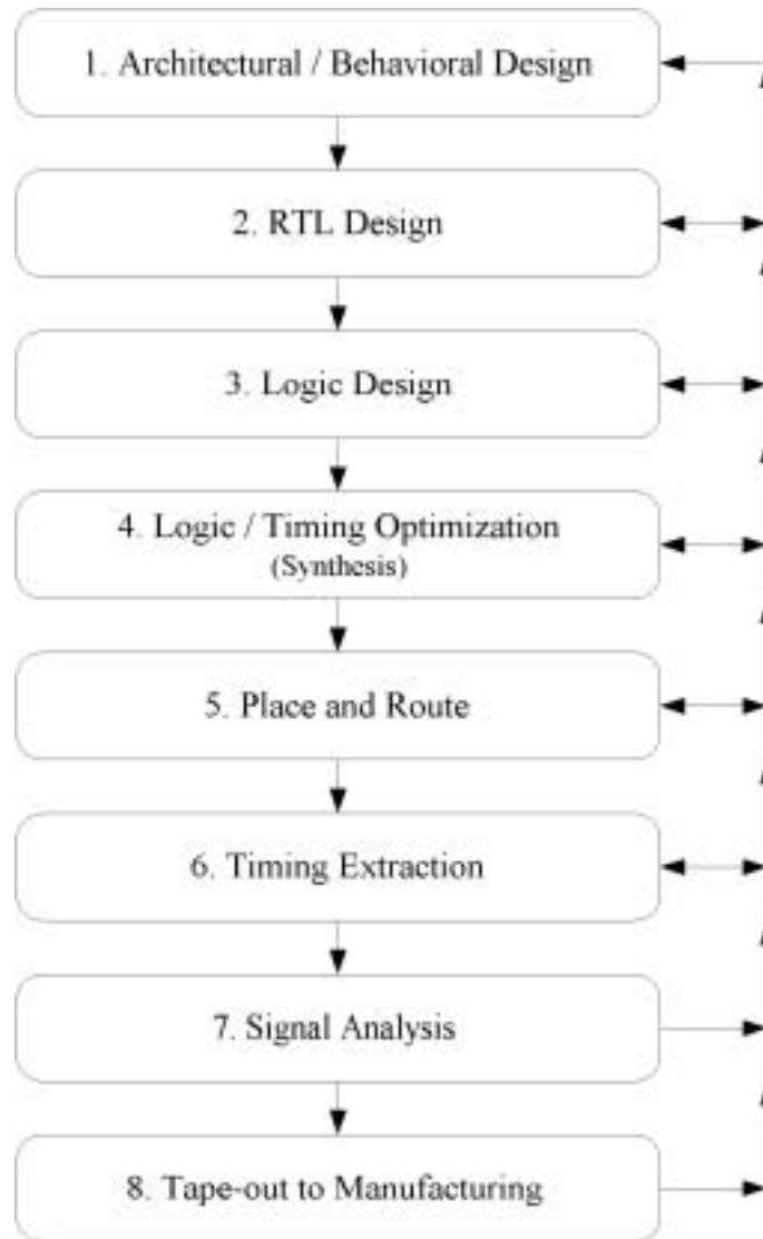
Figure 4.2 Detailed ASIC flow.
