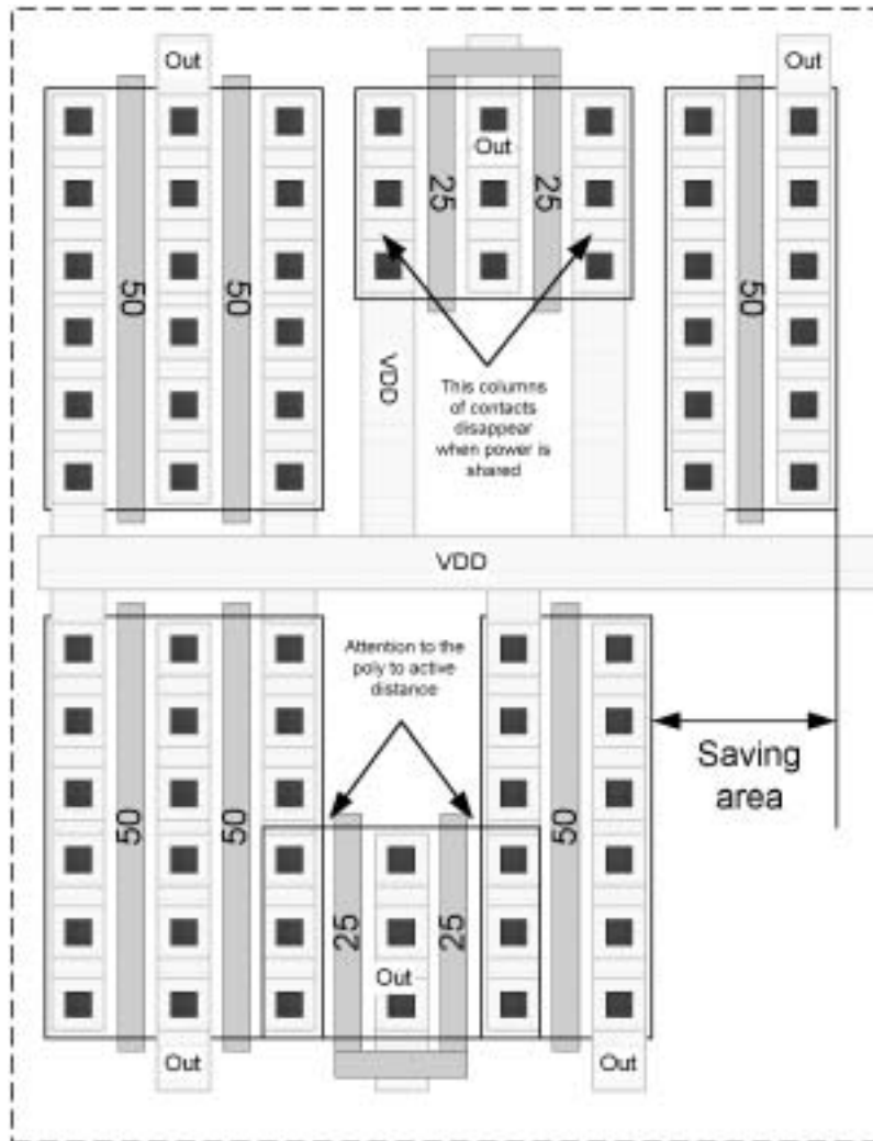
Figure 3.30 Transistor power sharing example.
