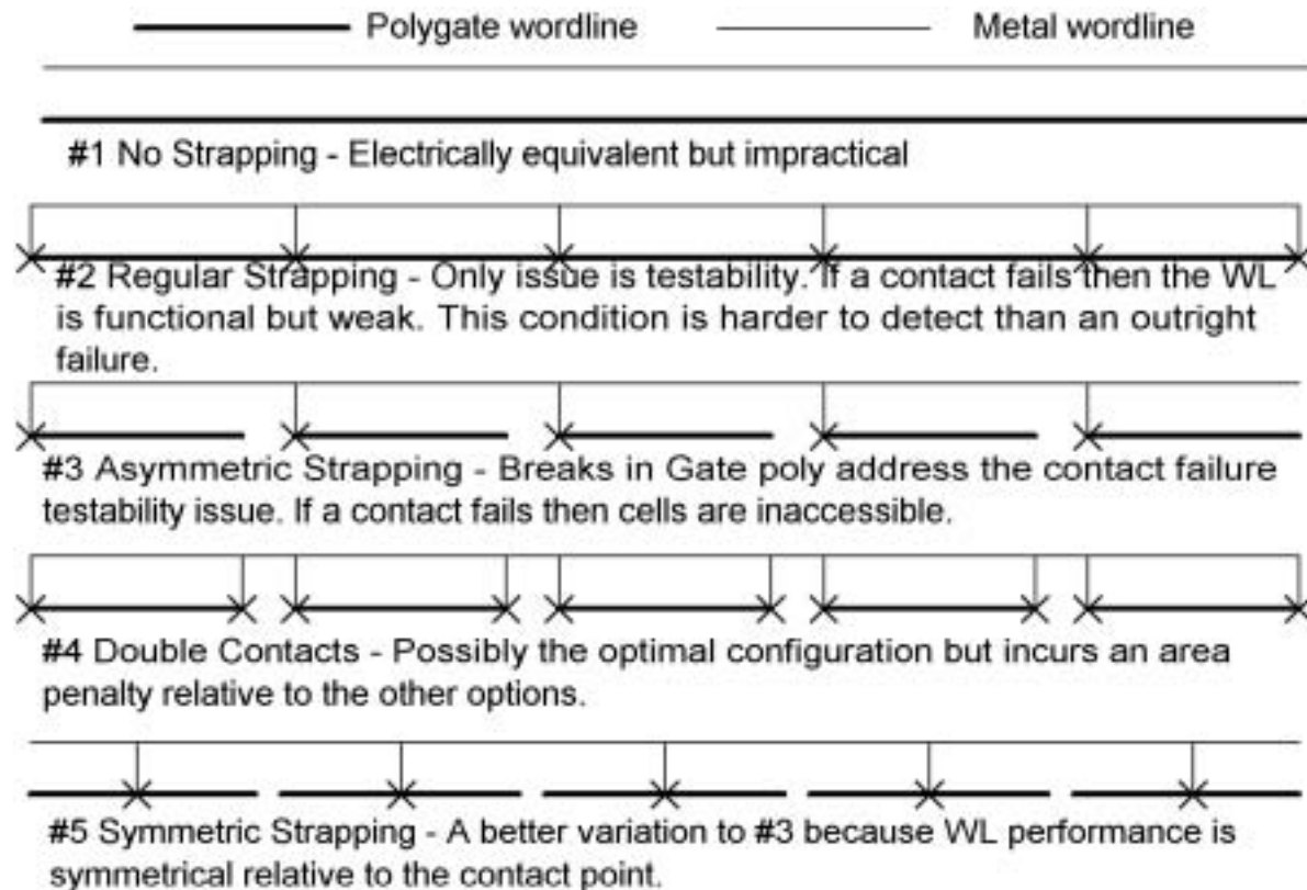
Figure 5.25 Wordline strapping schemes.
