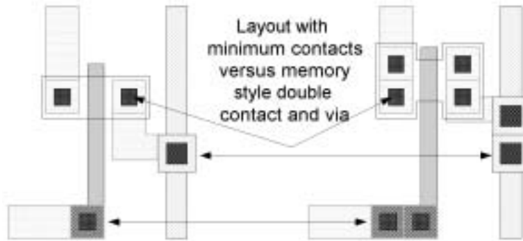
Figure 8.12 Single and double contact design styles.
