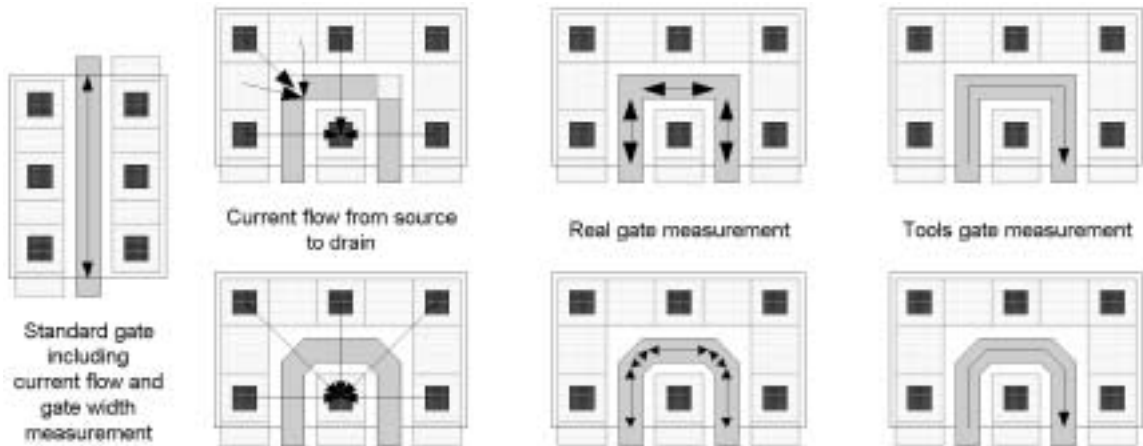
Figure 7.25 Simple examples of bent gates.
