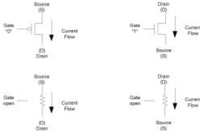
Figure 3.6 PMOS and NMOS transistors.
