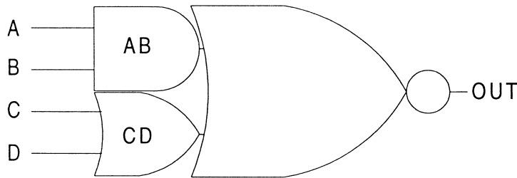
Figure 2.14 Complex gate example.
