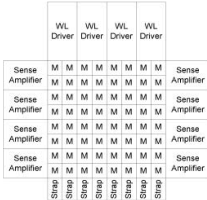
Figure 5.24 Memory array pitch-limited cells.
