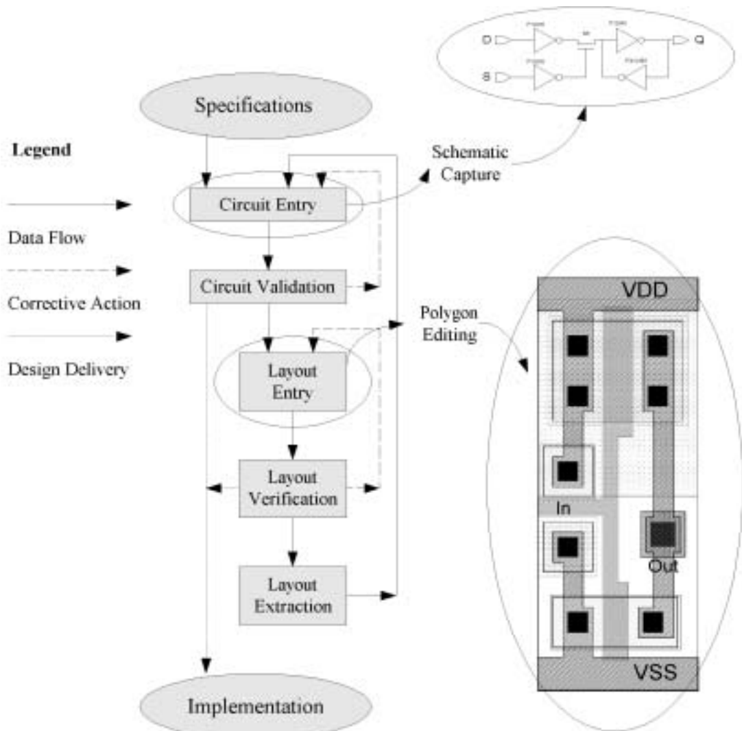
Figure 4.3 Full-custom (or analog) design flow.
