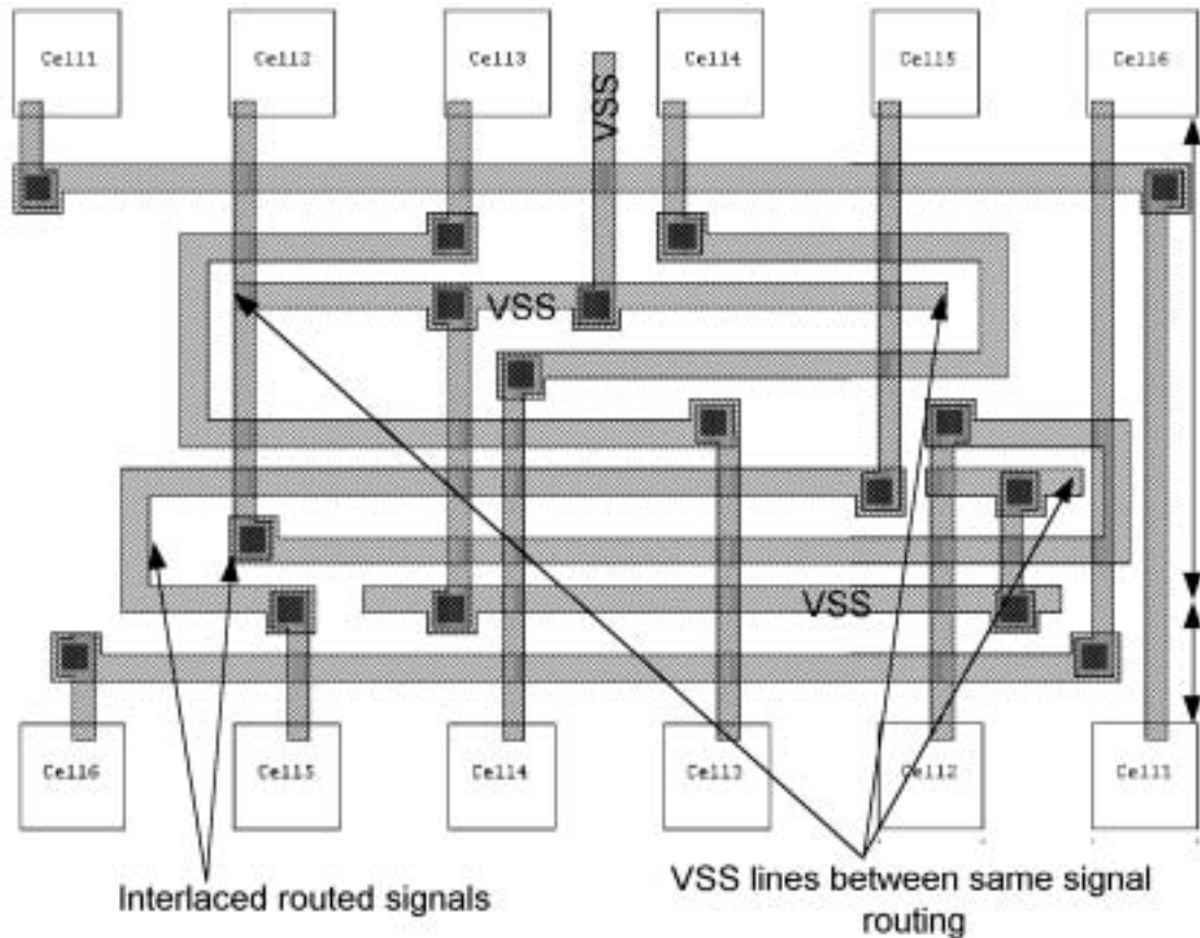
Figure 7.23 Physical compensation example.
