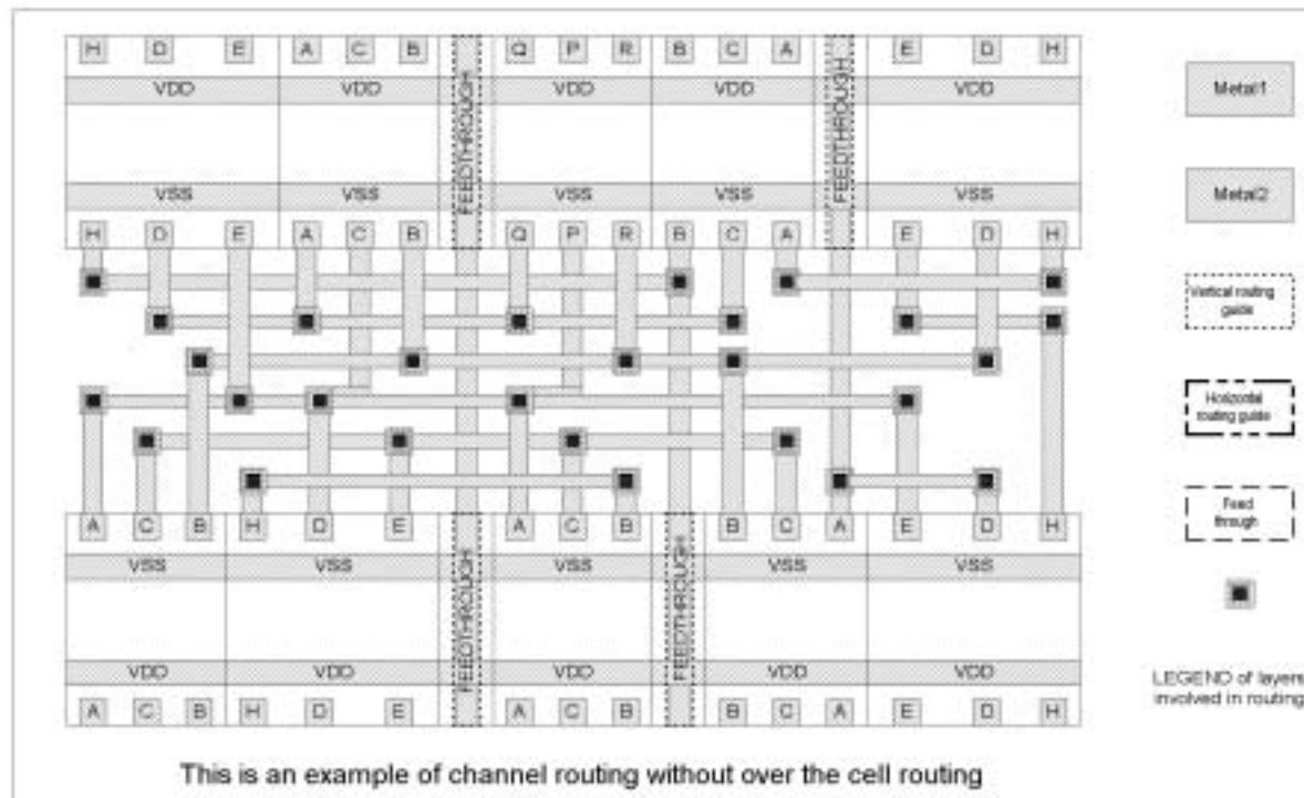
Figure 5.3 Channel routing.
