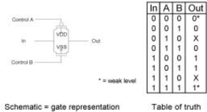
Figure 2.16 Transmission gate.
