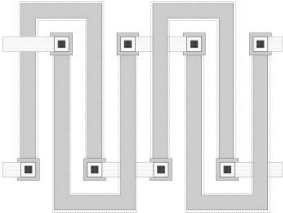
Figure 7.8 Balanced interlaced resistor.
