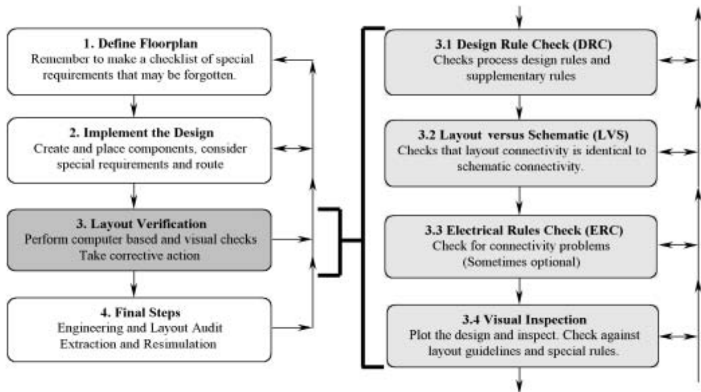
Figure 3.33 Layout verification procedure.
