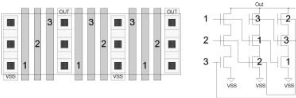
Figure 7.21 Balanced NMOS series transistors.
