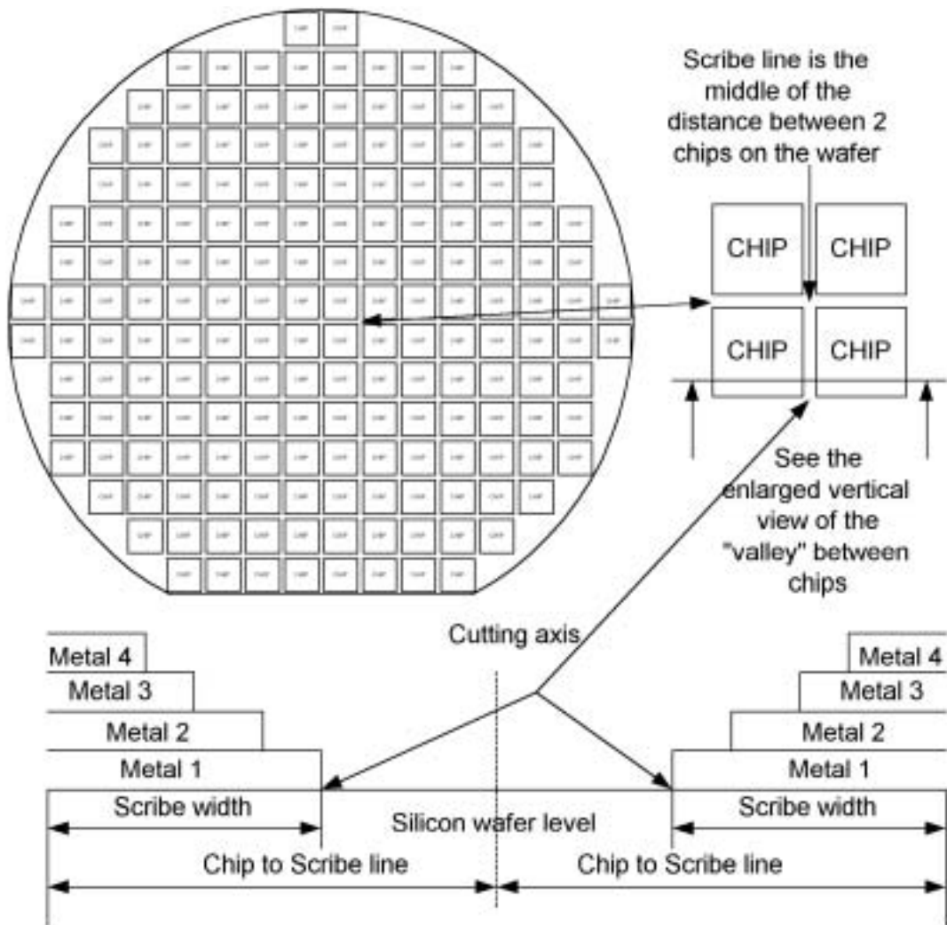
Figure 5.32 Scribe lines.
