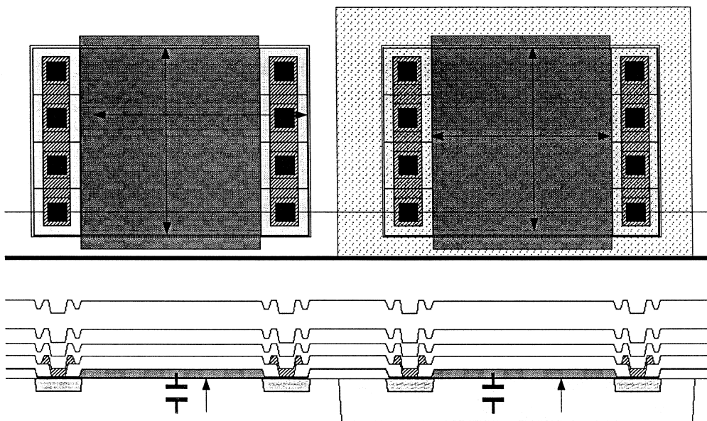
Figure 7.10 Transistor capacitors.
