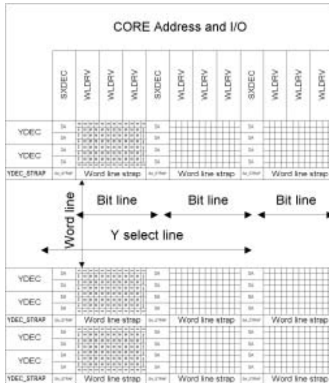
Figure 5.21 DRAM architecture.
