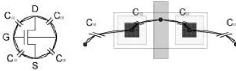
Figure 7.11 Transistor capacitance model.
