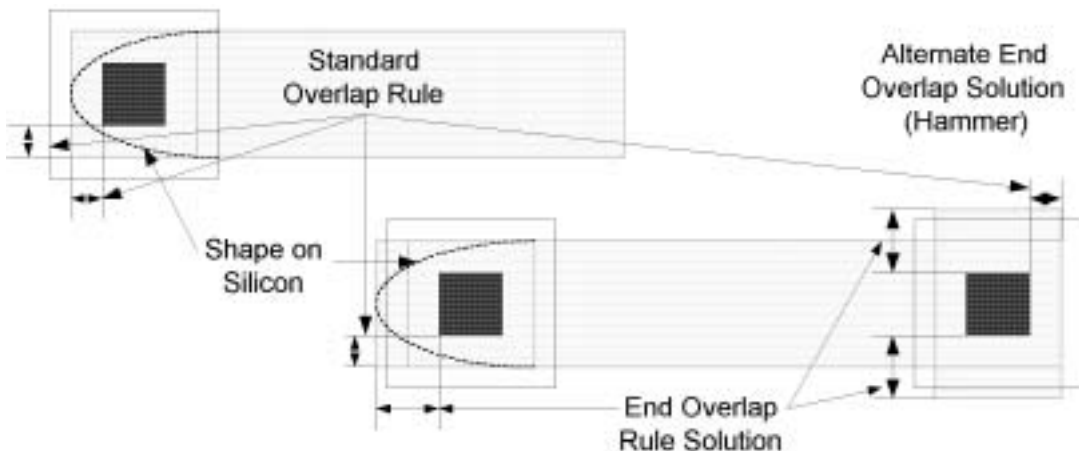
Figure 8.11 End overlap rule example.
