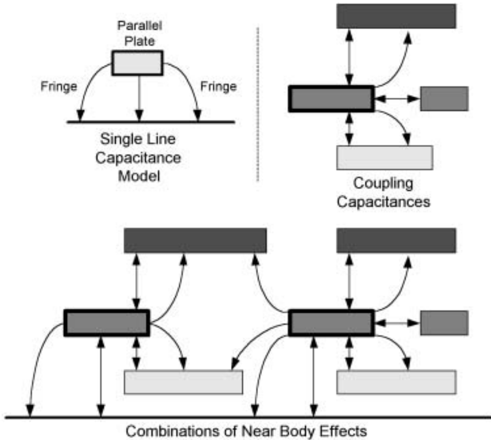
Figure 7.13 Interconnect routing capacitance examples.
