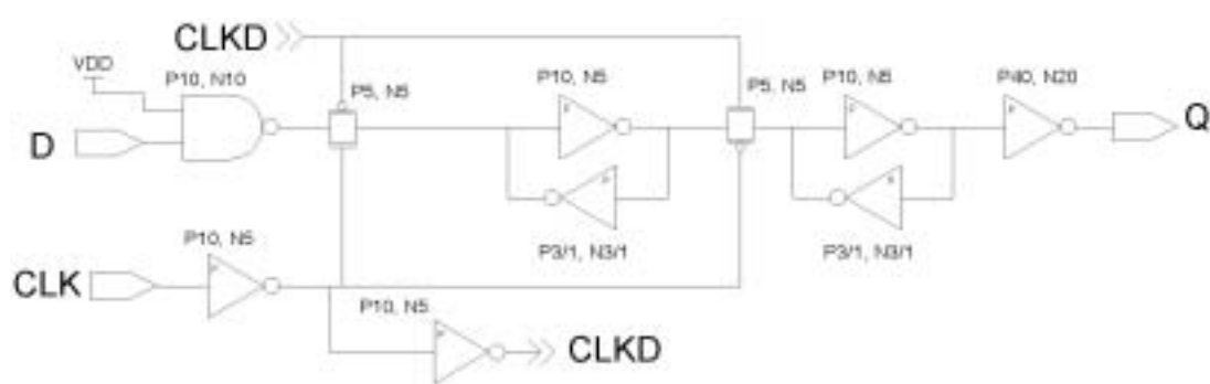
Figure 2.17 Schematic example.
