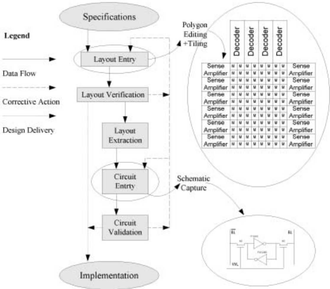
Figure 4.6 Memory IC design flow.
