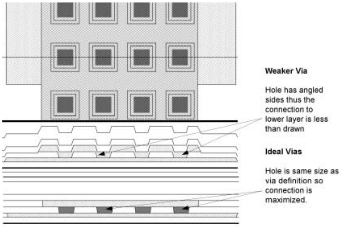
Figure 8.5 Cross-sectional view of via cuts.
