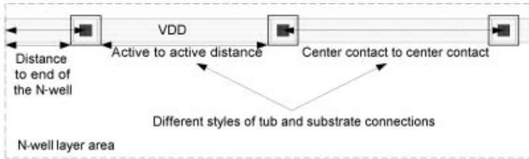
Figure 8.15 Tub connecting the N-well to VDD voltage.
