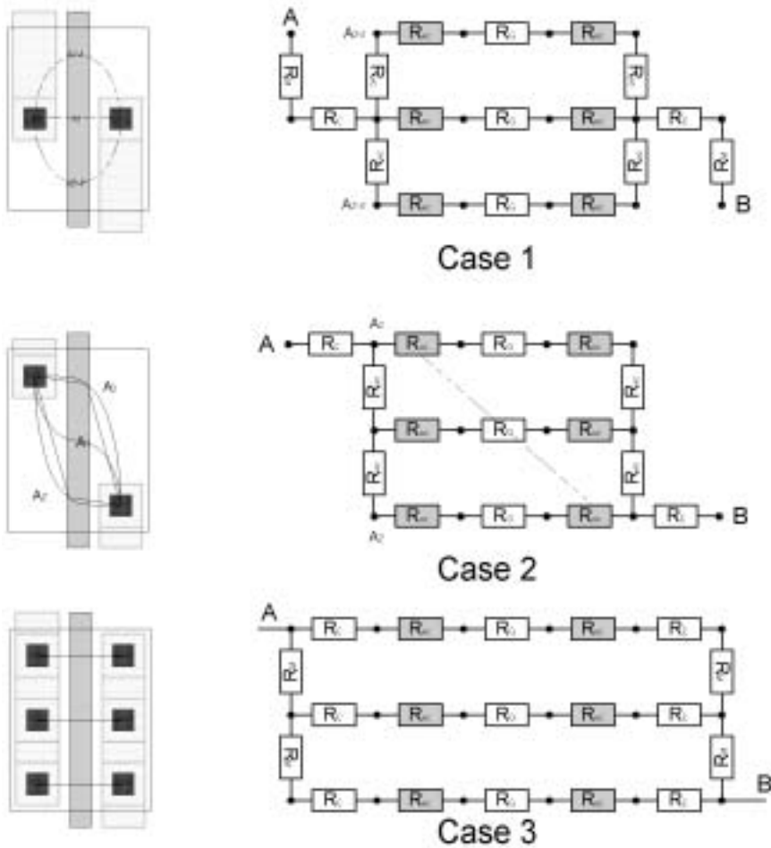
Figure 7.3 Examples of transistor contacting schemes.
