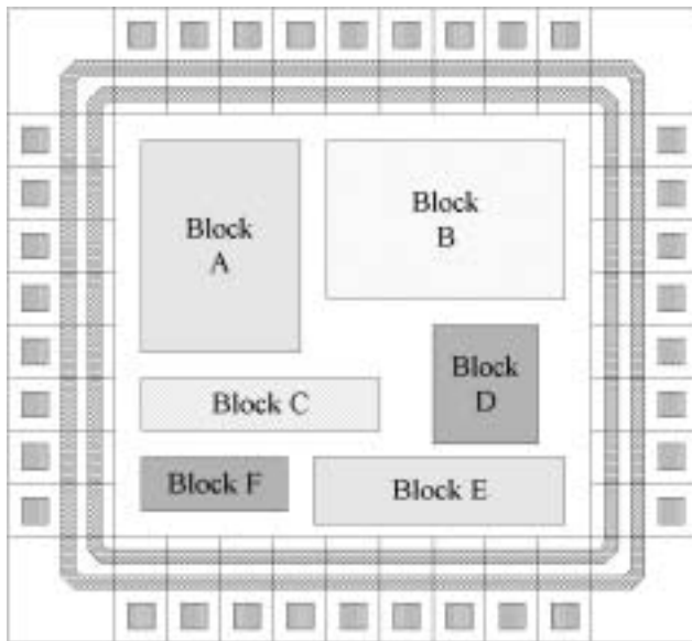
Figure 10.2 Components of a simple chip floorplan.
