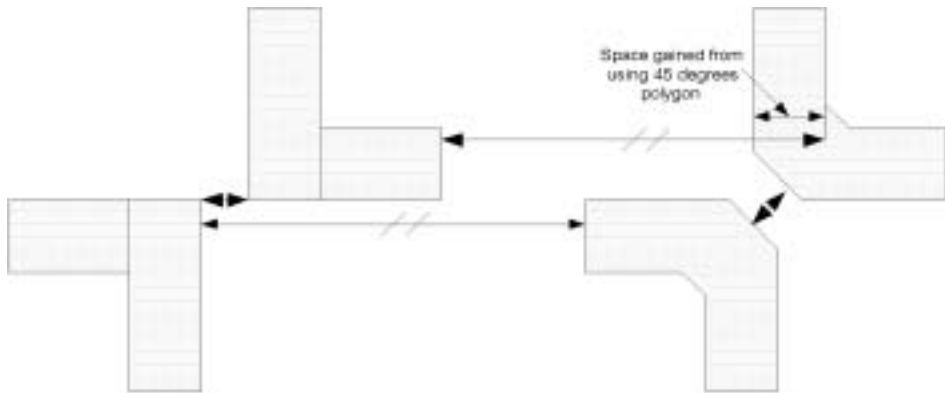
Figure 7.24 Optimal routing of wide signals.
