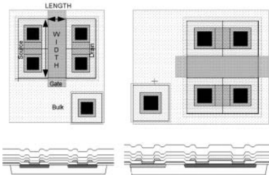
Figure 3.7 Simple PMOS transistor layout.
