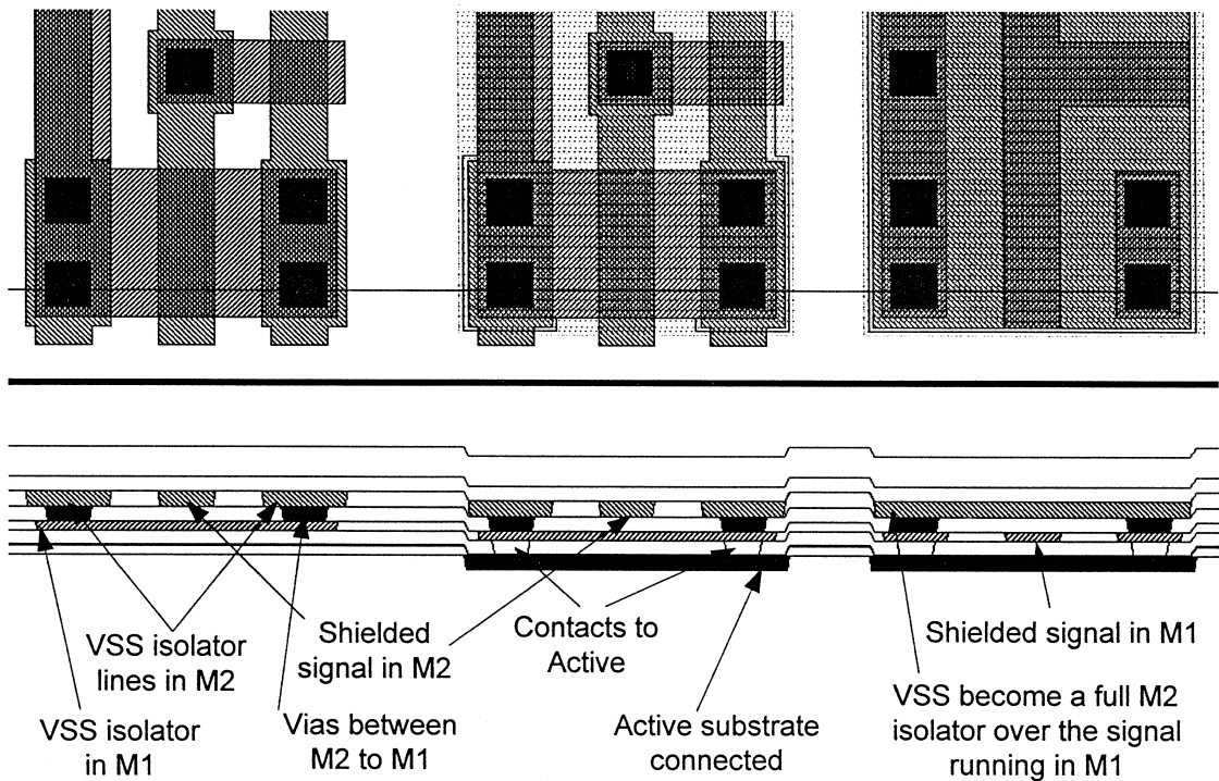
Figure 7.17 Shielding options in two-metal process.
