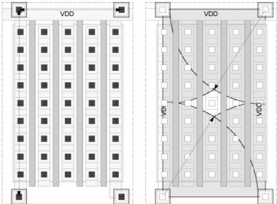
Figure 8.16 Example of tub area coverage inside N-well.
