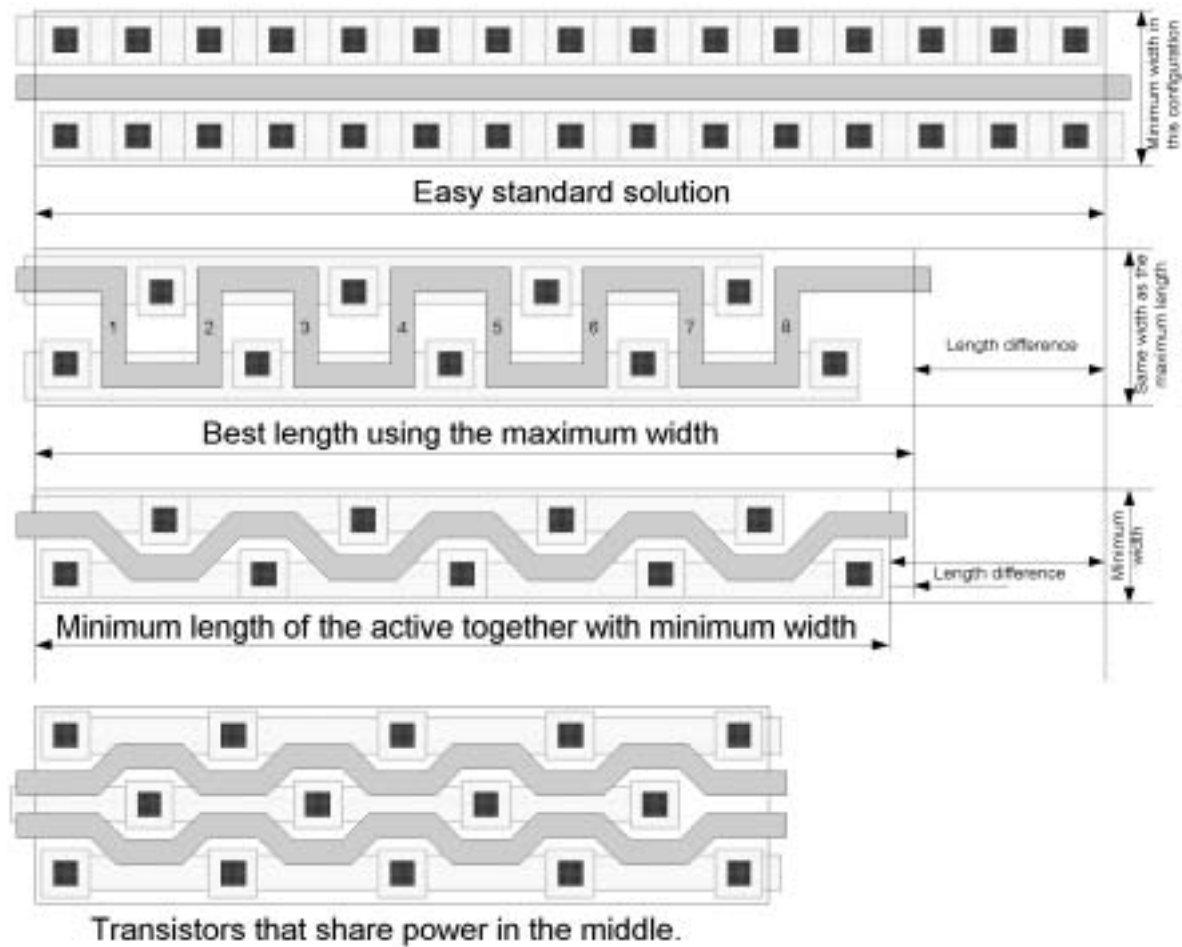
Figure 7.26 Bent transistors to minimize area.
