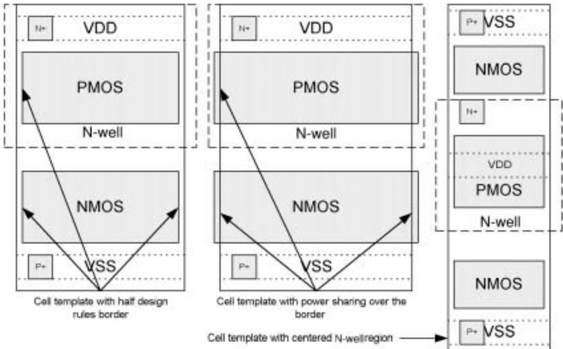
Figure 3.27 Example cell template.
