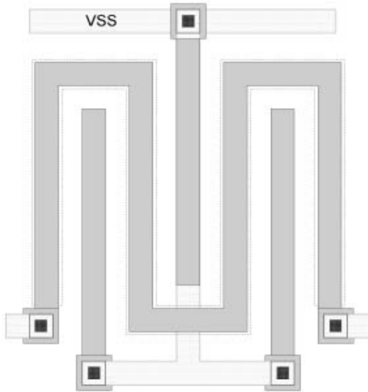
Figure 7.7 Shielded resistor.
