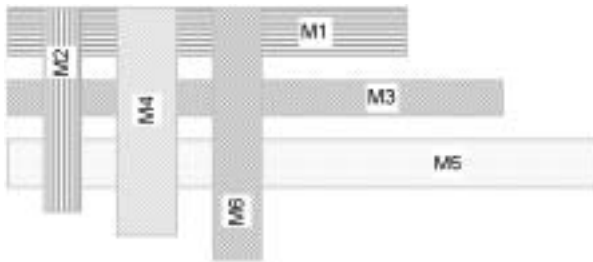
Figure 3.26 Routing direction.
