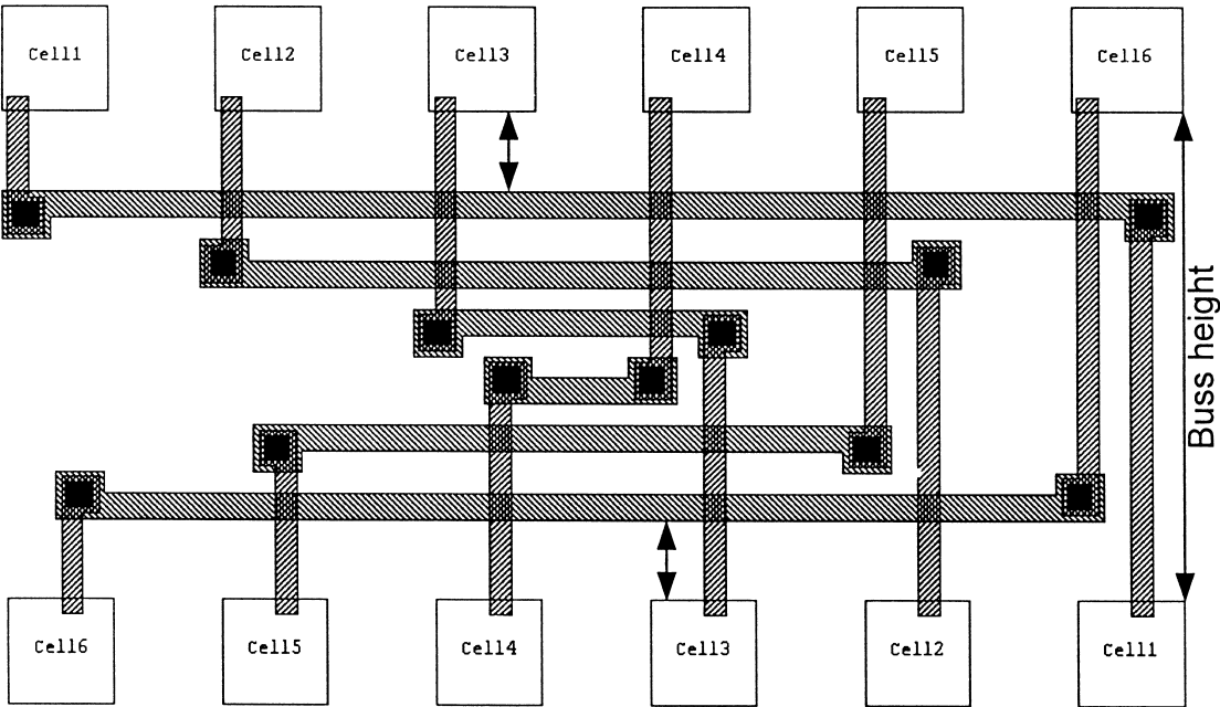
Figure 7.22 Simple bus routing.
