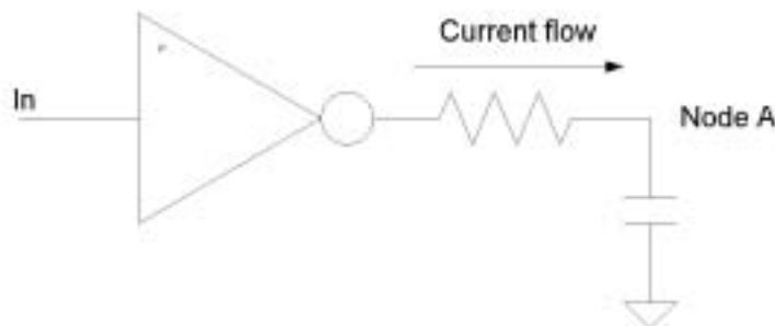
Figure 2.20 Delay calculation circuit.
