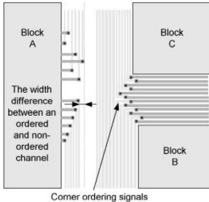
Figure 6.7 Example of channel ordering.
