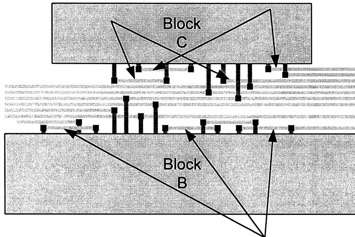
Figure 6.5 Local routing line sharing.
