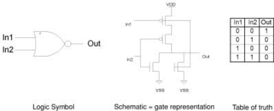
Figure 2.12 Two-input NOR gate.
