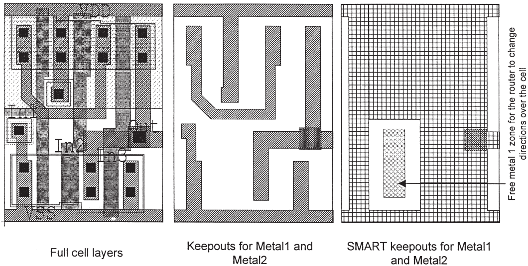
Figure 5.7A Example of cell obstructions.
