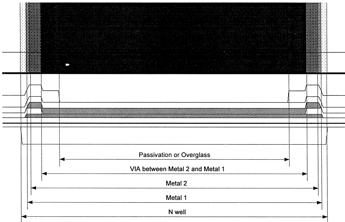
Figure 5.15 Bonding pad layout.
