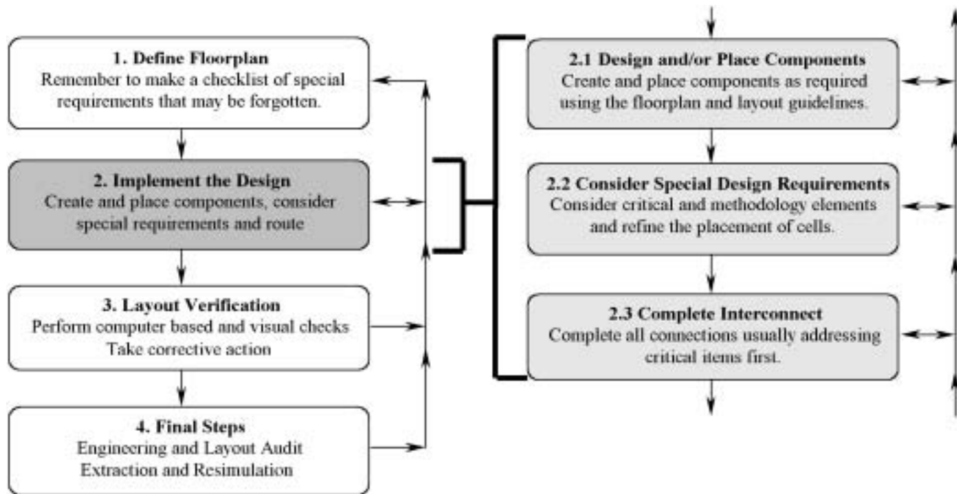
Figure 3.32 Layout implementation procedure.
