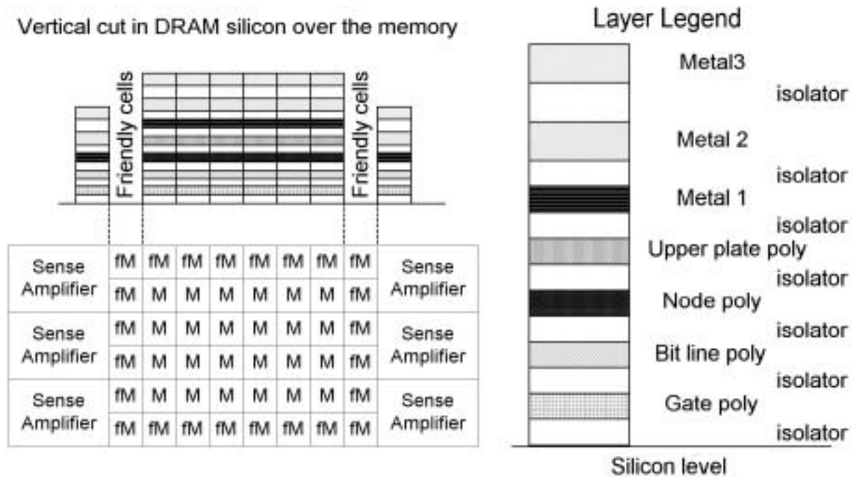
Figure 5.23 Cross-section of a typical stacked capacitor DRAM process.
