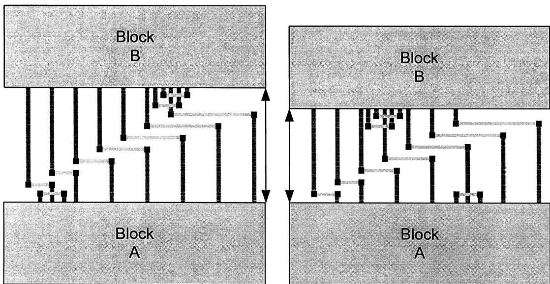
Figure 6.6 Changing cell placement to optimize routing channel.
