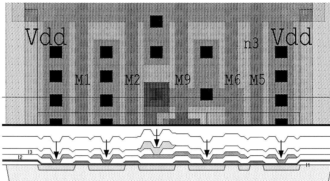
Figure 3.12 Illustration of contacts and vias.
