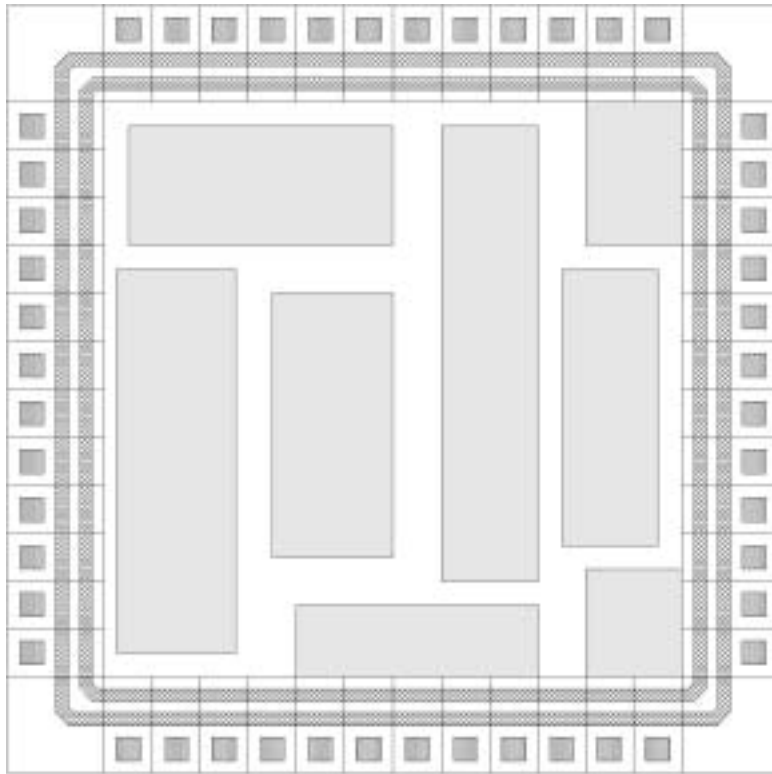
Figure 6.4 Example of chip floorplan showing signal blocks and channels.
