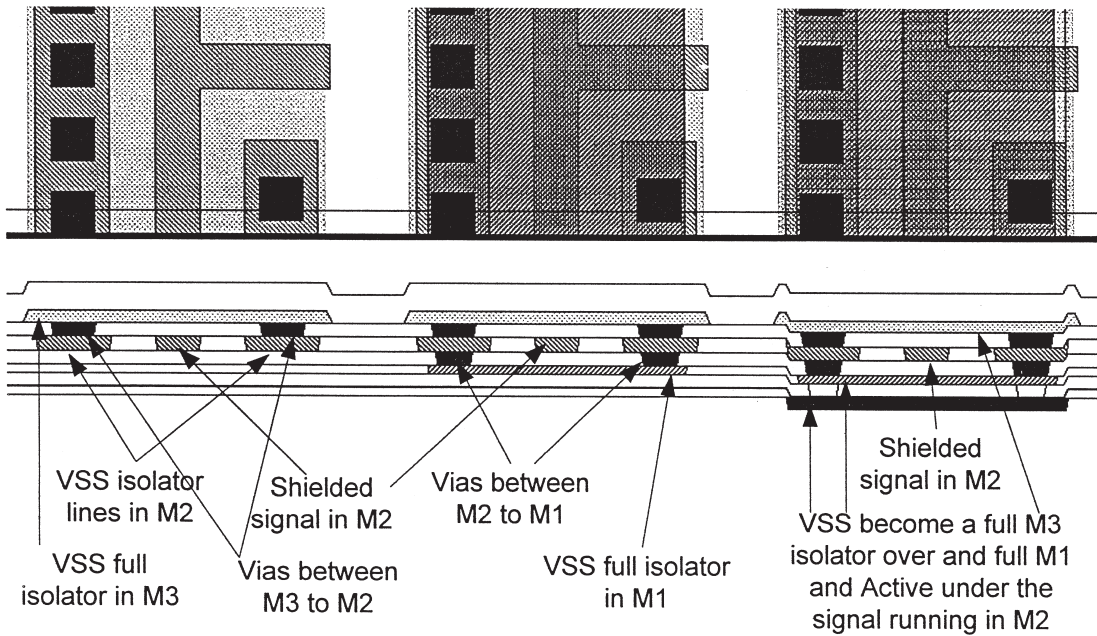
Figure 7.18 Shielding options in three-metal process.
