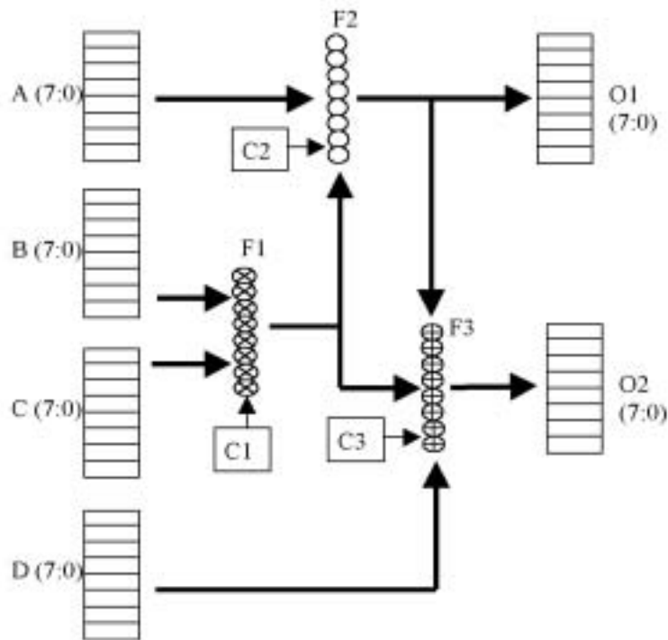
Figure 5.11 Datapath block diagram example.
