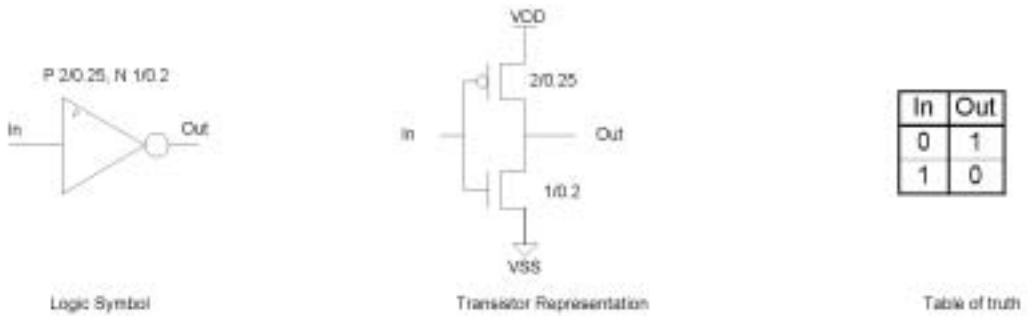
Figure 3.13 Inverter representations.
