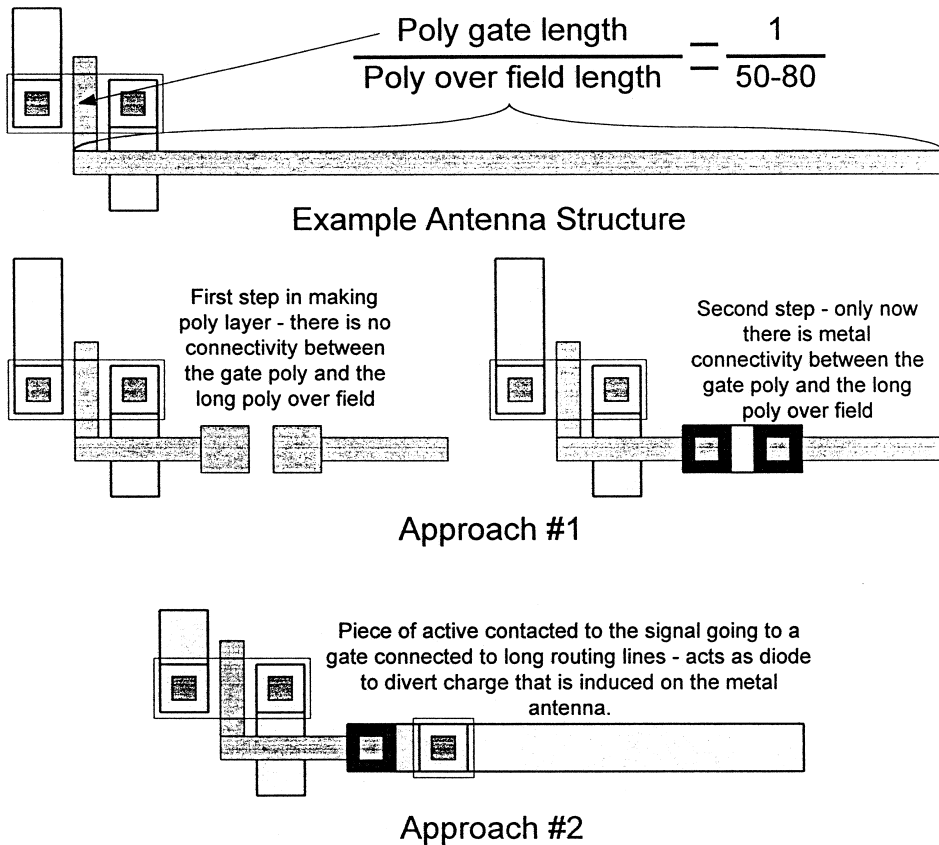
Figure 8.9 Antenna rules example and solution.
