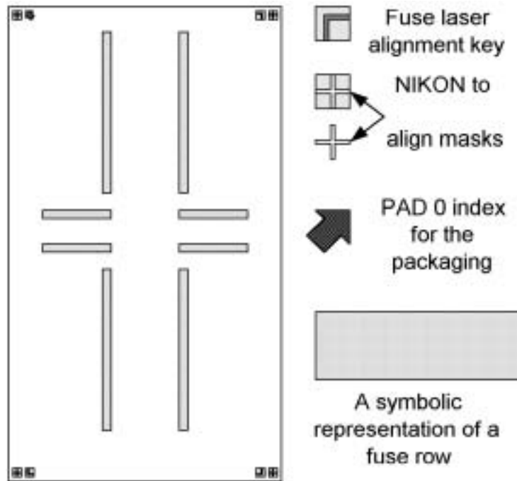
Figure 5.31 Examples of alignment keys.
