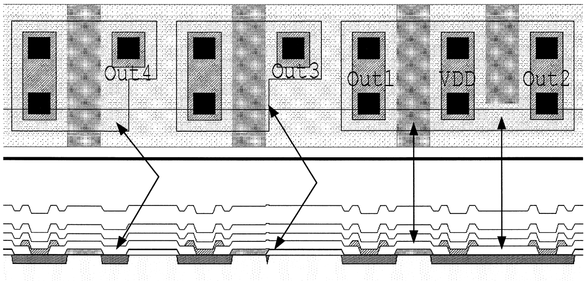
Figure 3.19 More examples of the overlap rule.
