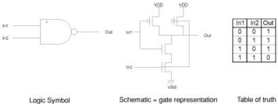
Figure 2.10 Two-input NAND gate.
