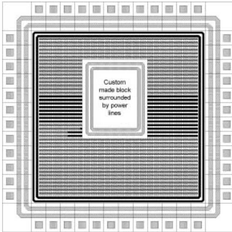
Figure 5.10 Embedded custom block in a gate array design.
