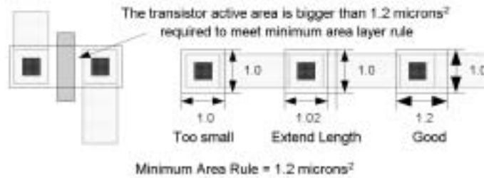
Figure 8.10 Minimum area layer example.
