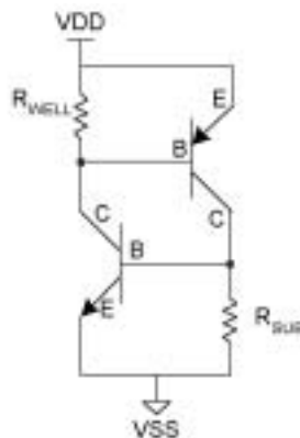
Figure 8.14 Redrawn latch-up circuit model.
