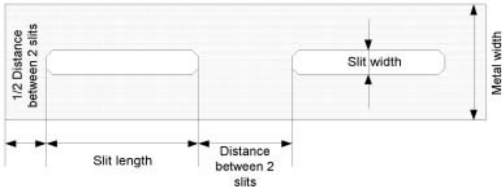
Figure 8.2 Metal slit example and design rules.
