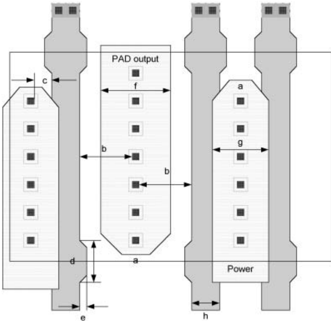
Figure 5.19 Output buffer transistor design.
