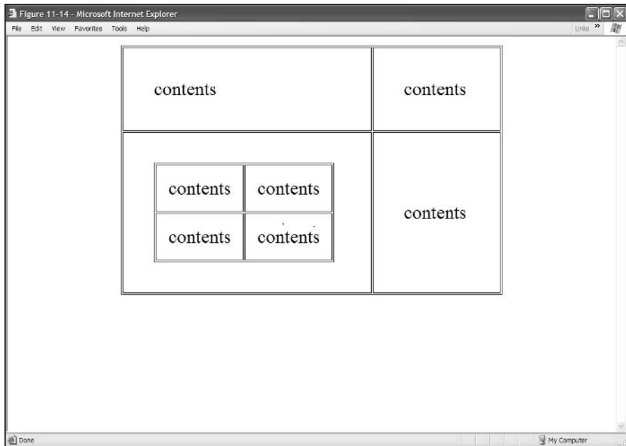
Figure 11-12: Nested tables.
