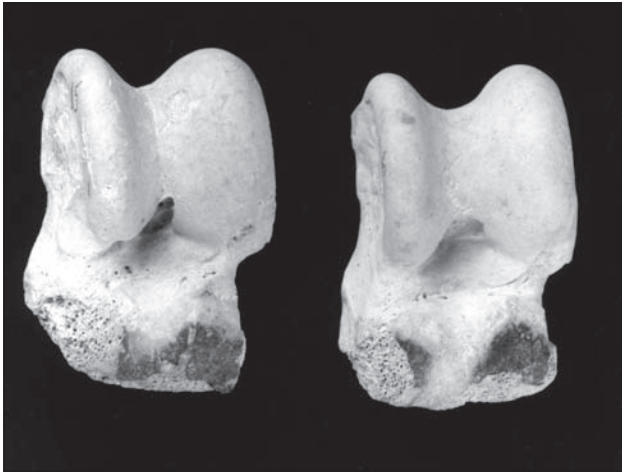
Figure 5.12. Durrington Walls. Pig astragali with burn marks and erosion of distal end.
