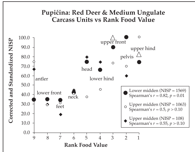
Figure 7.7. Carcass unit frequency vs rank food utility for red deer and medium ungulates from Lower Midden and Upper Midden Mesolithic phases at Pupičina Cave.
