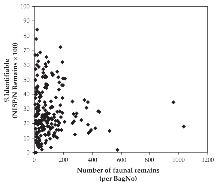
Figure 7.10. %Identifiable versus sample size by excavation lot (BagNo) at Pupičina Cave.
