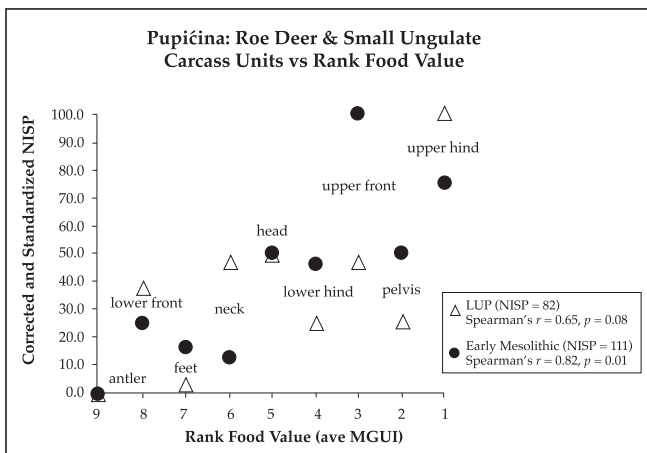
Figure 7.8. Carcass unit frequency vs rank food utility for roe deer and small ungulates from LUP and Early Mesolithic phases at Pupičina Cave.
