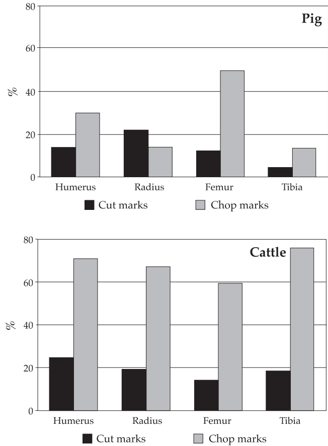
Figure 5.8. Percentage of butchered bones of pig and cattle at Durrington Walls. Pig: humerus = 404; radius = 385; femur = 239; tibia = 503. Cattle: humerus = 76; radius = 83; femur = 69; tibia = 72.
