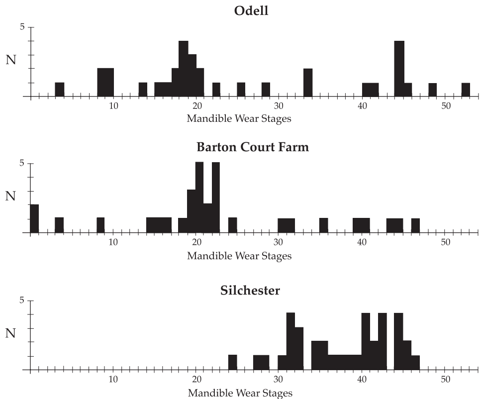
Figure 3.1. Cattle mortality profiles from three Late Iron Age sites in central southern Britain. (Mandible Wear Stages - see Grant 1982.) 1
