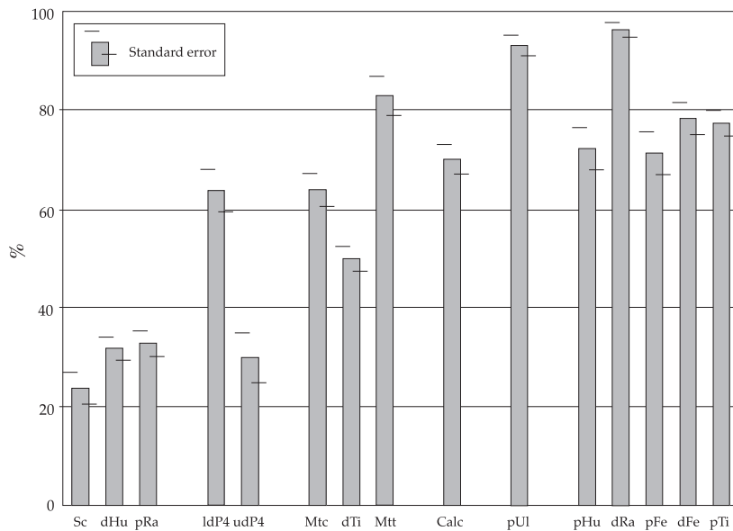
Figure 5.2. Durrington Walls. Percentages of unfused diaphyses and deciduous 4th premolars (dP4) of pig. Unfused diaphyses only were counted. The percentage of dP4s is calculated as 100 \times n \text{ dP4} / (n \text{ dP4} + n \text{ P4}) . The elements are ordered in the sequence of fusion and tooth eruption suggested by Habermehl (1975). Key: p proximal, d distal, l lower, u upper, Sc scapula, Hu humerus, Ra radius, Mtc metacarpal, Ti tibia, Mtt metatarsal, Calc calcaneum, Ul ulna, Fe femur.
