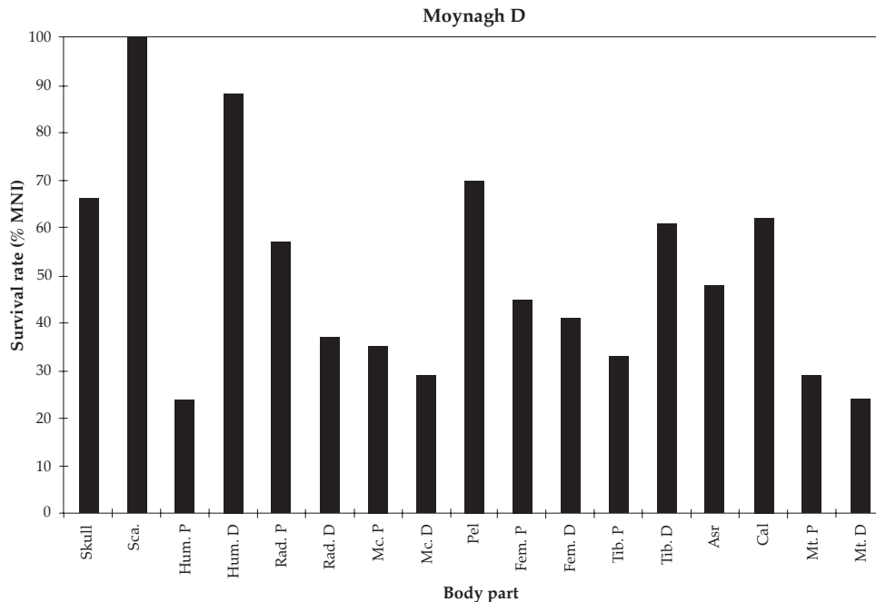
Figure 4.2. Distribution of cattle carcass parts from Moynagh crannog sample D (McCormick 1987). The survival rate is calculated by giving the part on which the minimum number of individuals (MNI) was based, a value of 100 per cent and expressing the MNI values for the other parts accordingly.
