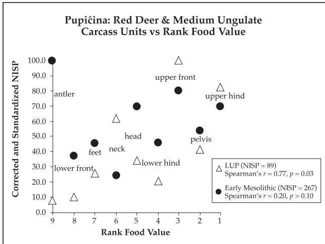
Figure 7.6. Carcass unit frequency vs rank food utility for red deer and medium ungulates from LUP and Early Mesolithic phases at Pupičina Cave.
