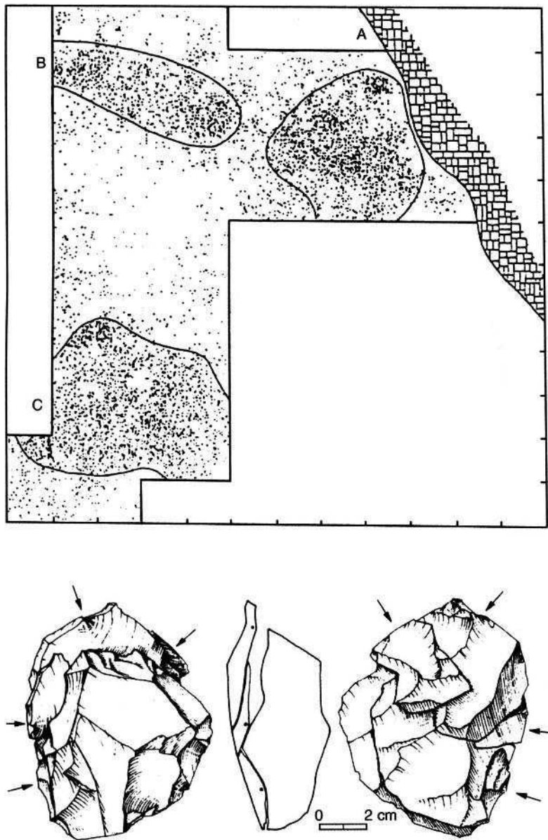
Figure 5.11. Monte Avena. Top: the horizontal distribution of implements at the quarry site, with concentrations A, B, and C (grid in meters) (after Broglio and Guerreschi 1992). Bottom: the refitting of a core (after Lanzinger 1984).
