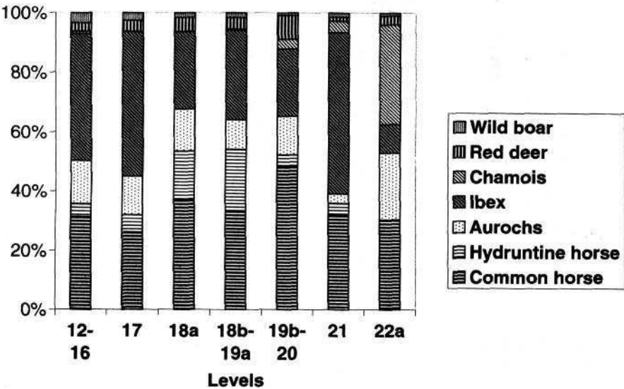
Figure 6.9. Grotta Paglicci. The ungulates of levels 22a to 12 (based on Sala 1983). Total NISP = 7,629. Capreolus capreolus the roe deer, totaling four more specimens, is omitted.
