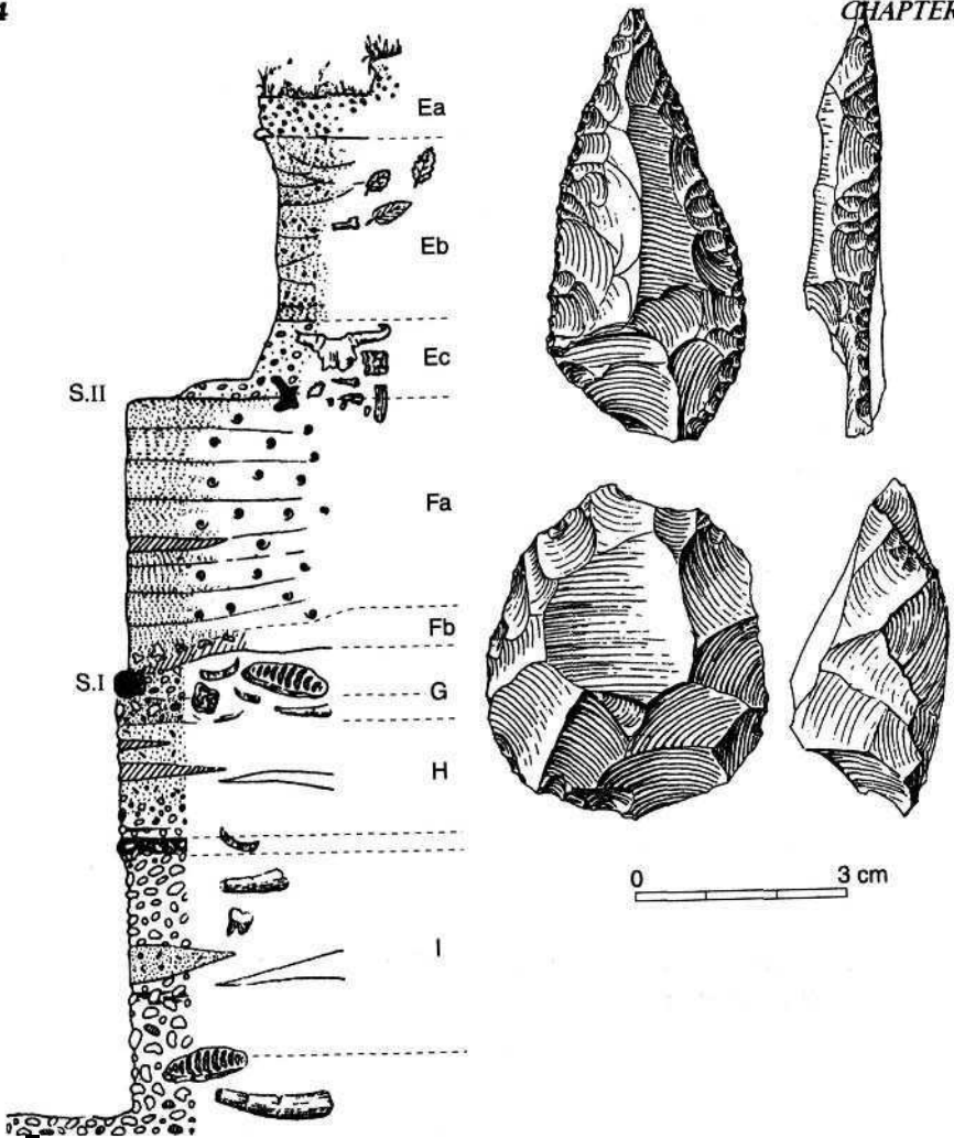
Figure 4.6. Saccopastore. Left: the stratigraphic sequence, showing the position of the skulls Saccopastore I (SI) and Saccopastore II (SII) (after Segre 1948). Right: a Mousterian point and a discoidal core from level E a–c (source: Blanc 1938–1939).
