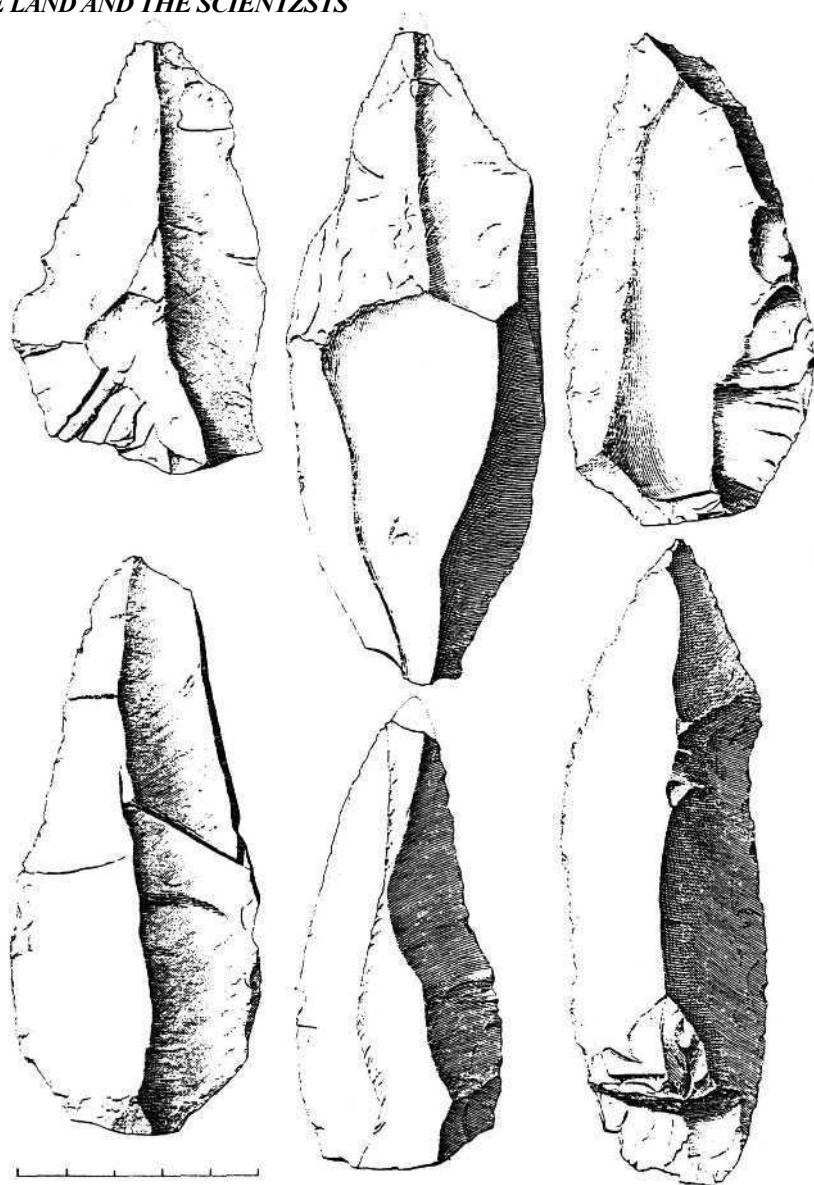
Figure 1.3. Grotta di S. Teodoro. The lithic industry, as illustrated by F. Anca in 1867 (scale in cm).
