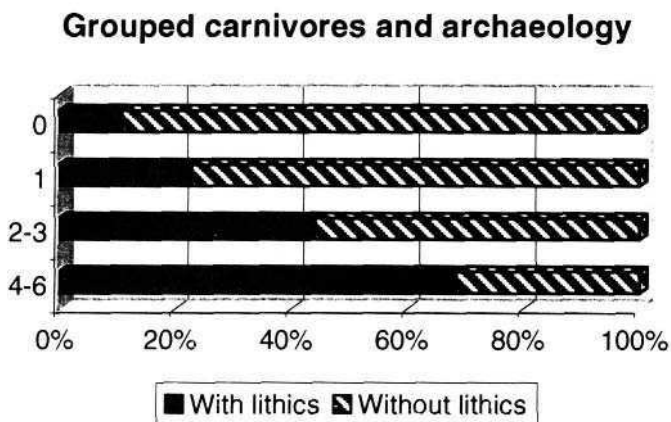
Figure 4.19. The competition for caves. Compared frequency of carnivore species at 193 paleontological and archaeological sites (OIS 7 to 3), based on presence-absence counts (after Mussi in press). The carnivores are bears (brown bears and cave bears), hyenas, wolves, lions, leopards, and lynxes.
