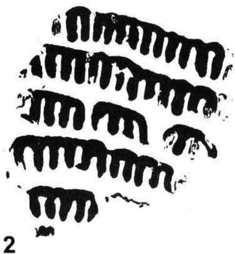
Figure 7.32. Grotta Romanelli. Block from the final Pleistocene deposit, with a geometric pattern originally painted in red (after Blanc 1938–1939).
