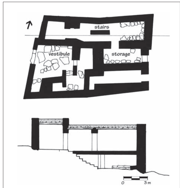
9.31. Plan and section. House Ad, Gournia. After Gournia , plan.
