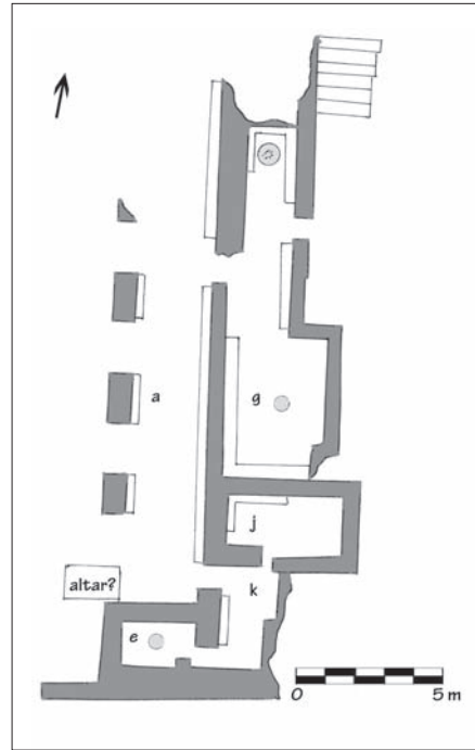
4.15. Plan. Building east of Chrysolakkos, Malia. After H. van Effenterre 1980, fig. 230.
