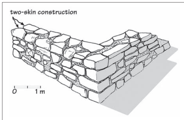
2.1. Reconstruction. Rubble wall.
