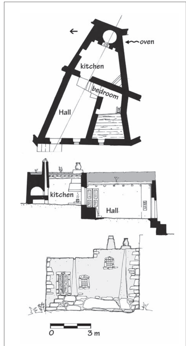
9.28. Plan, section, and elevation. Modern traditional house, Achladia. After Vasileiades 1976, fig. 148.
