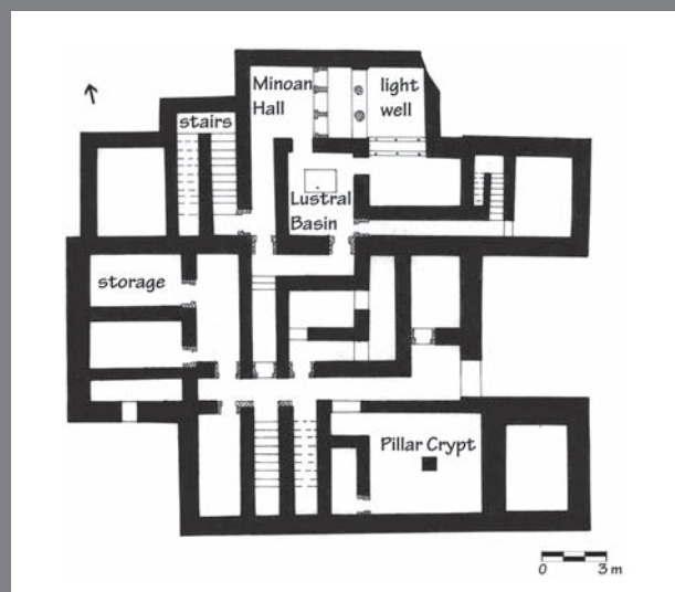
9.20. Plan. House C, Tyllissos. After Hazzidakis 1934, Pl. 6.
