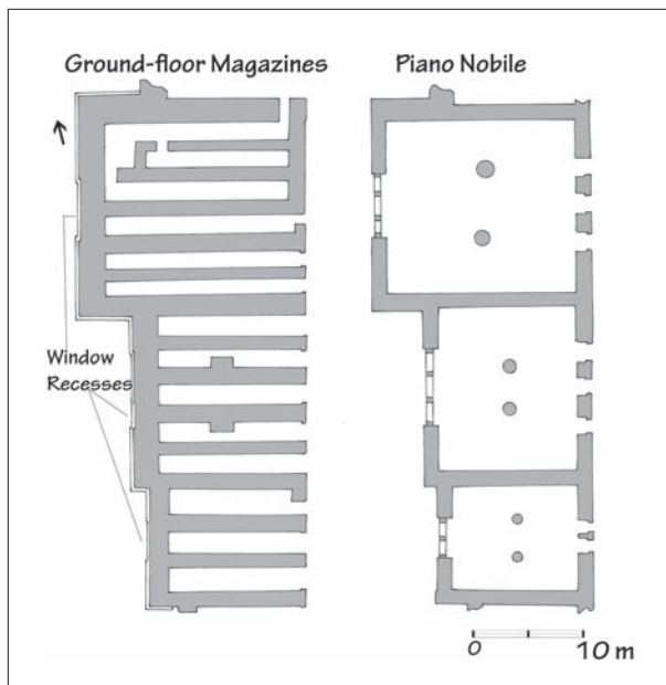
7.8. Plan. Piano Nobile according to Graham. After PoC , fig. 85.
