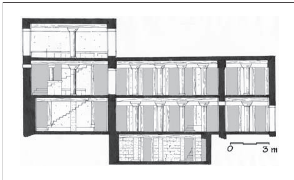
9.5. Section. South House, Knossos. After PM II , fig. 208.
