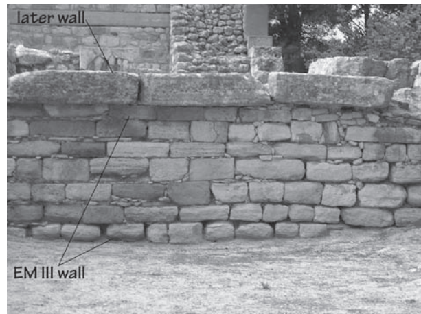
4.17. EM III facade, Palace at Knossos. Photo by author.
