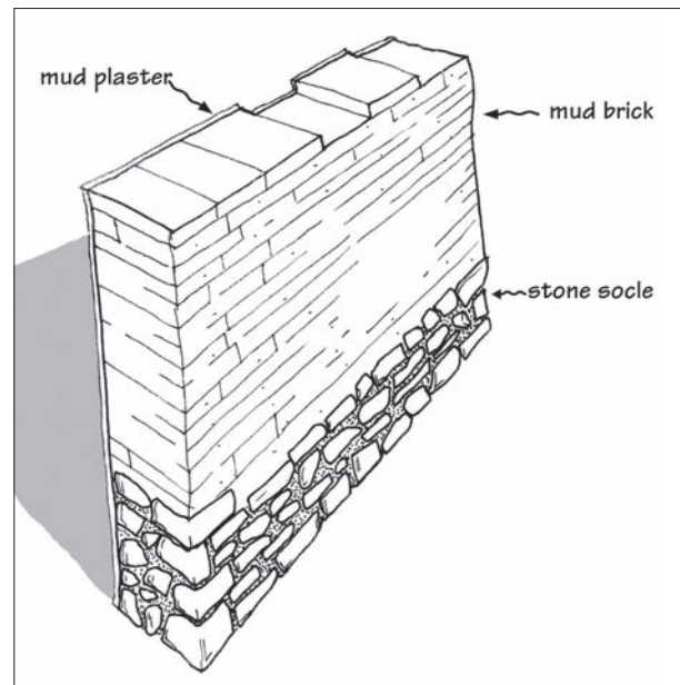
2.2. Reconstruction. Mud brick on rubble socle.
