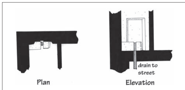
9.51. Restored plan and section. Toilet in Room 4a, West House, Akrotiri, Thera. After Palyvou 1986, fig. 6.
