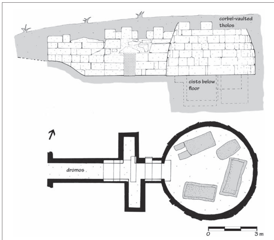
10.10. Plan and elevation. Kephala Tholos, Knossos. After Hutchinson 1962, fig. 58.
