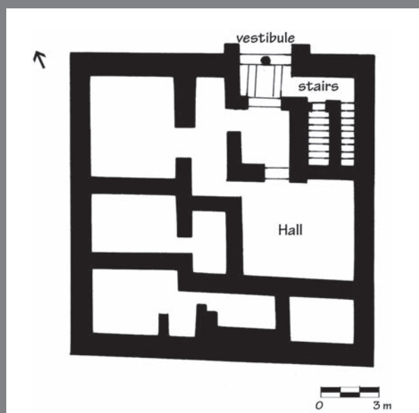
9.25. Plan. House G, Zakros. After Hogarth 1900-1901, p. 138, fig. C.
