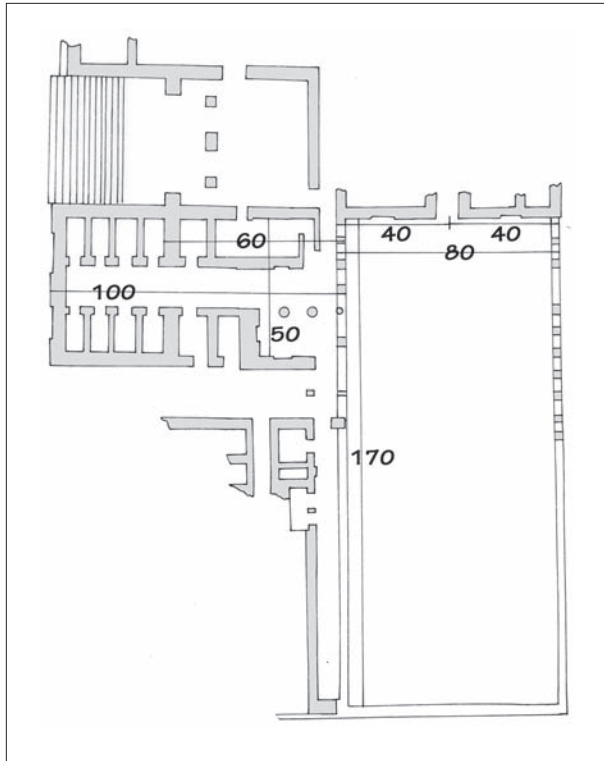
8.9. Design of Palace at Phaistos according to Graham's Minoan foot. After PoC, fig. 144.
