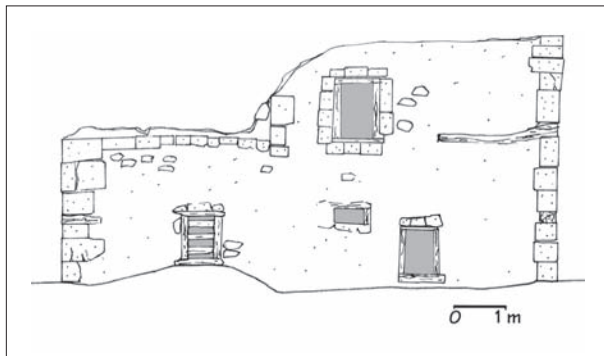
9.52. Elevation. West facade, West House, Thera. After Palyvou 1986, fig. 7.
