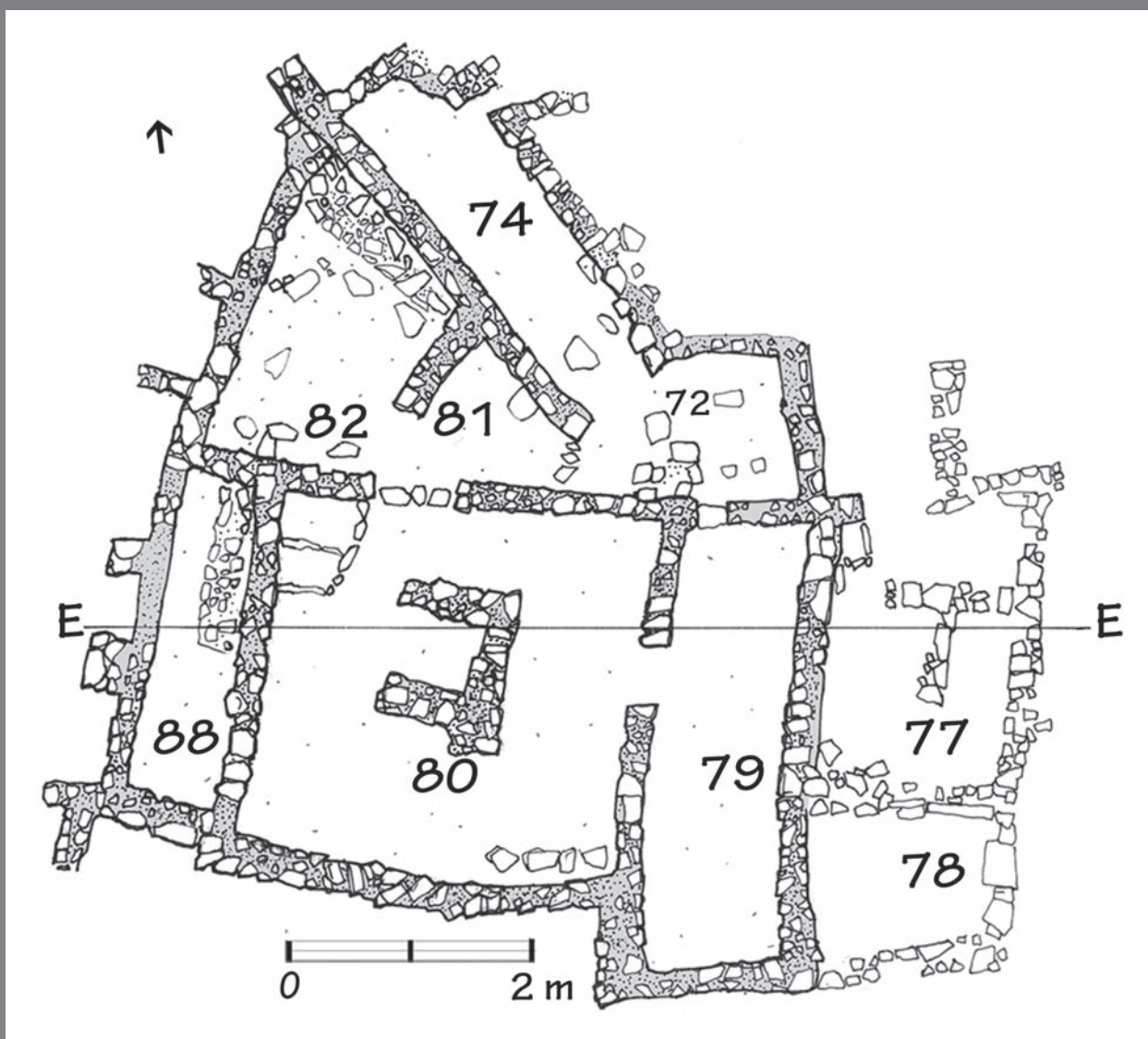
3.4. Plan. South Central House, Myrtos. After Warren 1972, plan.
