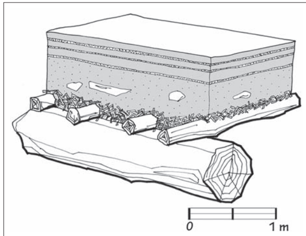
2.3. Construction of a flat roof.
