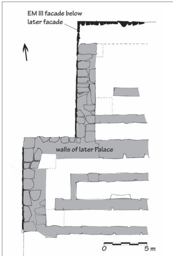
4.16. Plan. EM III facade, Palace at Knossos. After Graham 1987, fig. 158.
