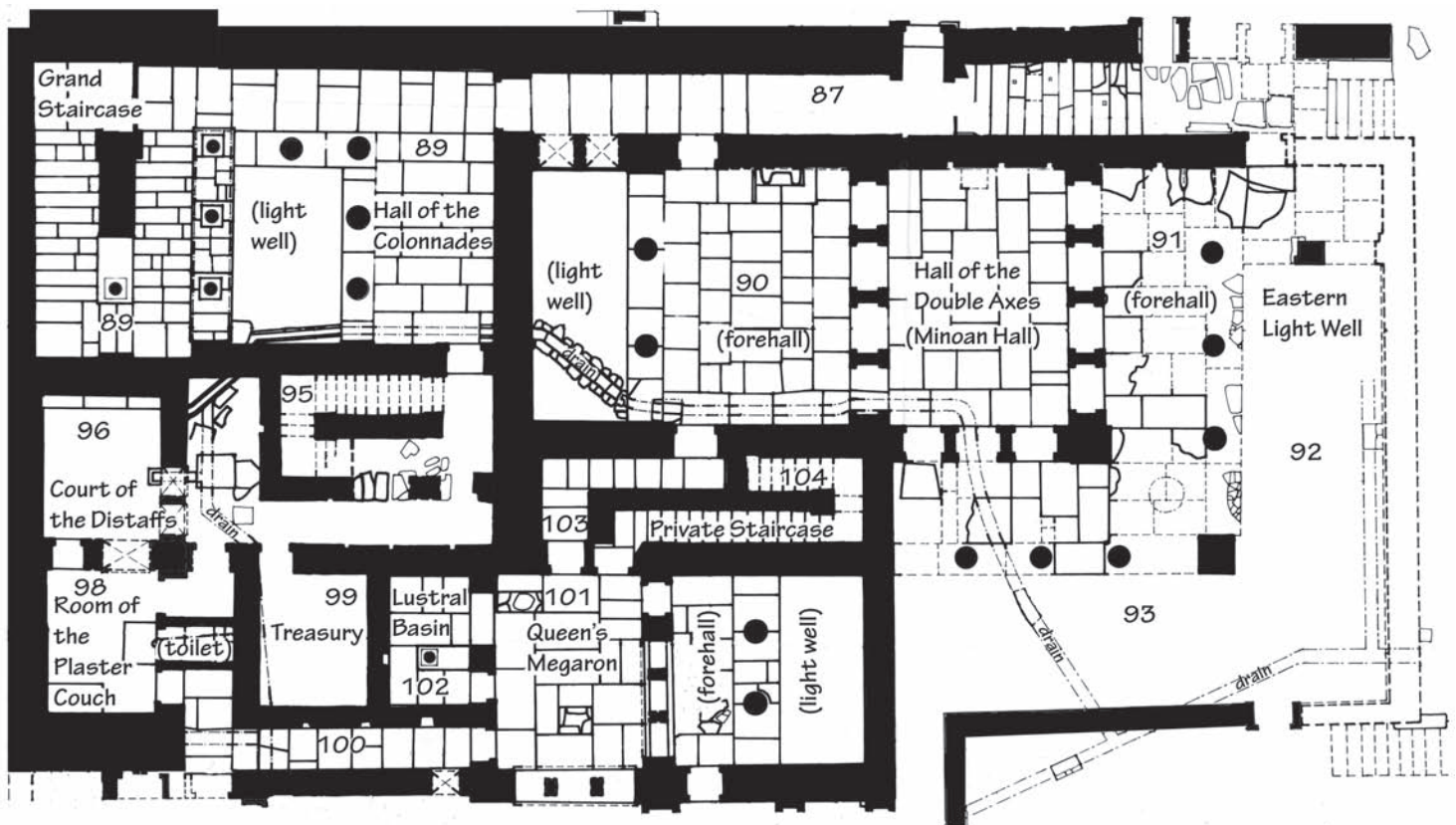
7.9. Plan. Residential Quarter. After Hood and Taylor 1981, Plan.
