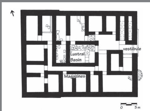
9.21. Plan. House B, Tyllissos. After Hazzidakis 1934, Pl. 6.
