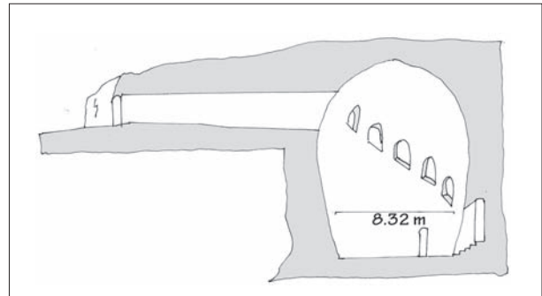
4.18. Restored section. Hypogaeum, Knossos. After PM I , fig. 74.
