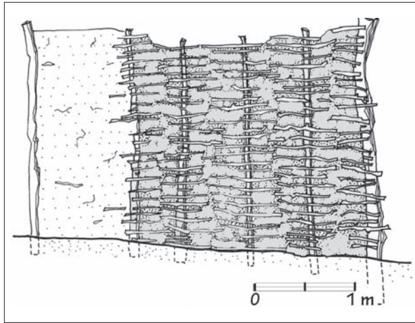
2.6. Reconstruction. Wattle-and-daub wall. After Theochares 1973, fig. 149.
