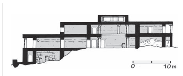
8.12. Restored section. So-called Palace, Gournia. After Soles 1979, p. 13, fig. 3.
