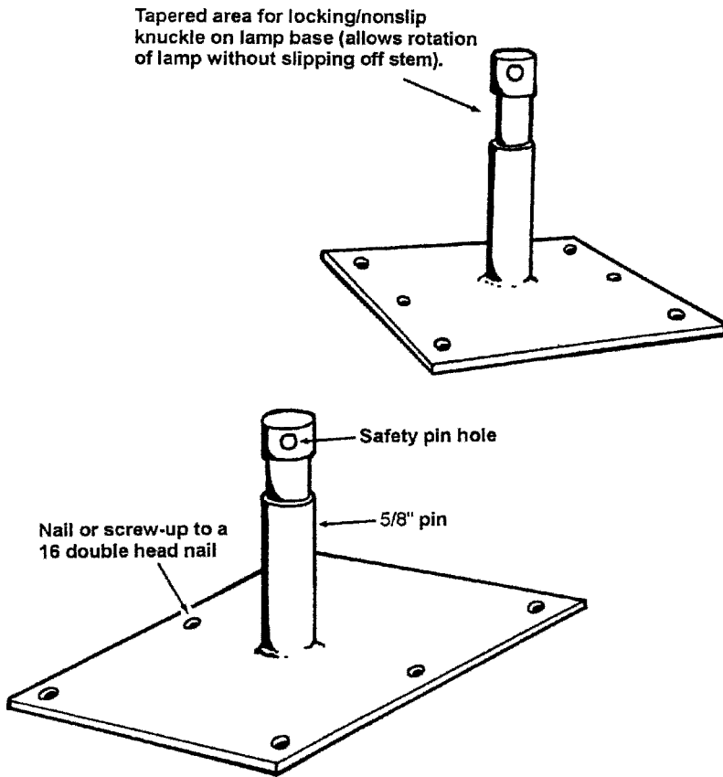
Figure 2.2 Baby plates.
