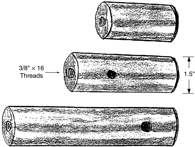
Figure 7.15 Starter plugs (smooth) for Speed-Rail® 1-1/2" (Modern Equipment Company).
