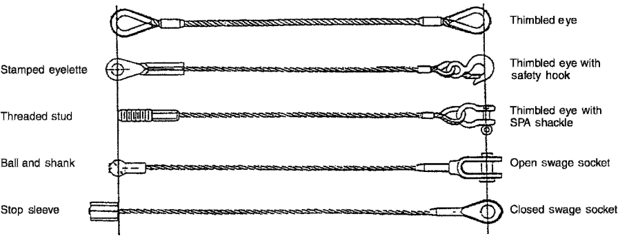
Figure 8.1a Miniature cable ends.
