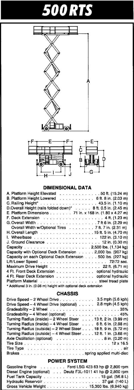
Figure 9.2 Scissors lift with extending platform.
