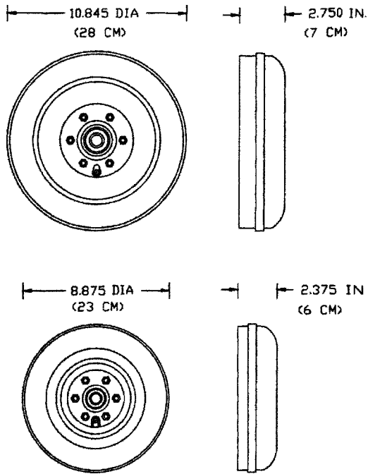
Figure 14.28 Pneumatic wheels (PNE).
