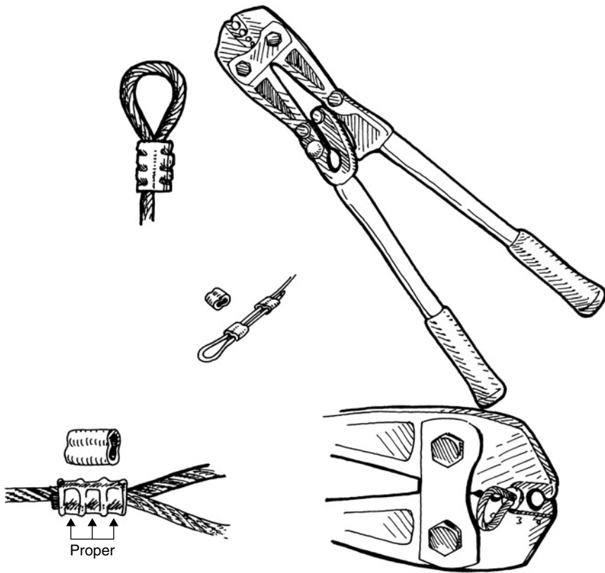
Figure 8.1b Handheld nico press for sleeves.
