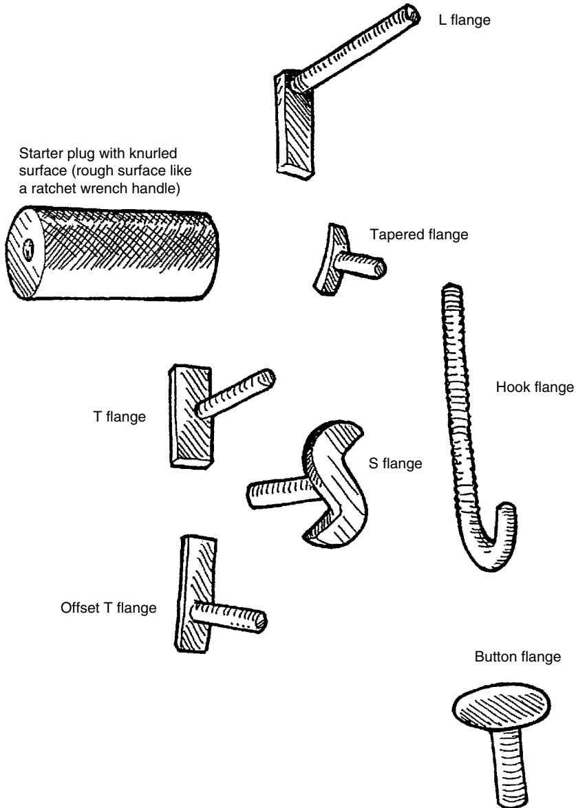
Figure 7.17 Speed-Rail® starter plug flanges for auto frames ( 3/8" \times 16 pitch thread) (Modern Equipment Company).
