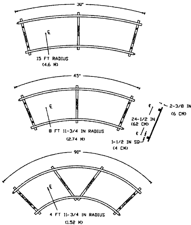
Figure 14.27 Square curved track.
