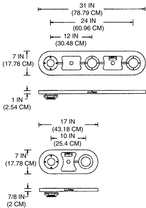
Figure 14.12 Offsets (nicknamed "Ubangie").
