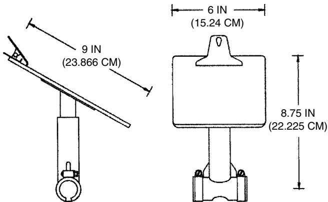
Figure 14.9 Cue board.
