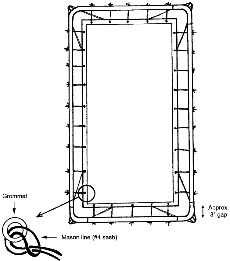
Figure 2.32b Griffon.
