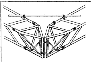
18" POINT ADAPTER
