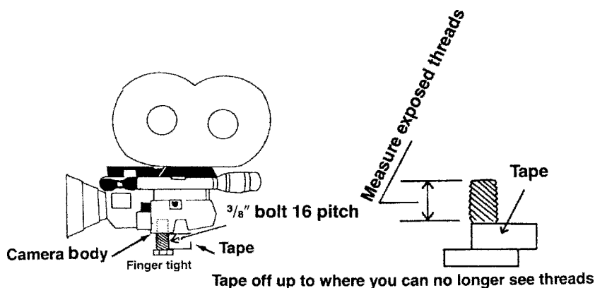
Figure 7.2 Tape method.
