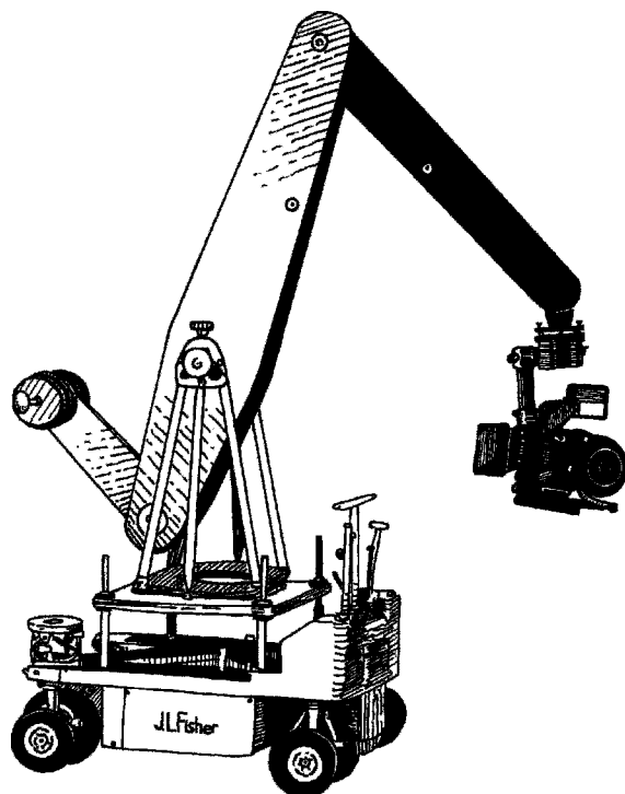
Figure 10.17 Z-Jib Arm (Model 6-200) on Fisher Dolly (Ken Hill Mfg.).
