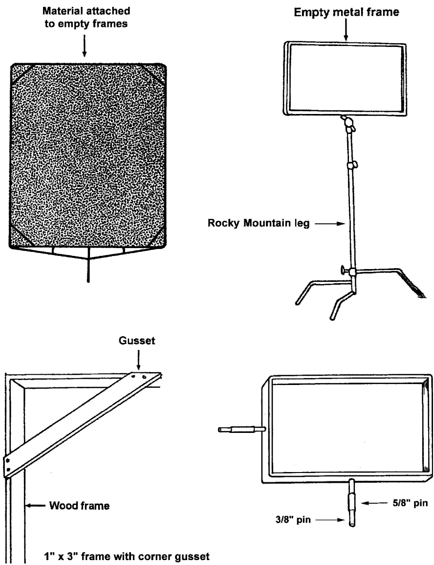
Figure 2.24 Empty frames.
