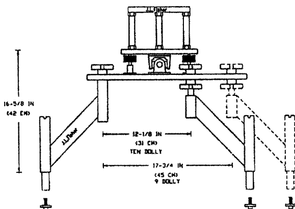
Figure 14.11 Center mount kit.
