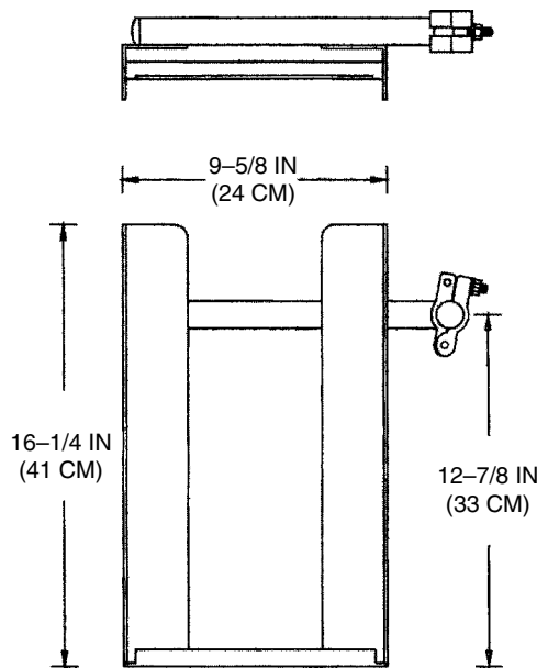
Figure 14.19 Monitor rack (MRD).
