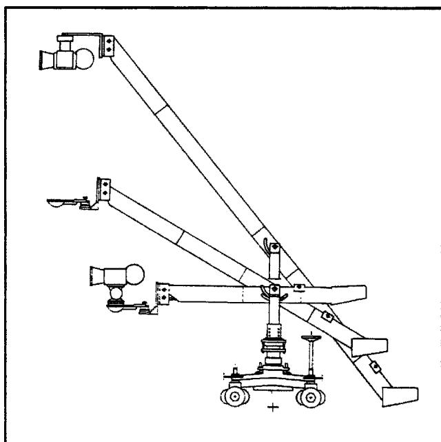
Figure 10.28b Aero Jib/Arm.
