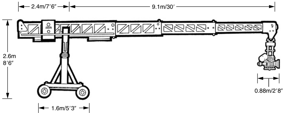
Figure 10.37 Super Technocrane.
