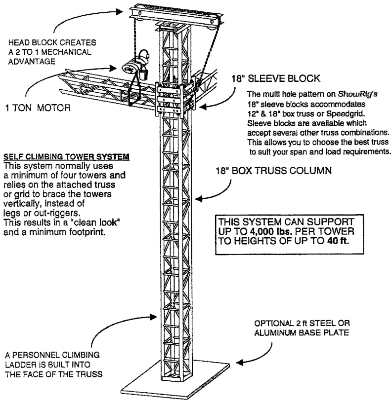
Figure 7.36 (Continued) ShowRig tower system.
