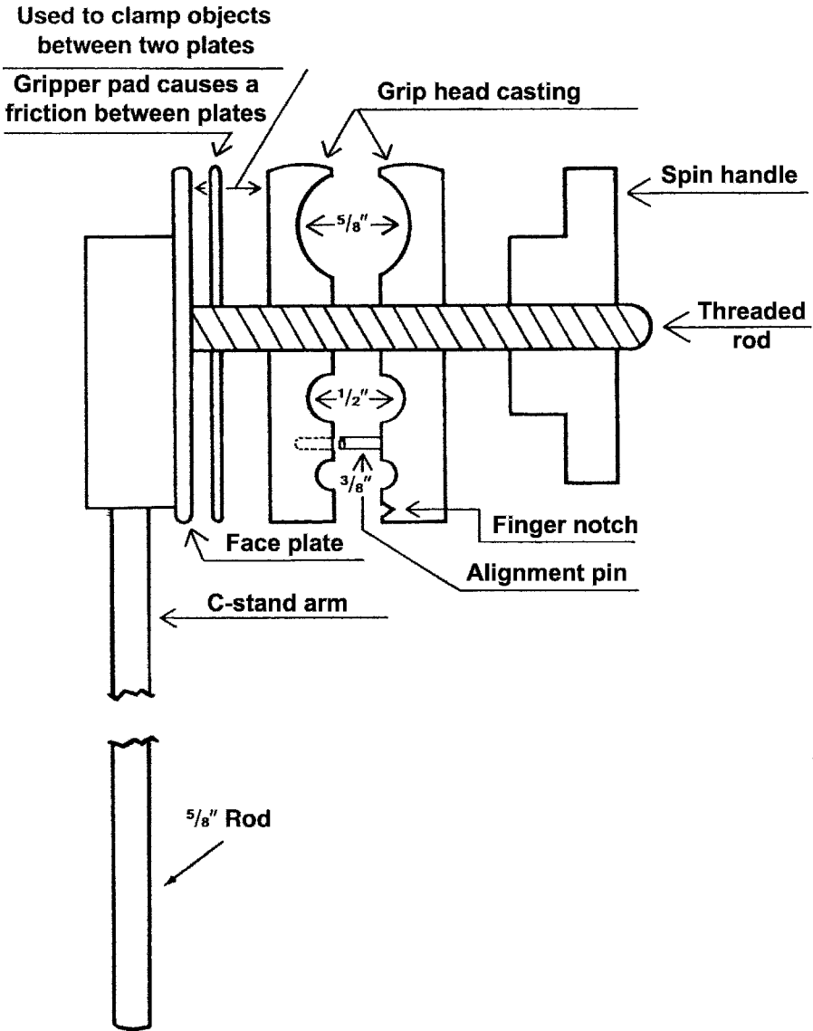
Figure 2.60f C-stand head.
