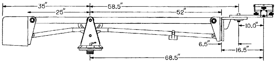
Figure 10.25b Fisher Jib/Arm, Model 21 (J. L. Fisher Mfg.).
