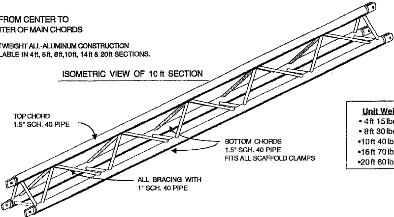
Figure 7.36 (Continued) ShowRig triangle trusses.
