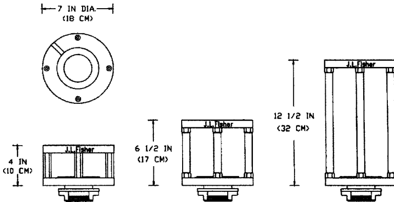
Figure 14.14 Rishers, 4", 6-1/2", and 12-1/2".
