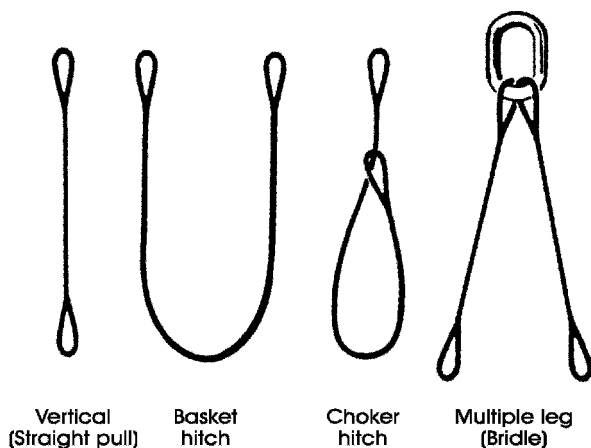
Figure 8.3a Slings.
