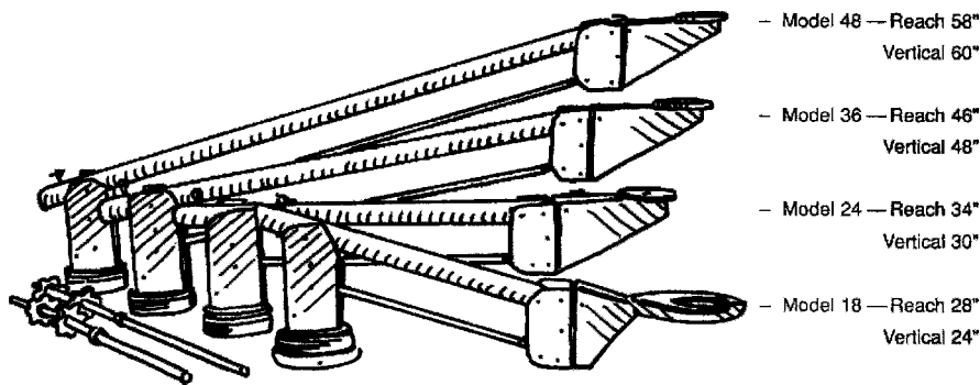
Figure 10.4 Trovato Tote Jib (Trovato Manufacturing, Inc.).
