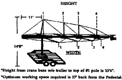
Figure 10.45b The Akela Crane.
