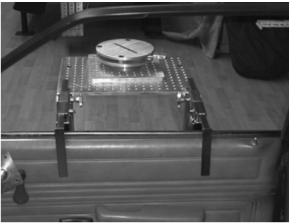
Figure 19.30 Hostess tray (car side camera mount).
