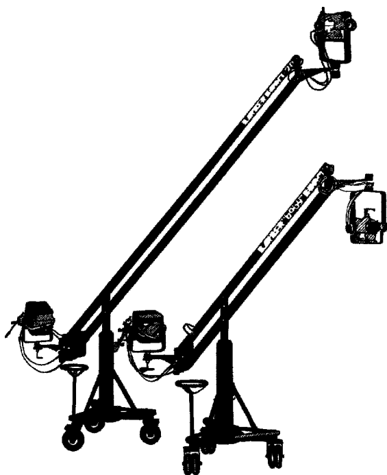
Figure 10.29a Barber Baby Boom and Barber Boom 20.
