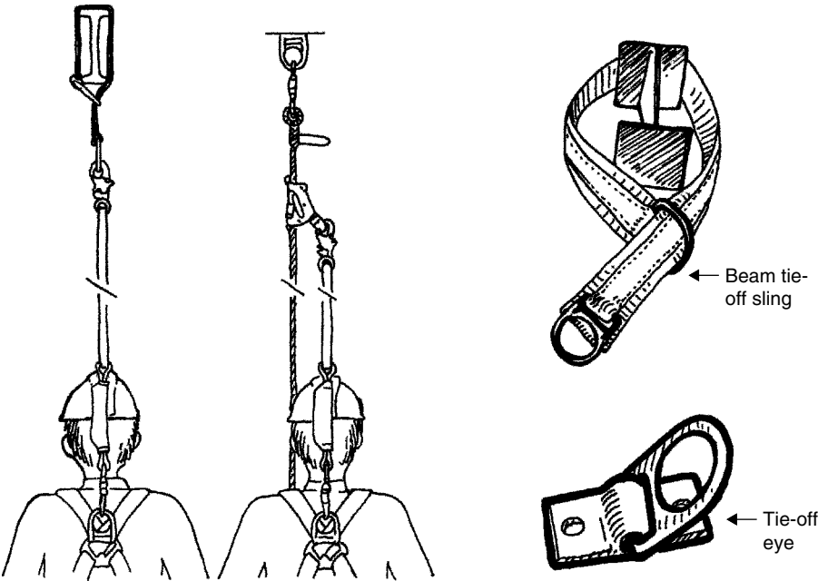
Figure 9.3b Example of attach point.
