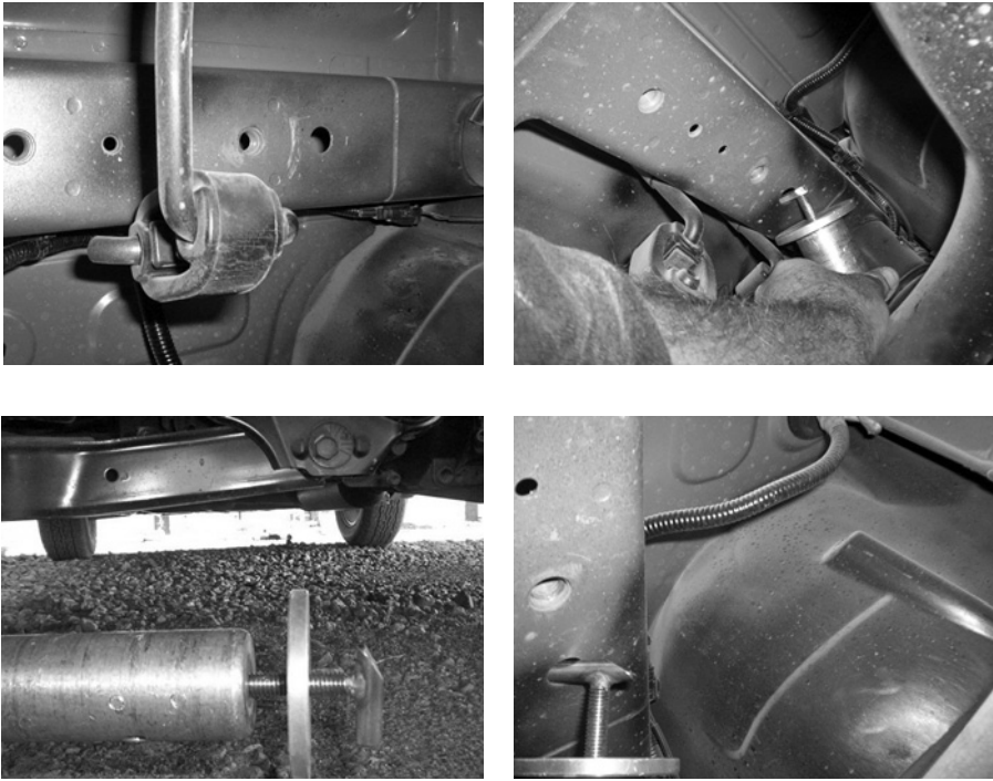
Figure 19.21 The undercarriage of a car will usually have several holes to “get a bite” using starter plugs.
