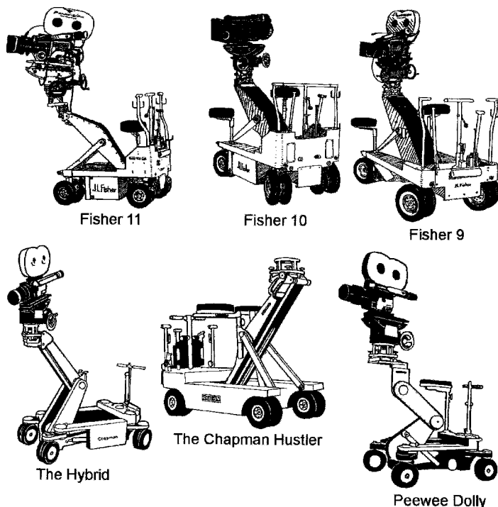
Figure 14.1 Various dollies from the J. L. Fisher Co. (top) and the Chapman Leonard Co. (bottom).
