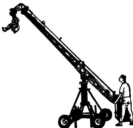
Figure 10.33b Pegasus Crane Remote (Panther).
