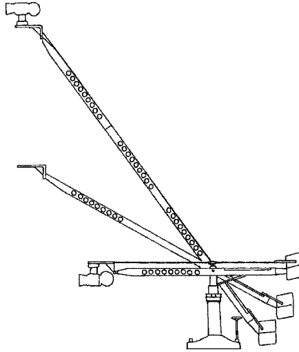
Figure 10.40b Enlouva Crane (Camera Support System, Inc.).
