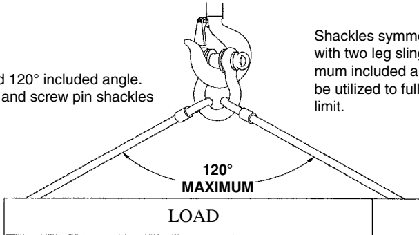
Figure 8.3e Shackles.
