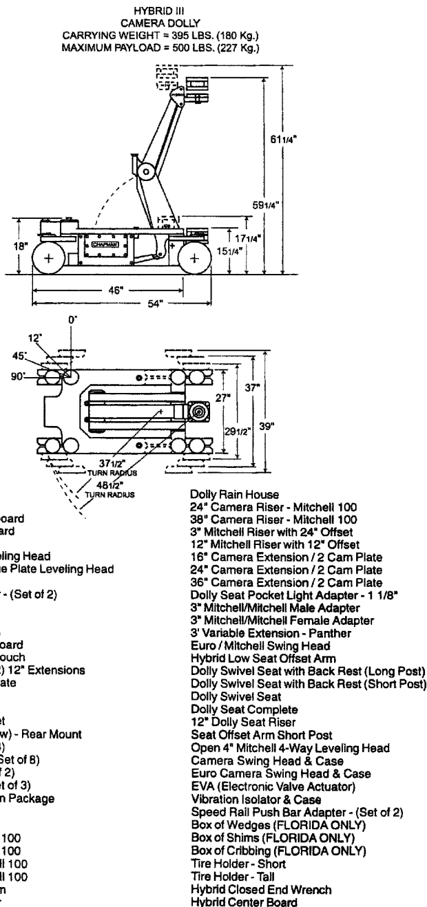
Figure 14.57 Hybrid III accessories.
