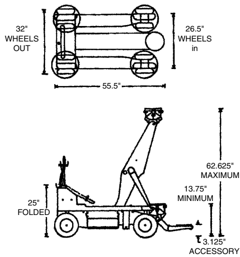
Figure 14.6b Fisher #10 crab dolly.
