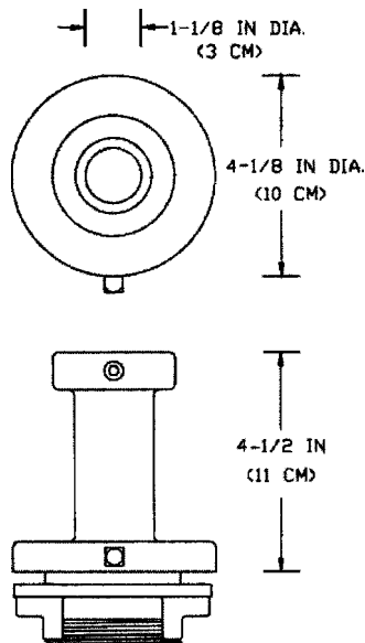
Figure 14.15 Adapter for 1-1/8" lamp pin.
