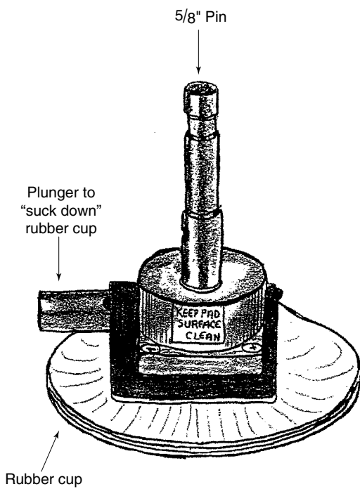
Figure 7.9 Small super grip.
