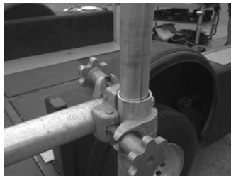
Figure 19.46 Slide the tubes inside the upright tubes. Now install a cross and secure it to the trailer by tying it down.
