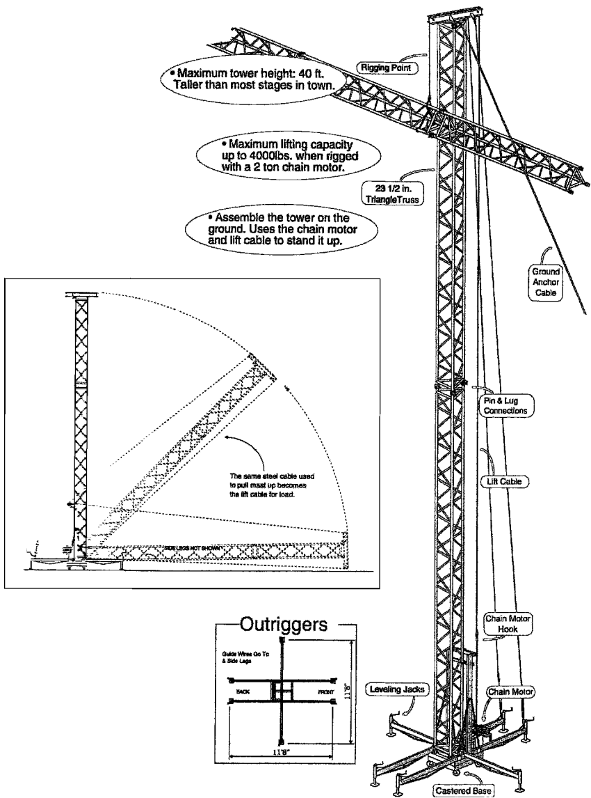
Figure 7.36 (Continued) ShowRig tower system.
