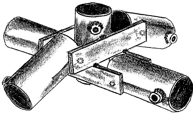
Figure 7.21 Four-way swivel coupler for Speed-Rail® (Modern Equipment Company).
