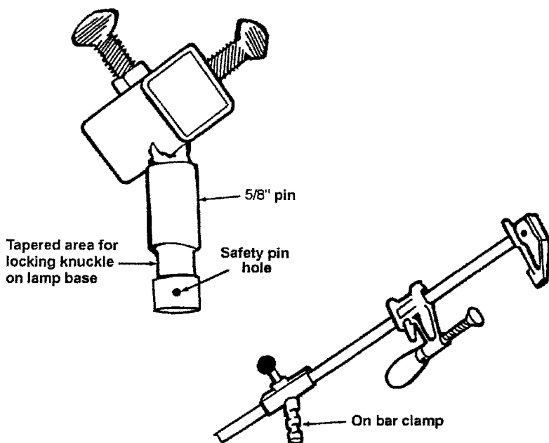
Figure 2.3 Bar clamp adapter pin.
