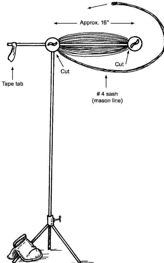
Figure 2.60g How to cut several lines the same length.
