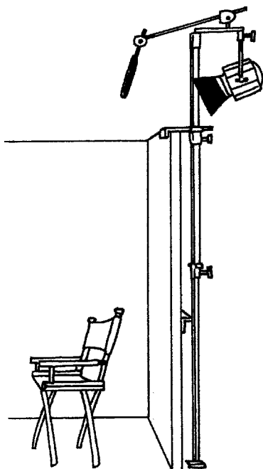
Figure 2.39a Lamppost system.
