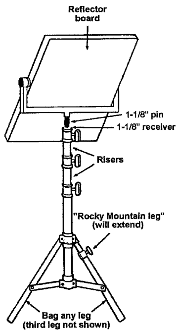
Figure 2.62a Reflector stand with Rocky Mountain leg.
