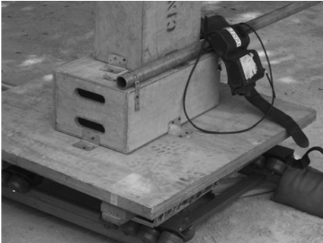
Figure 19.65 Makeshift dolly using channel wheels 4 × 4 plywood and apple boxes (adapting, making things work).
