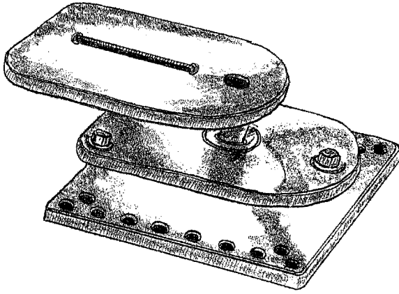
Figure 7.7 Ball level head.
