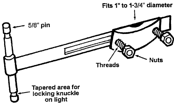
Figure 2.57 Side arm.
