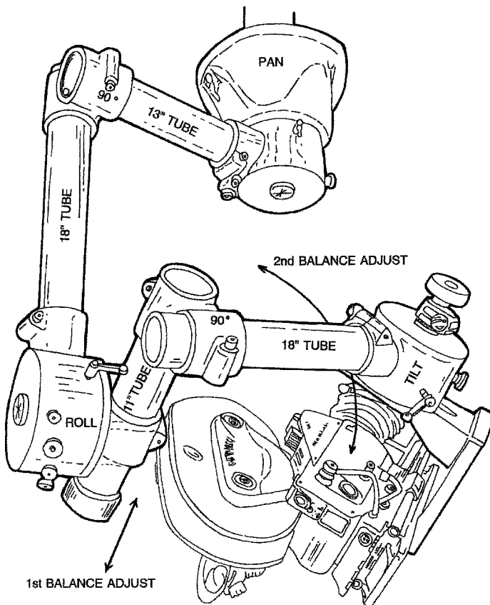
Figure 16.10b Weaver/Steadman Head.
