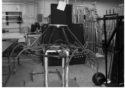
Figure 19.72 Spring-loaded Mitchell plate base (used to bounce camera during filming) for earthquakes/crashes (Modern Studio Equipment).
