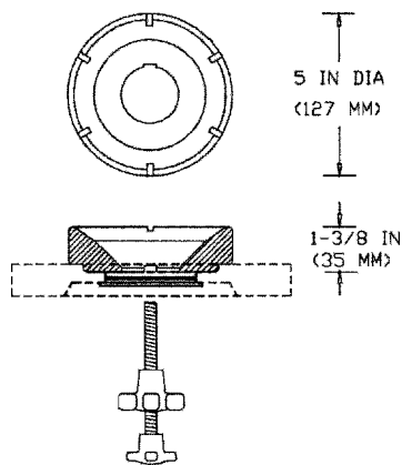
Figure 14.13 Ballmount adapter (a.k.a. Euro ball mount adapter).
