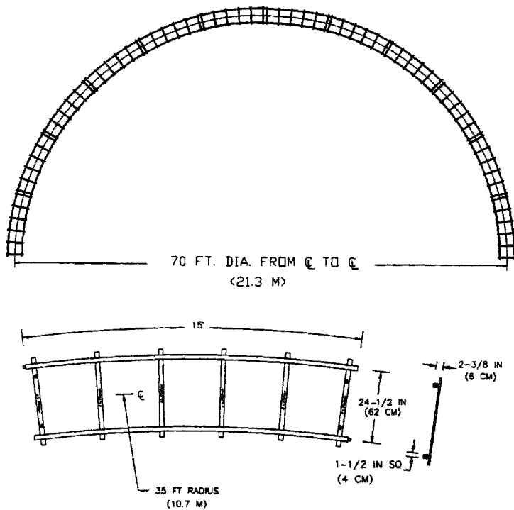
Figure 14.30 70 ft. diameter curved track (CS7) square tube.
