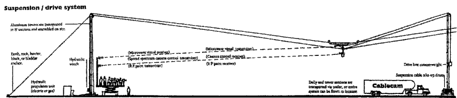
Figure 13.1a Cablecam over large area.
