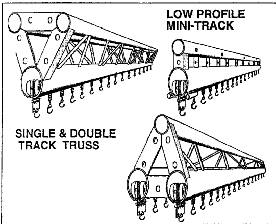
Figure 7.36 (Continued) ShowRig truss deck, platforms, green bead tower, and track chords systems.
