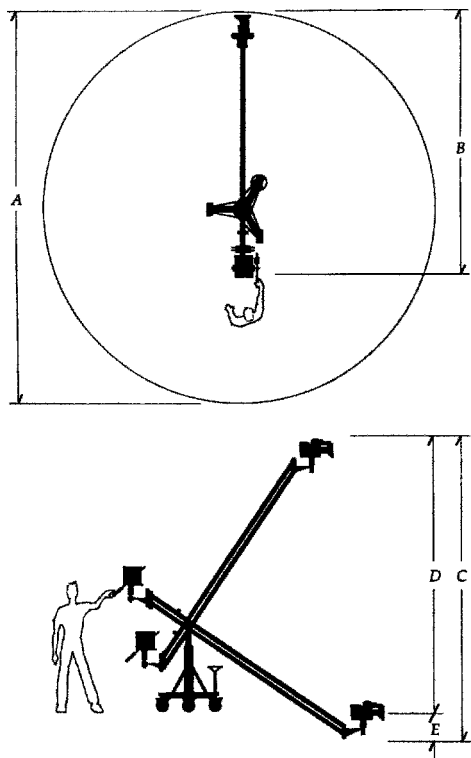
Figure 10.29b Barber Baby Boom.
