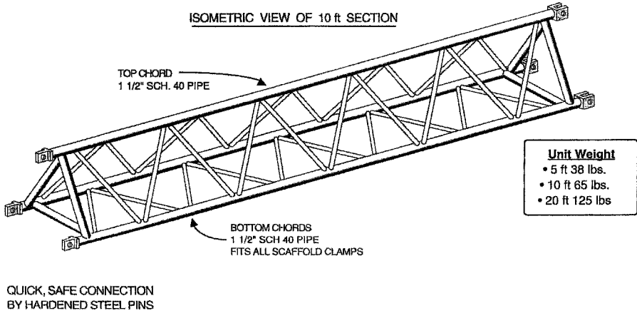
Figure 7.36 (Continued) ShowRig triangle truss.
