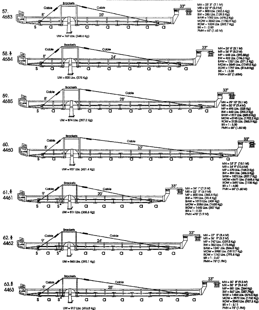
Figure 12.1 Lenny Cable Systems.
