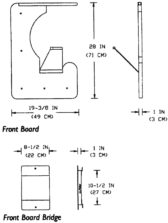
Figure 14.25 Front board and bridge.
