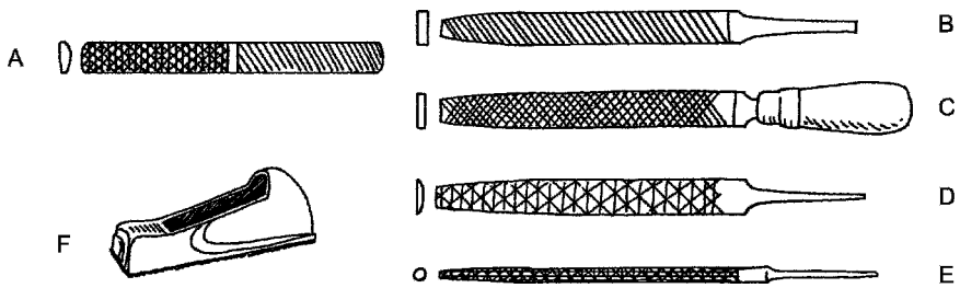
Figure 5.2 Files. A. Four in one, double/single (shown); rasp/half—round (not shown). B. Single. C. Double. D. Half round double crosscut. E. Rat tail. F. Hand rasp.
