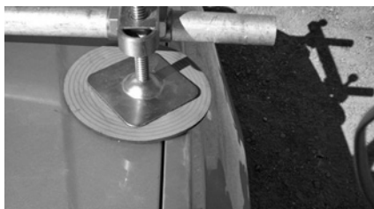
Figure 19.22 Hood mount foot pad (mouse pad).
