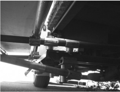
Figure 19.37 Rigging an auto/truck with speed rail™ and pinch clamps.
