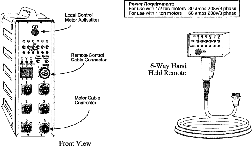
Figure 7.36 (Continued) ShowRig chain hoist and power distribution and hand-held remote systems.
