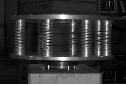
Figure 19.72 Spring-loaded Mitchell plate base (used to bounce camera during filming) for earthquakes/crashes (Modern Studio Equipment).
