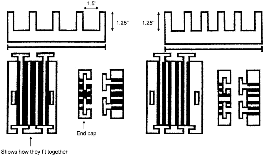
Figure 2.10 Cable crossovers.
