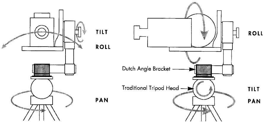
Figure 16.10a Weaver/Steadman Head.
