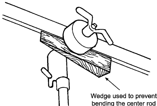
Figure 2.63b Overhead stand with a wedge.
