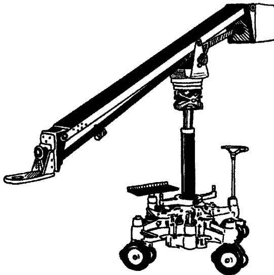
Figure 10.25c Fisher Jib/Arm, Model 21, on spider dolly.
