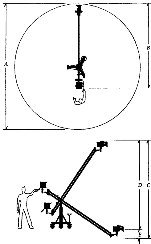
Figure 10.30d Barber Boom Travel.
