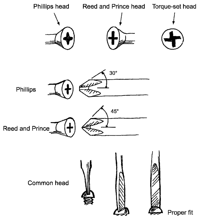
Figure 5.1b Screwdrivers.
