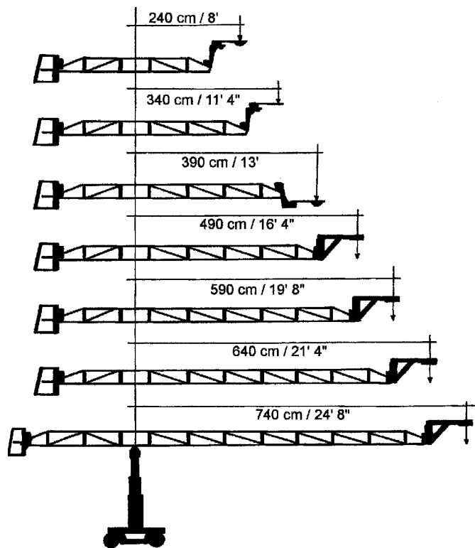
Figure 10.20b Javelin Crane Arm configurations (Egripment).
