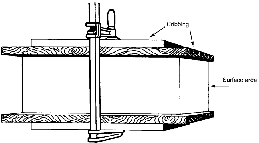
Figure 2.28a Furniture clamp with cribbing.
