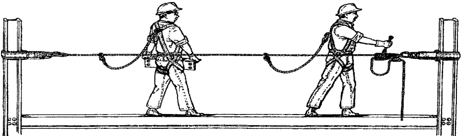
Figure 9.3d Body harness on cable.
