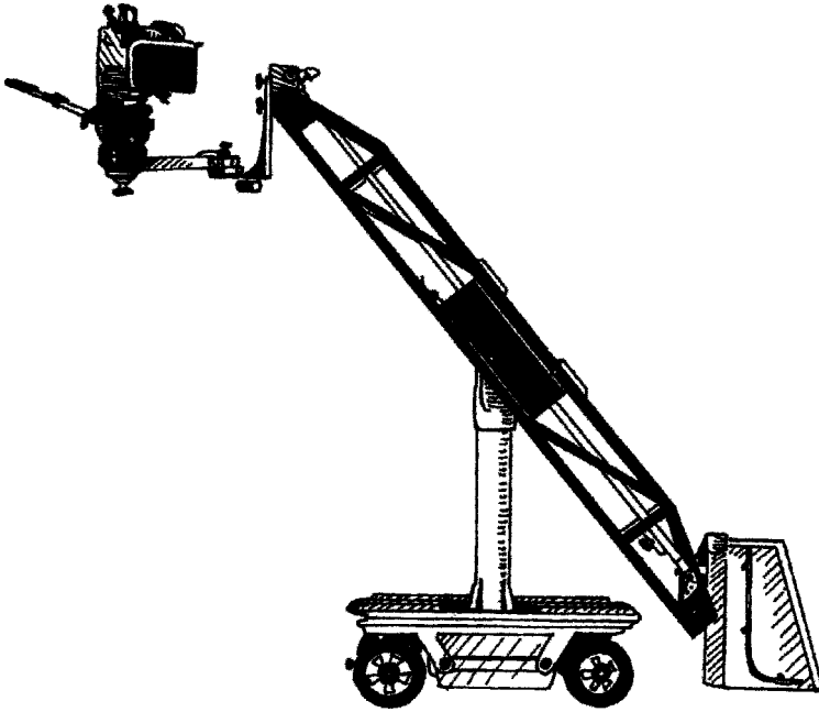
Figure 10.15a Maxi-Jib/Super Maxi-Jib (Egripment).
