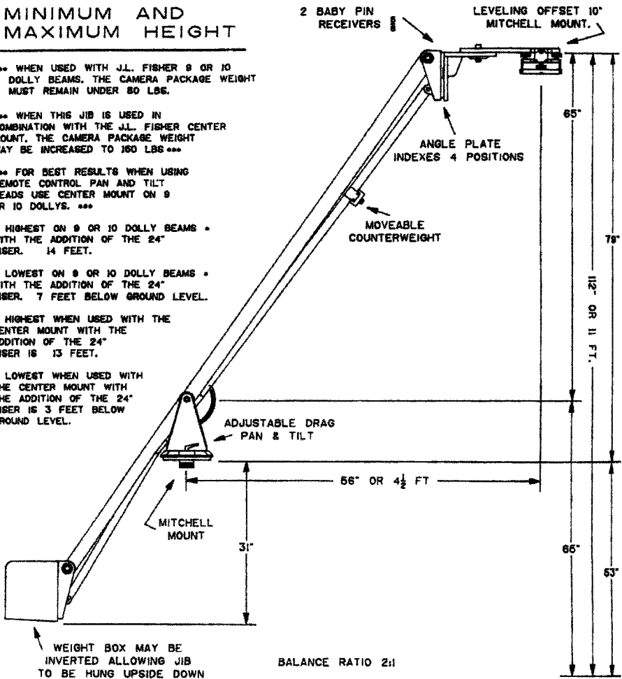
Figure 10.26a Fisher Jib/Arm, Model 22 (J. L. Fisher Mfg.).
