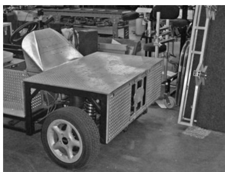
Figure 19.75 Cheese plate-covered “electric” (golf) cart (running/bicycle shots), very quiet (Modern Studio Equipment).
