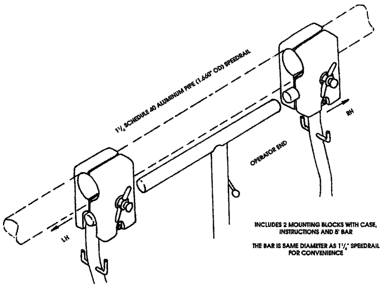
Figure 14.31 Push bar for #9, 10, and 11 dollies.
