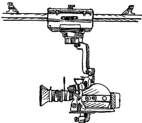
Figure 14.37 Filou track system (top mount/slung position).
