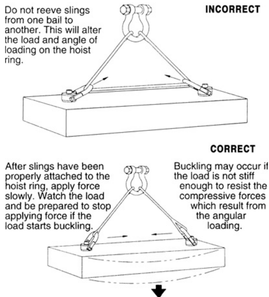
Figure 8.3d Correct and incorrect attached hoist ring.
