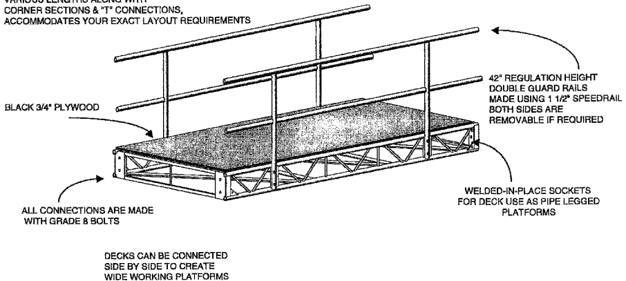
Figure 7.36 (Continued) ShowRig track chords and deck systems.
