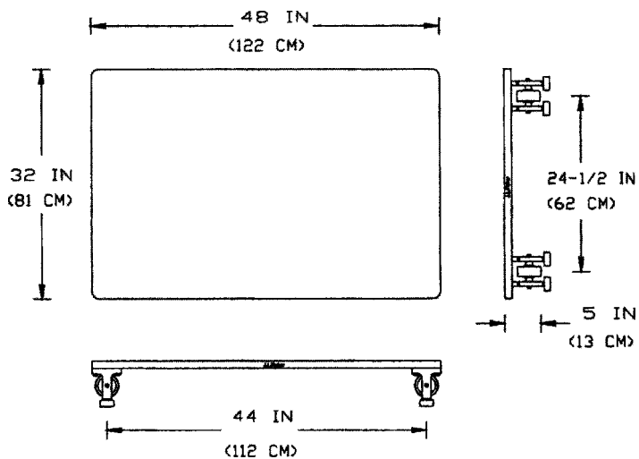
Figure 14.20 Scooter board (SCO).
