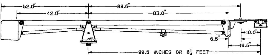
Figure 10.26b Fisher Jib/Arm, Model 22 (J. L. Fisher Mfg.).
