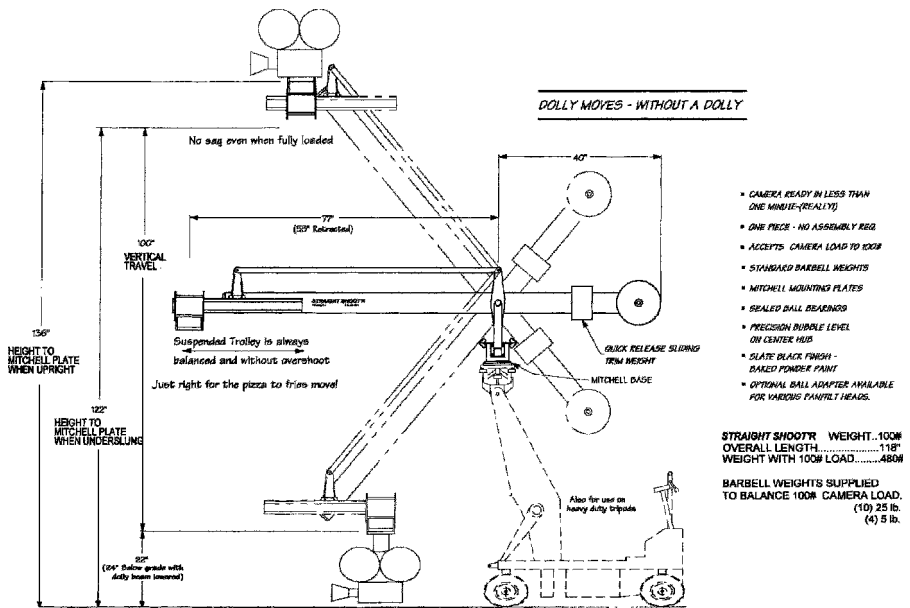
Figure 10.32b Straight Shoot'R.
