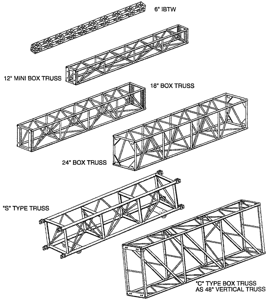
Figure 7.36 (Continued) ShowRig box trusses.
