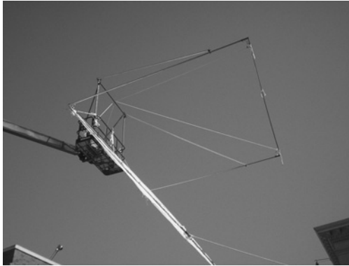
Figure 19.157a Fly swatter with flip down or side flip.
