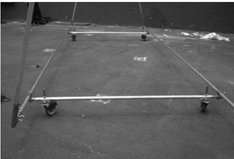
Figure 19.8 Rolling A-frame base built from speed rail, TM corners, 90-degree crosses, and casters/rollers.
