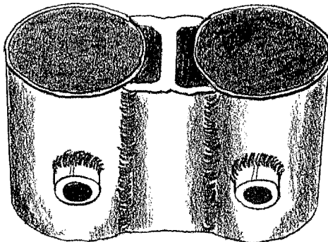
Figure 7.20 Speed-Rail® double coupler (Modern Equipment Company).
