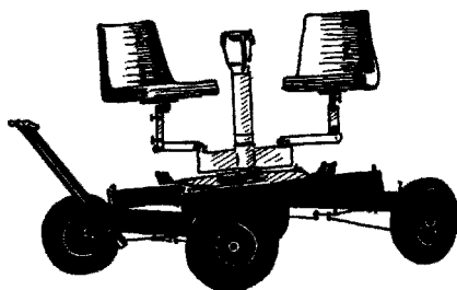
Figure 10.43b Giraffe Crane Base (Filmmär).
