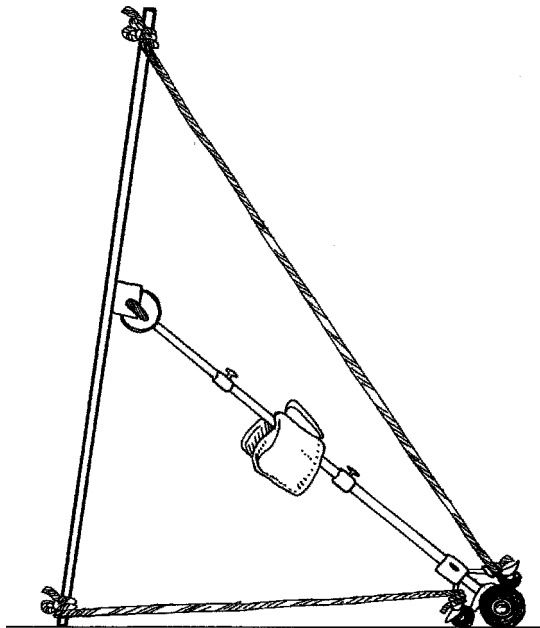
Figure 2.64b 12 ft. \times 12 ft. overhead set for wind conditions.
