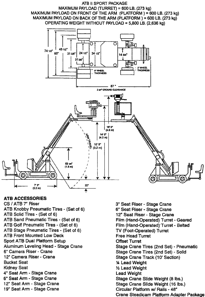
Figure 10.51 ATB II Sport Package.
