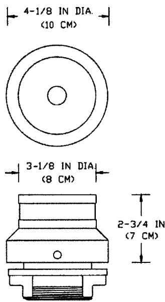
Figure 14.16 Adapter for spider head.
