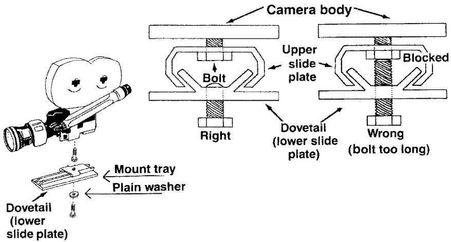
Figure 7.4 Dovetail method.
