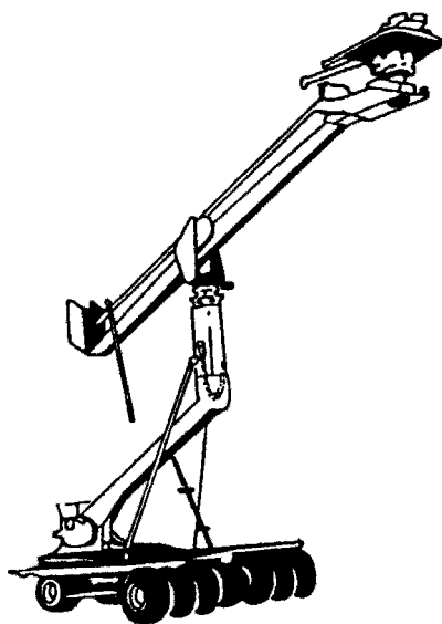
Figure 10.27b Chapman Crane Arm on Chapman Olympian (Chapman/Leonard).
