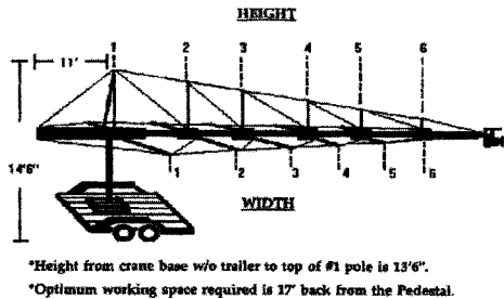
Figure 10.45d The Akela Crane.
