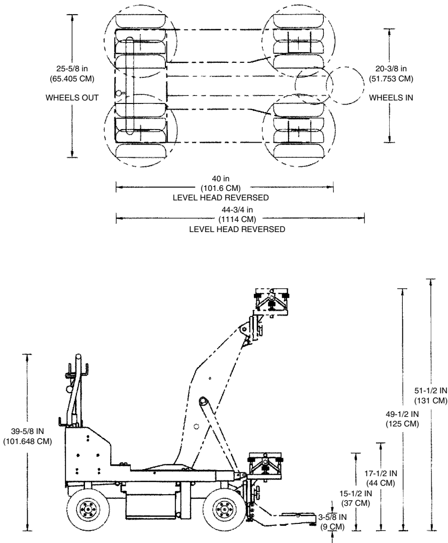
Figure 14.5b Fisher #11 crab dolly.
