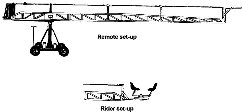
Figure 10.34a V.I.P. Four-in-one Crane.
