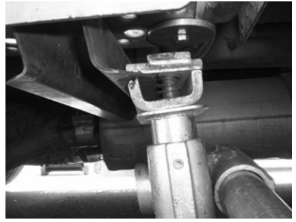
Figure 19.37 Rigging an auto/truck with speed rail™ and pinch clamps.
