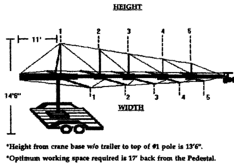
Figure 10.45c The Akela Crane.
