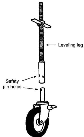
Figure 2.48b Parallel screw jack.
