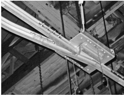
Figure 19.107 Curtain/backing switcher.
