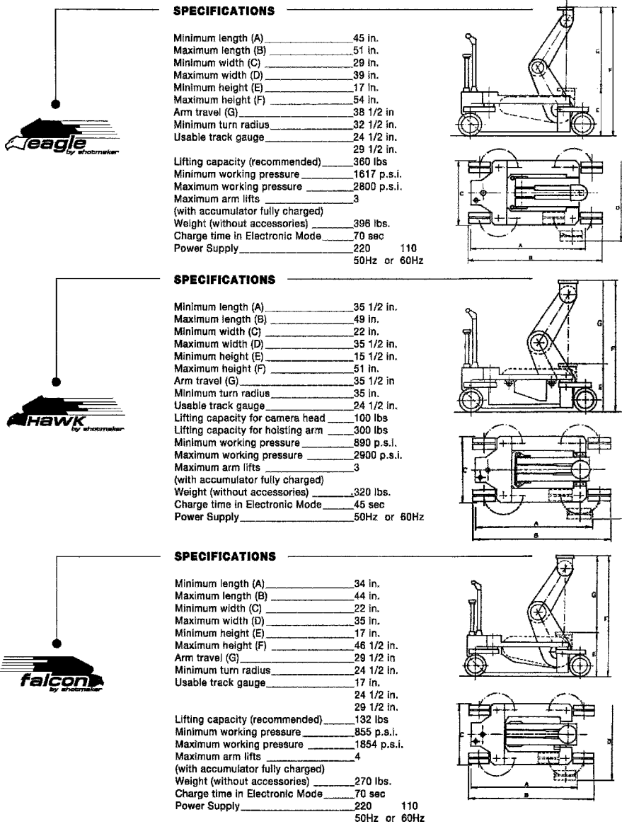
Figure 14.32 Shotmaker Blue specifications.
