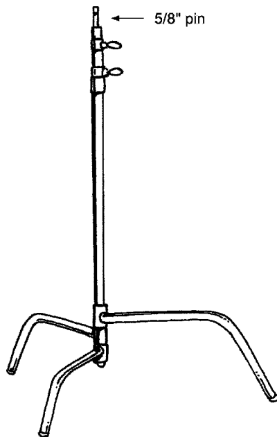
Figure 2.60a C-stand without a head or arm.
