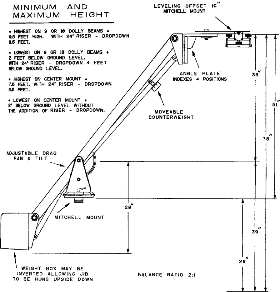
Figure 10.25a Fisher Jib/Arm, Model 21 (J. L. Fisher Mfg.).
