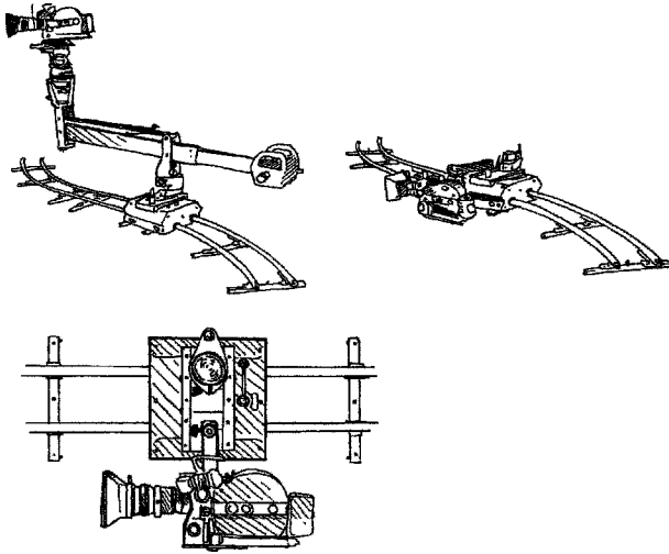
Figure 14.38 Filou track system (bottom/underslung and side-mount positions).
