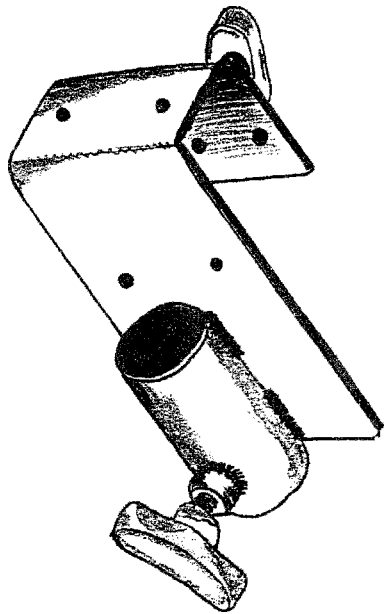
Figure 7.21 Four-way swivel coupler for Speed-Rail® (Modern Equipment Company).
