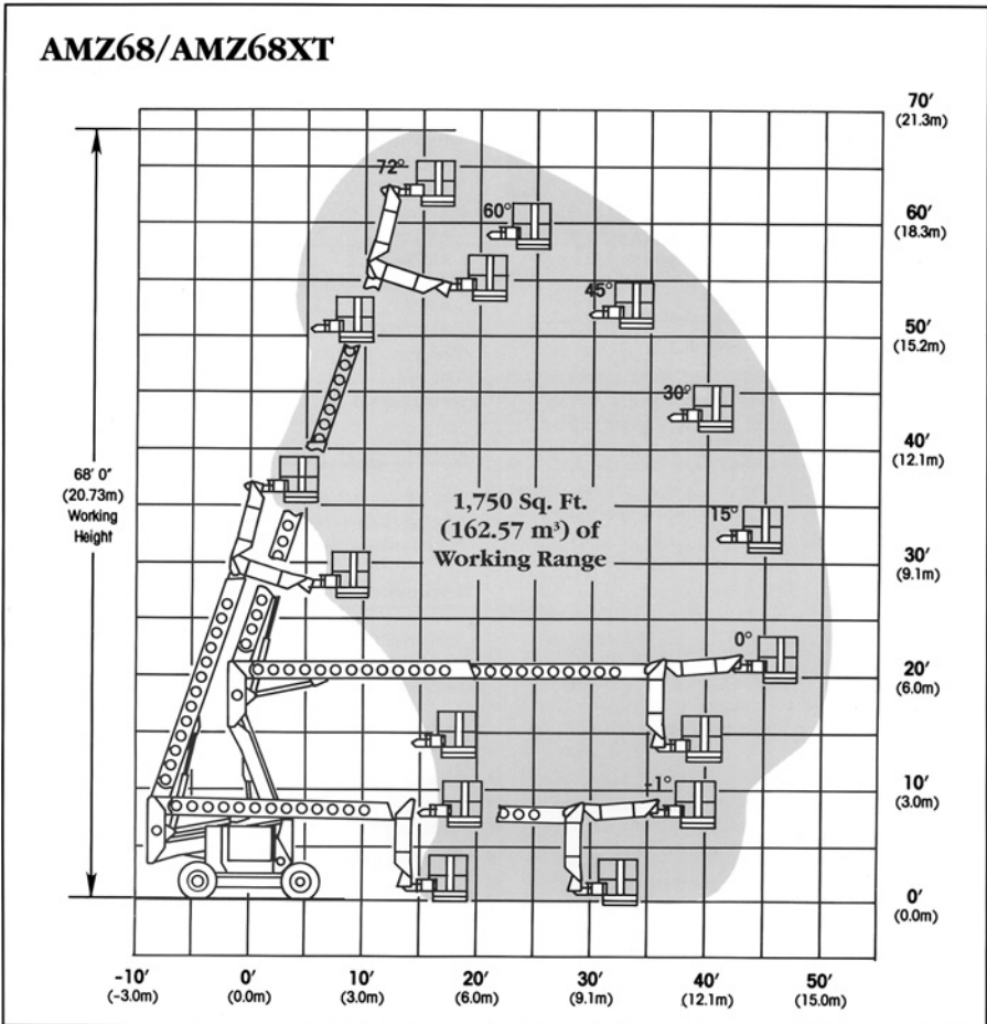
Figure 9.1 Condor with articulating arm.
