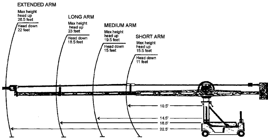
Figure 10.31c MC-88 Crane specs (Matthews).
