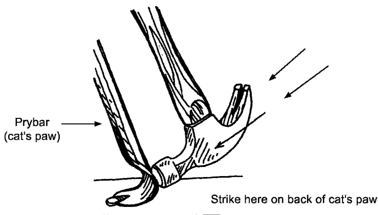
Figure 5.9 Claw hammer.
