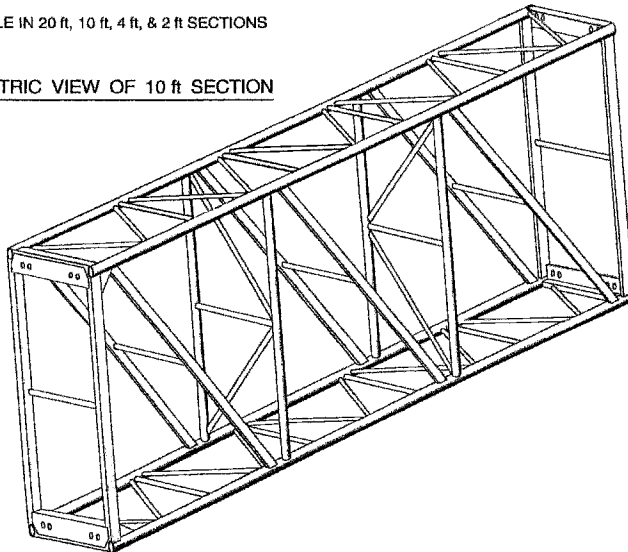
Figure 7.36 (Continued) ShowRig box trusses.
