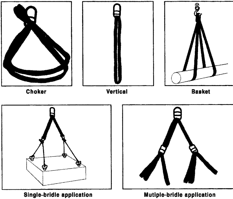
Figure 8.3c Bridle slings.
