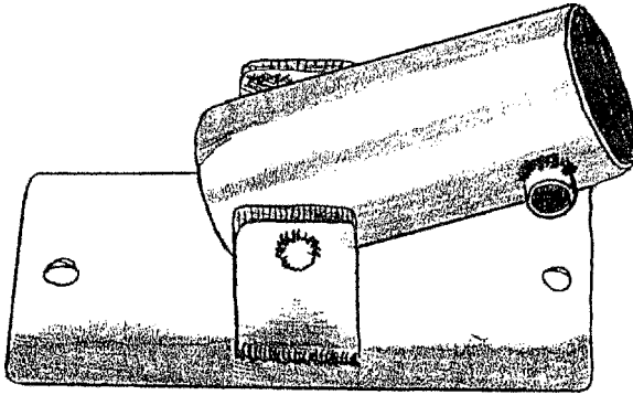
Figure 7.18 Speed-Rail® swivel flange (Modern Equipment Company).
