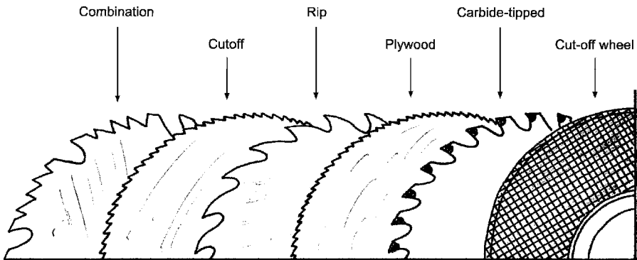
Figure 5.6 Circular saw blades.
