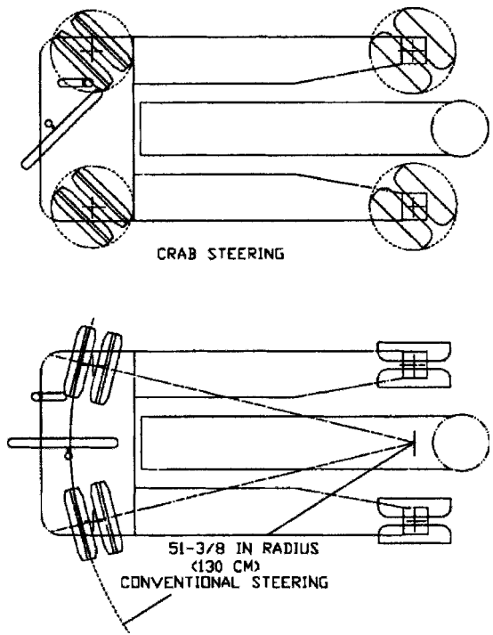
Figure 14.6c Fisher #10 crab dolly.
