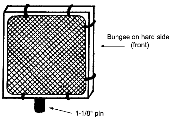
Figure 2.54d Attaching slip-ons.
