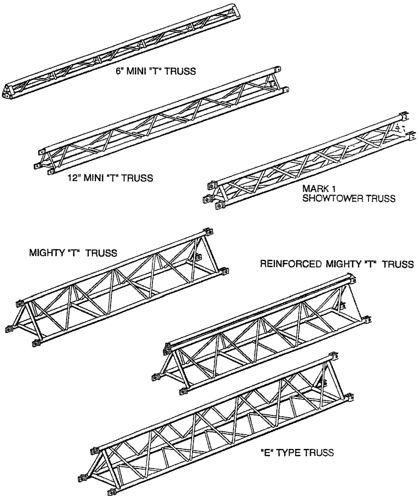
Figure 7.36 Triangle trusses.
