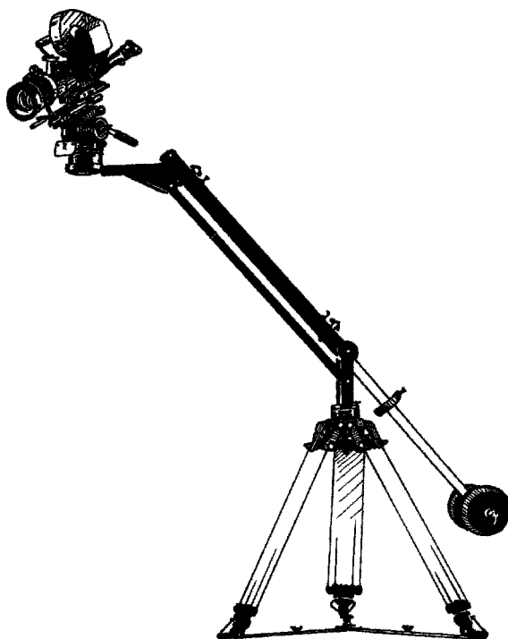
Figure 10.10a Porta Jib on tripod.
