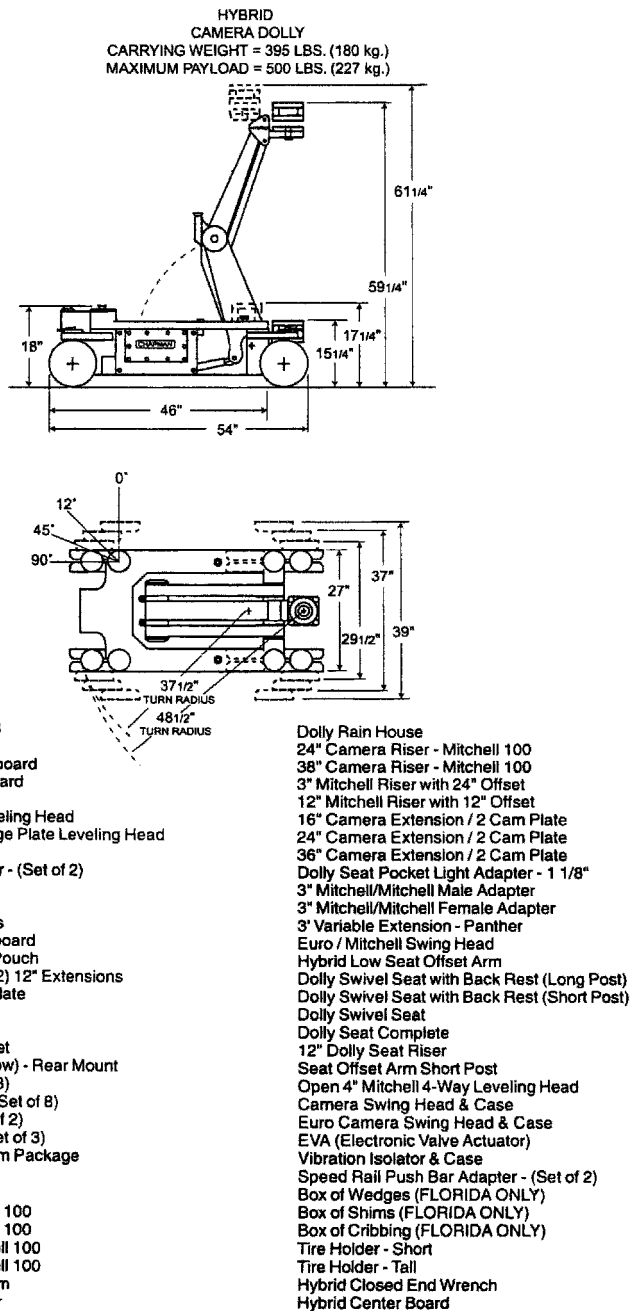
Figure 14.55 Hybrid accessories.
