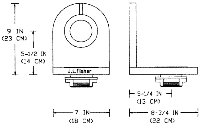
Figure 14.8 90-degree angle plates.
