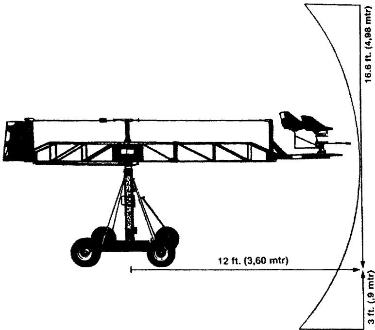
Figure 10.42b The Crane.
