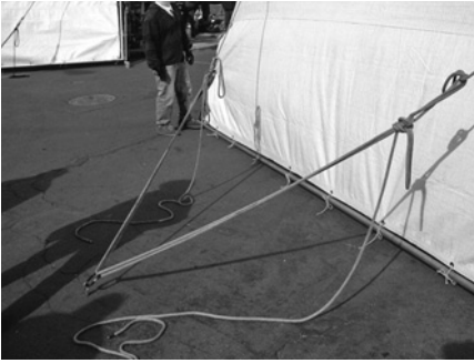
Figure 19.143 The “P-Ton” at work.
