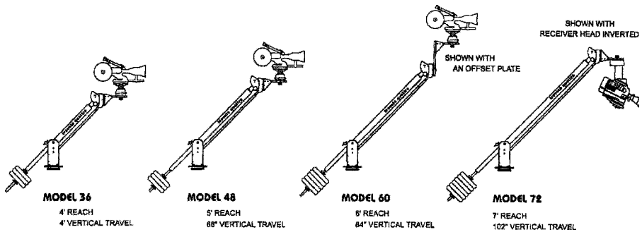
Figure 10.6 Trovato Tote Jib (Trovato Manufacturing, Inc.).
