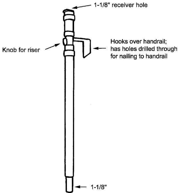
Figure 2.5 Bazooka for perms and green beds.
