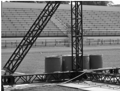
Figure 19.16 Water-filled drums to act as “weight” against the wind.
