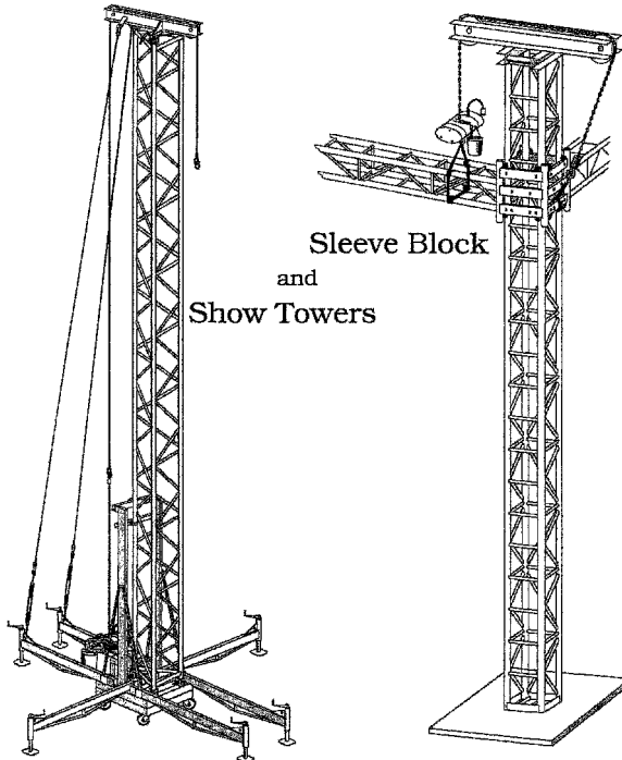
Figure 7.36 (Continued) ShowRig truss tower system.
