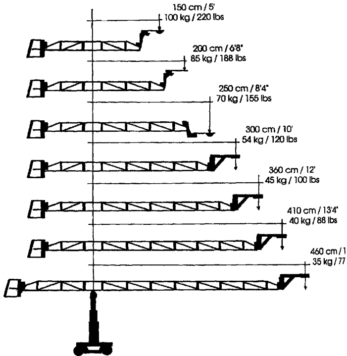
Figure 10.15c Maxi-Jib configurations.
