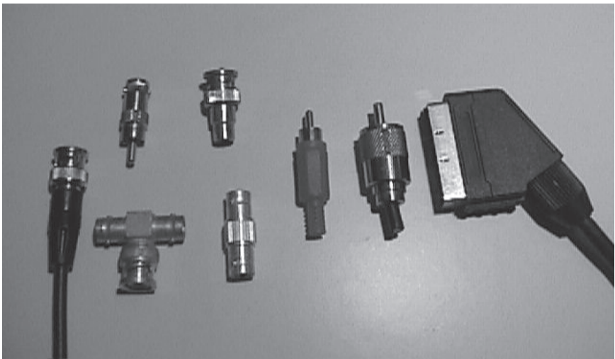
Figure 2.22 Range of connectors. From left to right: BNC crimp, BNC T coupler, BNC straight coupler, two variations of BNC/phono adapter (top), Phono, UHF, SCART
