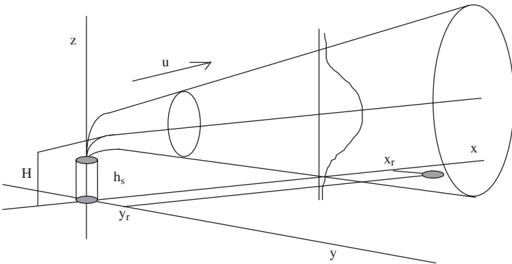
Fig. 1. Gaussian Plume Model.
