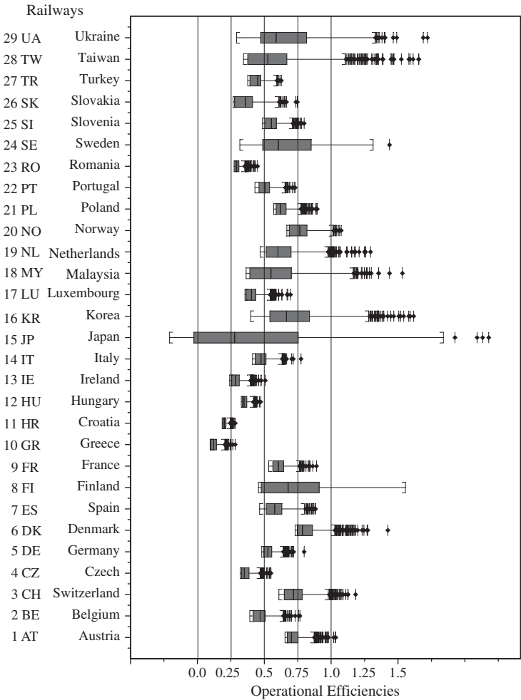
Fig. 3. Box Plots of Railway Operational Efficiencies.
