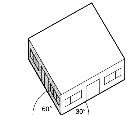
Figure 1.8 An axonometric projection, to give more of a bird's eye view of the proposed building
