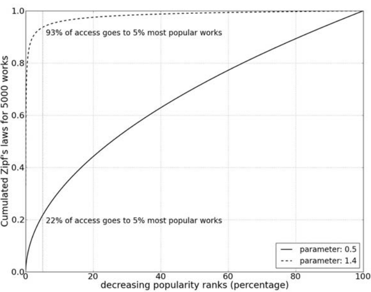
Fig. 3.3. Cumulated attention for extreme observed cases
