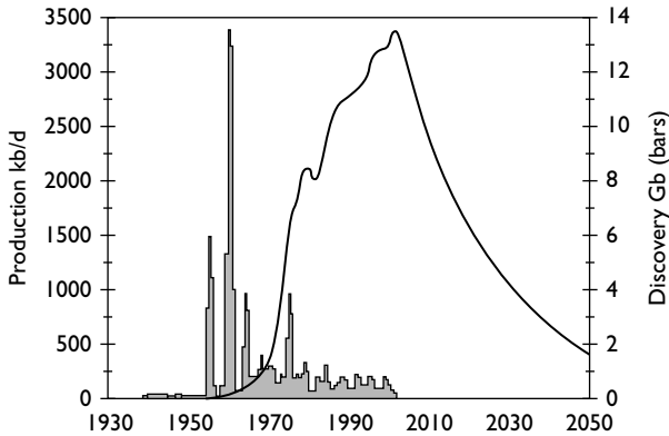
Figure 4.12 Chinese production
