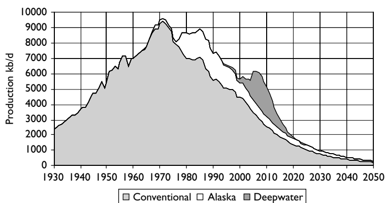
Figure 4.8 US production
