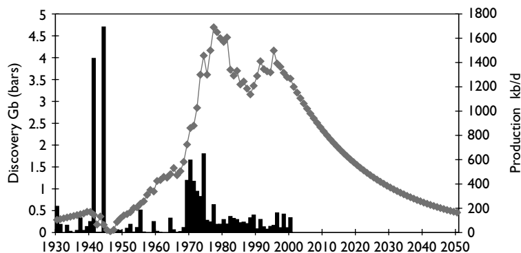
Figure 4.11 Indonesian production
