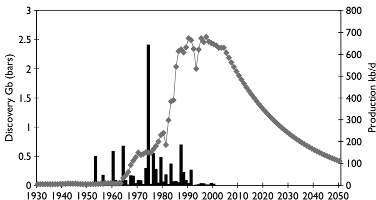
Figure 4.10 Indian production
