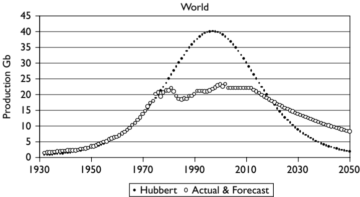
Figure 4.6 Hubbert curve
