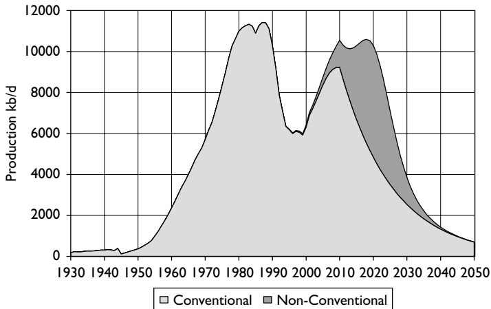
Figure 4.9 Russian production
