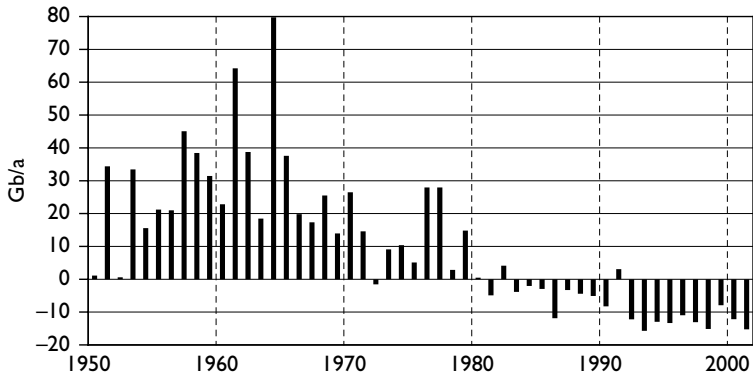
Figure 4.2 Discovery-consumption gap
