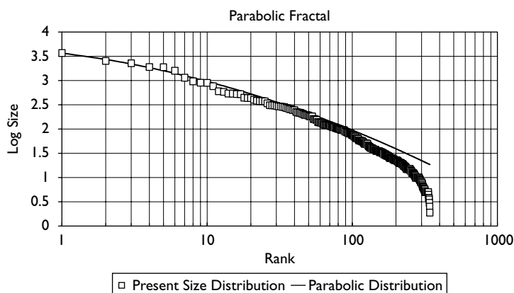
Figure 4.5 Parabolic fractal
