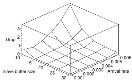
(c) Exterior piconet, K = 1 .
