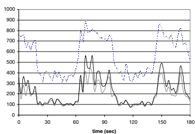
(a) Local delay under varying piconet load.
