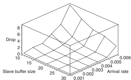
(b) Interior piconet, K = 0 .
