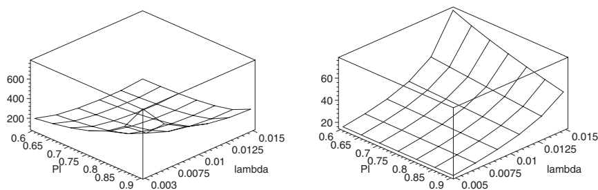
(a) Loci of T_1 values that minimize the delay for local traffic. (b) Loci of T_1 values that minimize the delay for non-local traffic.
