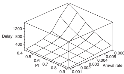
(a) Exterior piconets, M_s = 2 .
