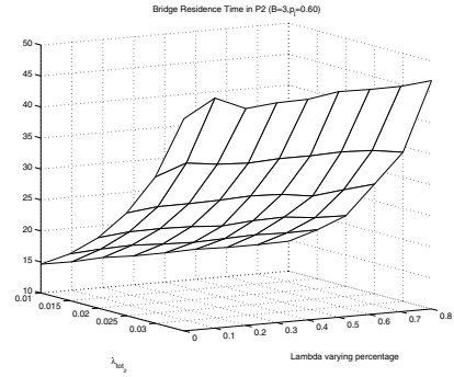
(b) Mean bridge residence time for piconet 2 when P_l = 0.6 in P1 and P3, asymmetric slave load.
