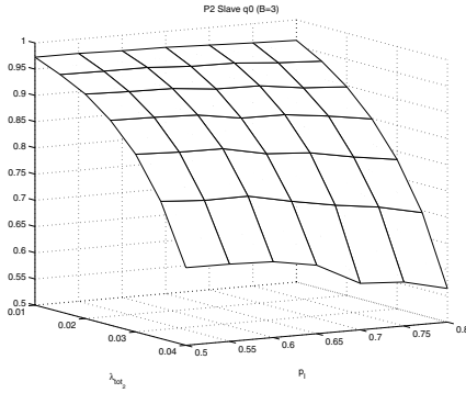
(a) q_0^i/Q_i(1, 1) for the slave in piconet 2 when \lambda_{tot} and P_l are varying.
