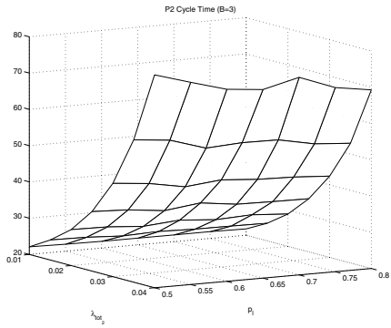
(d) Mean cycle time for piconet 2 as a function of P_l , symmetric slave load.
