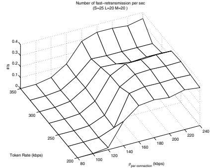
(f) Fast retransmission rate.
