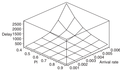
(e) Exterior piconets, M_s = 8 .
