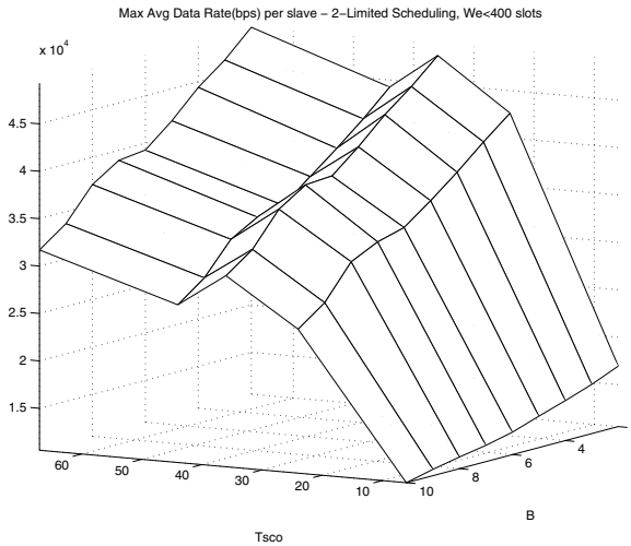
(b) Maximum achievable data rates (simulation results).
