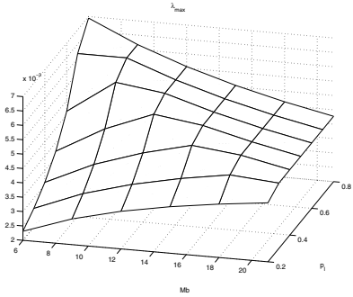
(b) Maximum packet burst arrival rate, \lambda_{max} , that does not lead to instability.
