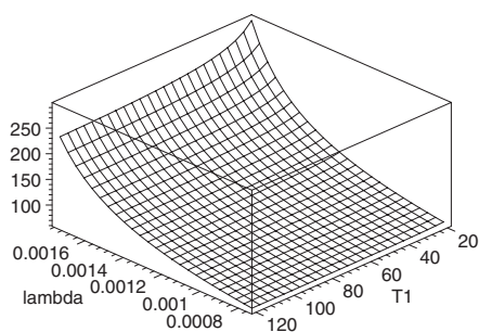
(b) Exhaustive polling, analytical solutions.
