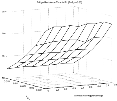
(a) Mean bridge residence time for piconet 1 when P_l = 0.6 in P1 and P3, asymmetric slave load.
