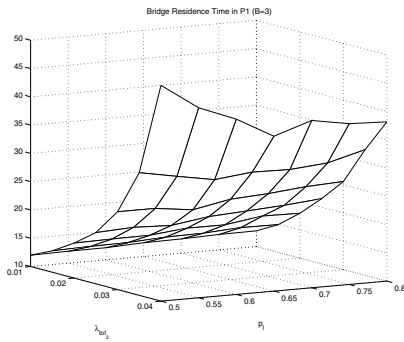
(c) Mean bridge residence time for piconet 1 as a function of P_l , symmetric slave load.
