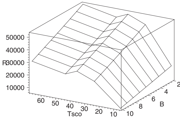
(a) Maximum achievable data rates (analytical solutions).
