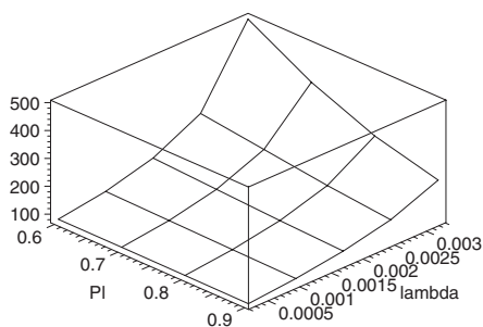
(a) End-to-end delay for local traffic.
