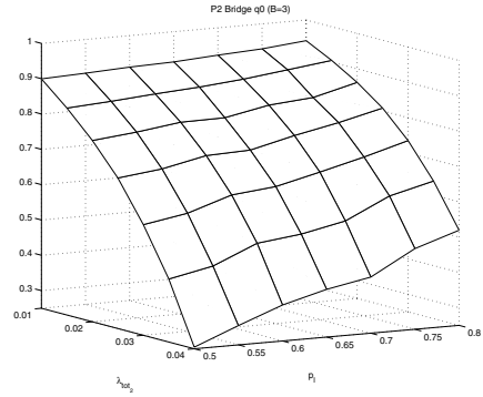
(b) q_0^i/Q_i(1, 1) for the bridge in piconet 2 when \lambda_{tot} and P_l are varying.
