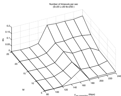
(e) Time-out rate.
