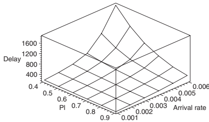
(c) Exterior piconets, M_s = 5 .
