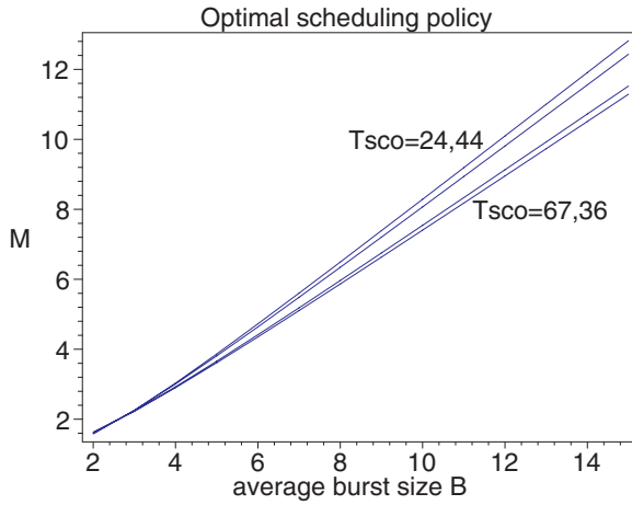
FIGURE 7.4 Optimal value of M as a function of the mean burst size \bar{B} . (From J. Mišić, V. B. Mišić, and K. L. Chan, “Talk and let talk: performance of Bluetooth piconets with synchronous traffic,” Ad hoc networks , 3 (4):451–477, © 2003 Elsevier B. V.)
