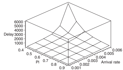
(f) Interior piconets, M_s = 8 .
