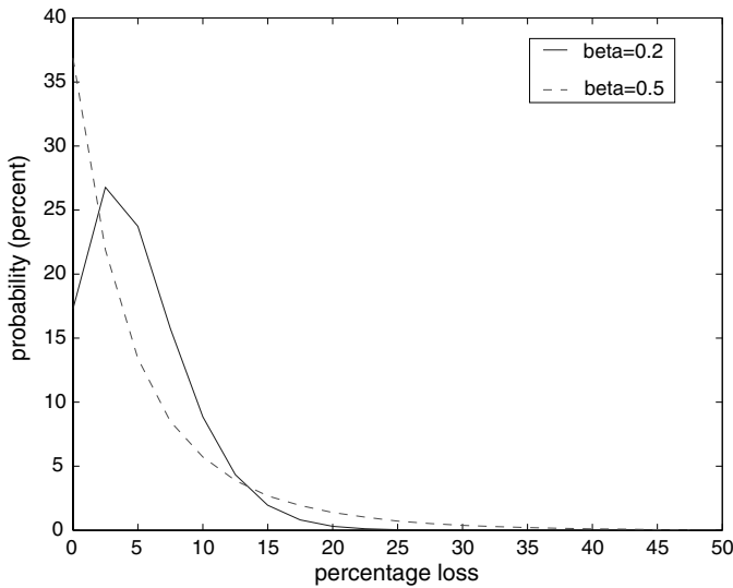
FIGURE 19.6. Unconditional Loss Distribution Functions for Smaller Portfolios (based on 500,000 simulations of the model)
