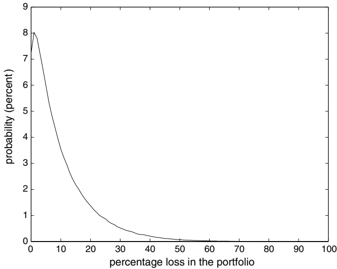
FIGURE 21.1. Loss Distribution Function for a Portfolio with 100 Assets (one-year horizon)
