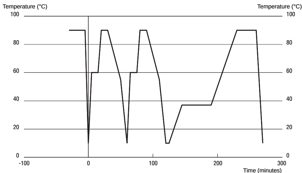
Figure 2. Process diagram
