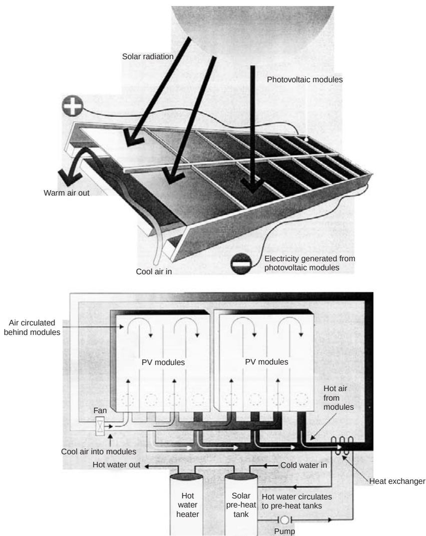
Figure 7.5 Diagrams of PV heat recovery system (courtesy of CADDET)
