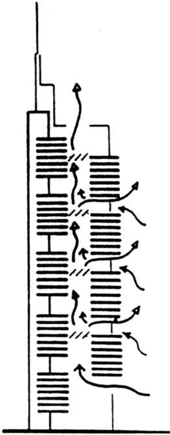
Figure 12.18 Natural ventilation paths in the Commerzbank
