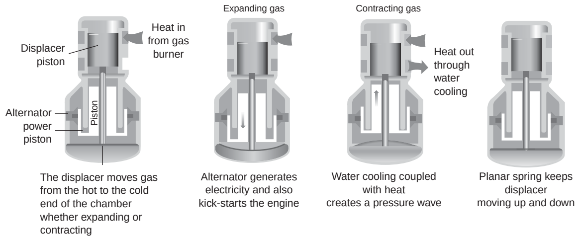
Figure 7.6 Four phases of the Stirling engine cycle
