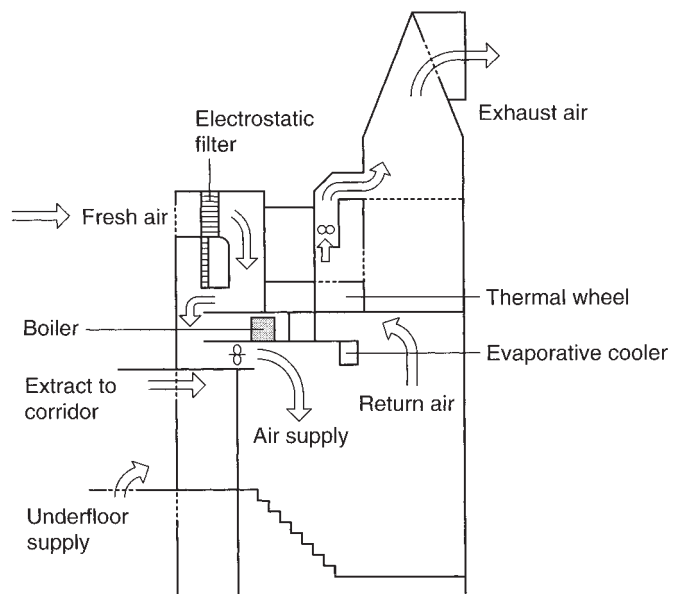
Figure 12.10 Air handling units (AHUs) Jubilee Campus
