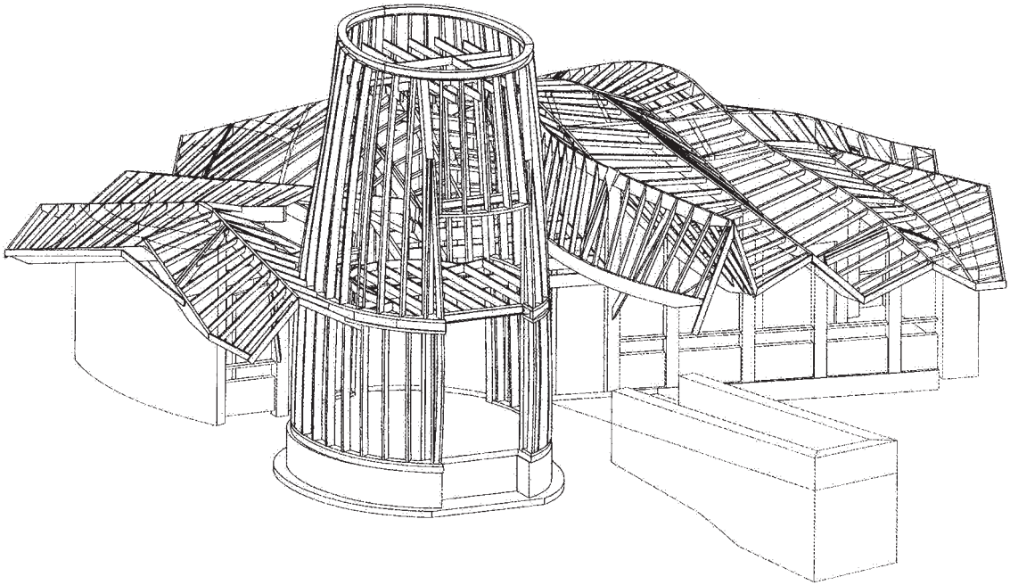
Figure 8.9 Roof formation, the Maggie Centre, Dundee (courtesy of RIBA Journal)
