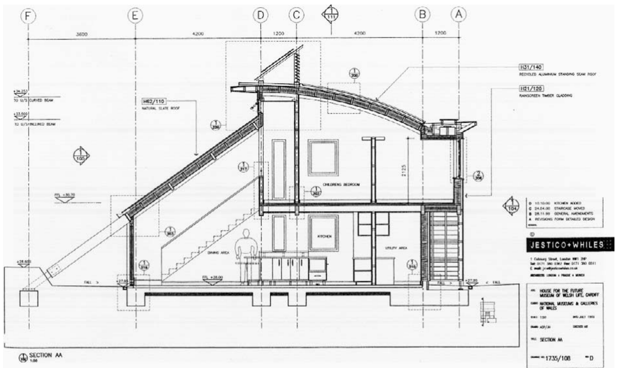
Figure 8.4 House for the Future – cross-section
