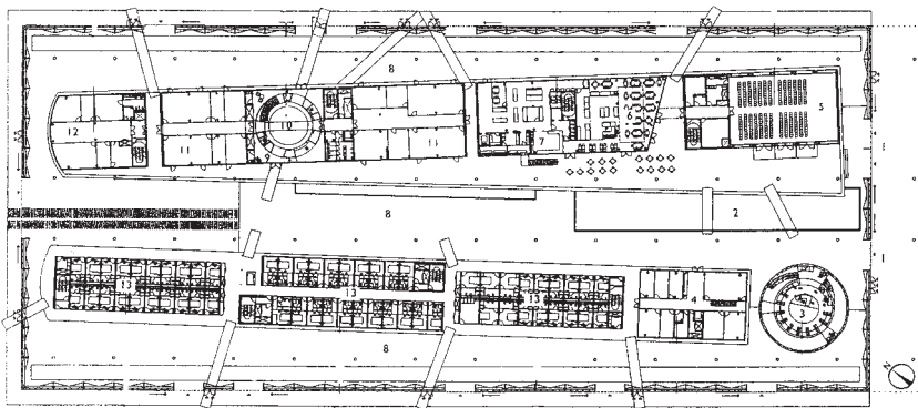
Figure 11.7 Mount Cenis ground floor plan
