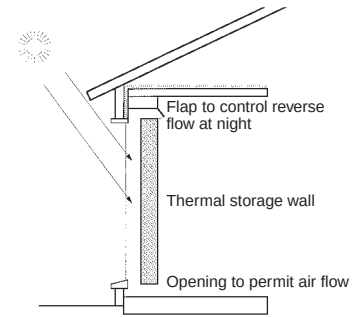
Figure 5.5 Indirect solar – Trombe wall
