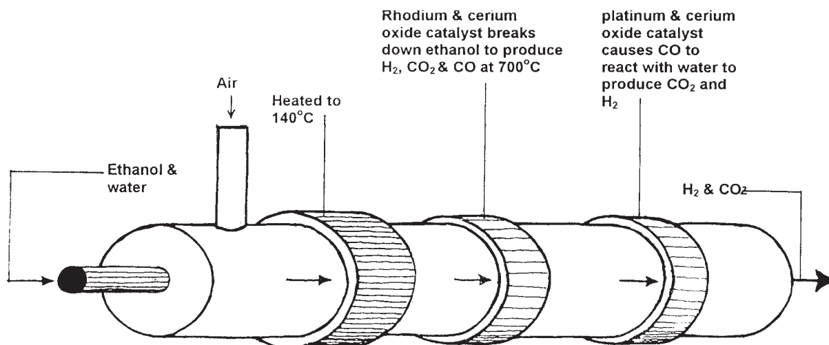
Figure 21.2 Compact fuel cell hydrogen generator (courtesy of New Scientist )
