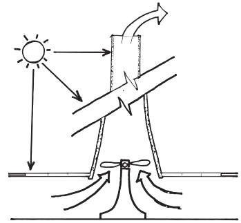
Figure 4.1 Solar chimney generator
