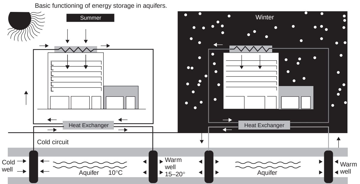
Figure 13.7 Principles of seasonal storage (courtesy of CADDET)
