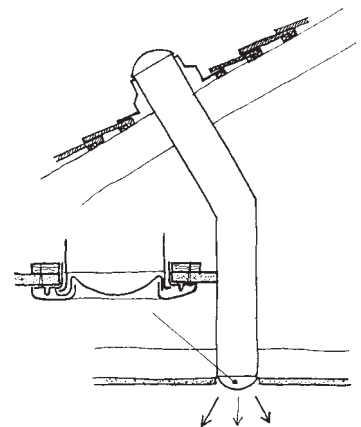
Figure 14.4 Section through a sunpipe
