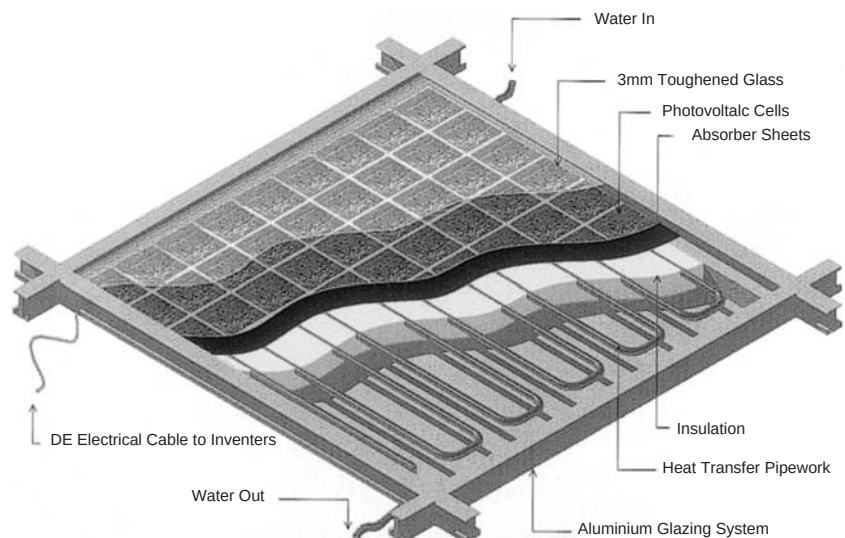
Figure 18.16 PV/thermal panels (Courtesy of Studio E Architects)
