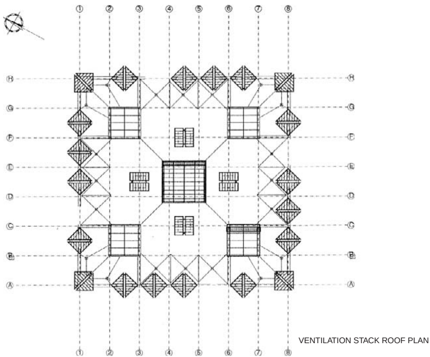
Figure 12.3 Plans, Coventry University library
