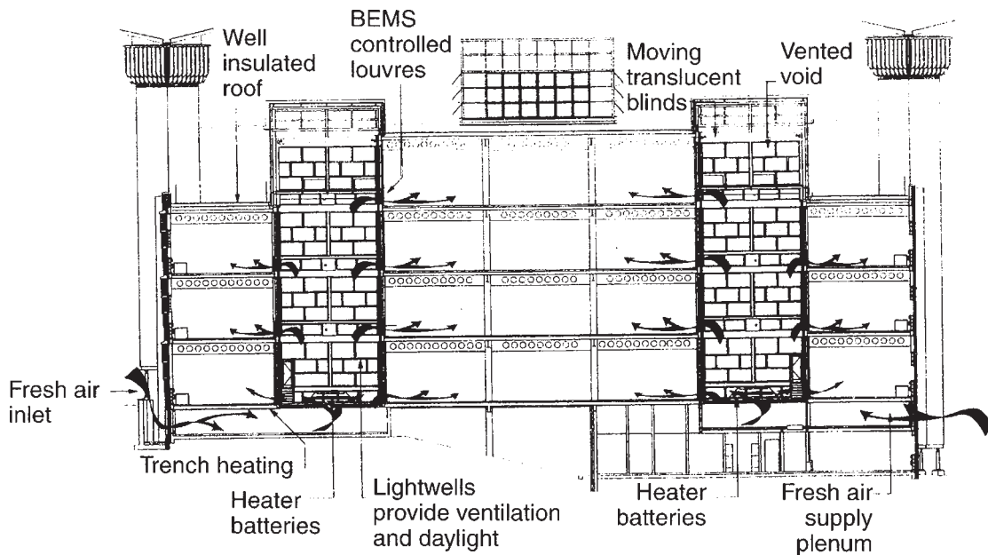
Figure 12.4 Air circulation paths
