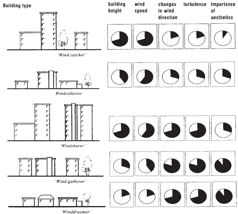
Figure 9.2 Categories of building cluster and their effectiveness for wind generation (courtesy of Ecofys and REW)
