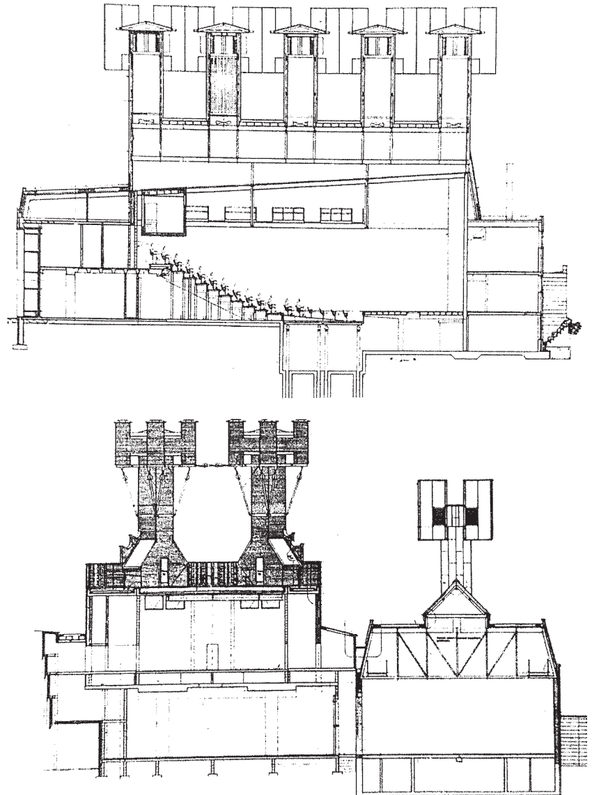
Figure 12.6 Longitudinal and transverse sections, Contact Theatre
