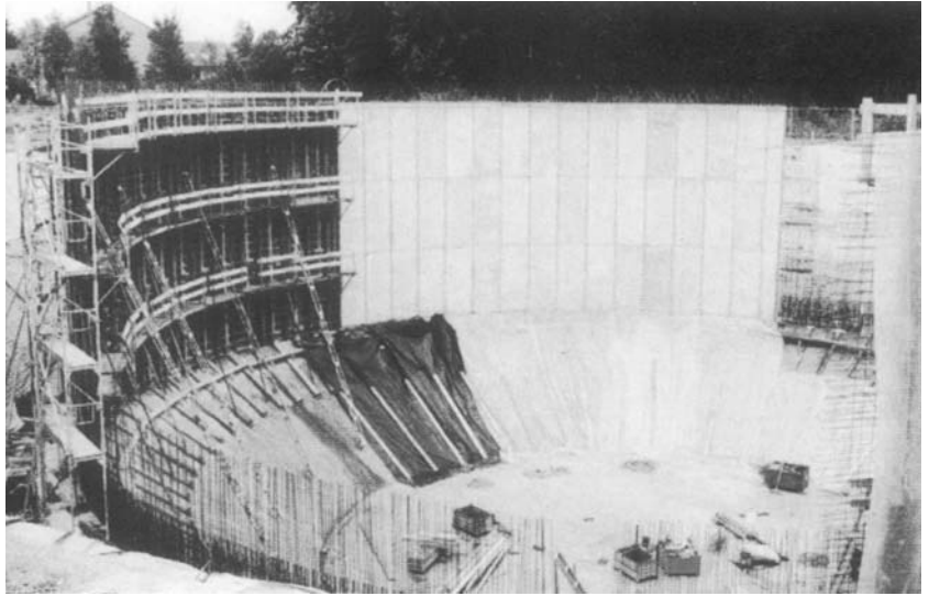
Figure 5.9 Seasonal storage tank under construction, Friedrichshafen (courtesy of REW)
