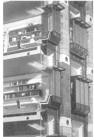
Figure 11.3 Portcullis House; cutaway section of facade
