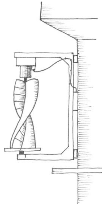
Figure 9.1 Helical side mounted turbine on oil platform
