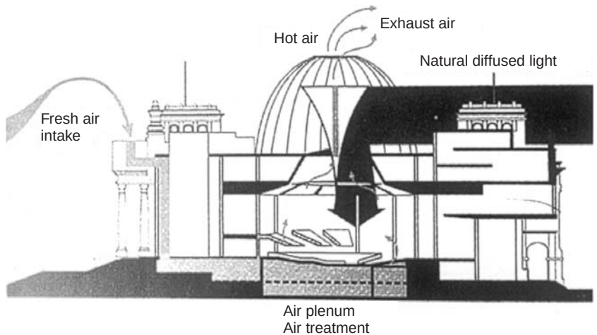
Figure 12.14 Displacement ventilation and natural light in the Reichstag
