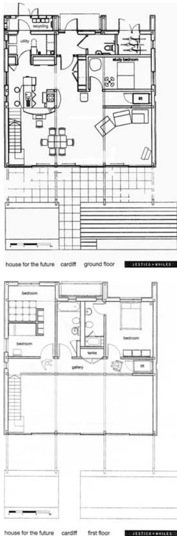
Figure 8.6 Ground and first floor
