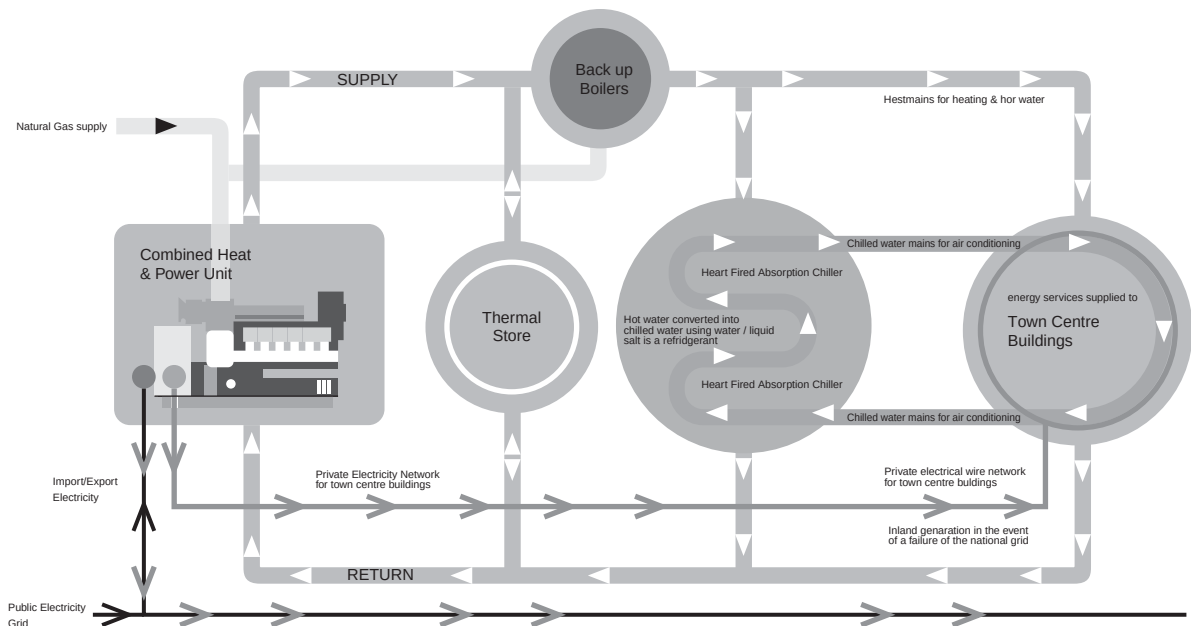
Figure 19.2 Combined heat, cooling and power grid, Woking town centre
