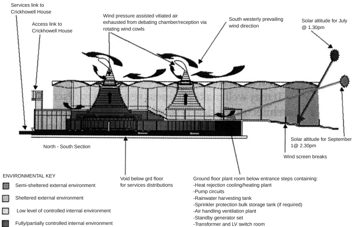
Figure 18.2 Welsh Assembly natural light and ventilation diagrams
