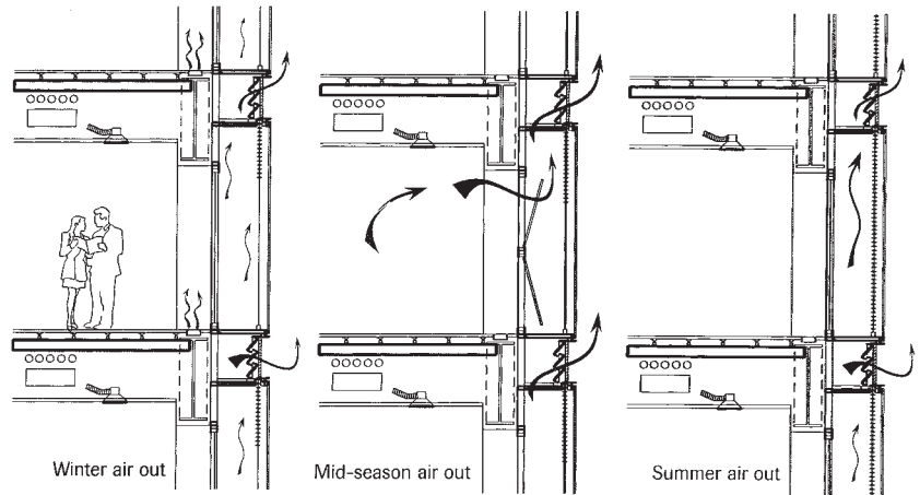
Figure 12.23 Natural ventilation in a climate facade, Minerva 2
