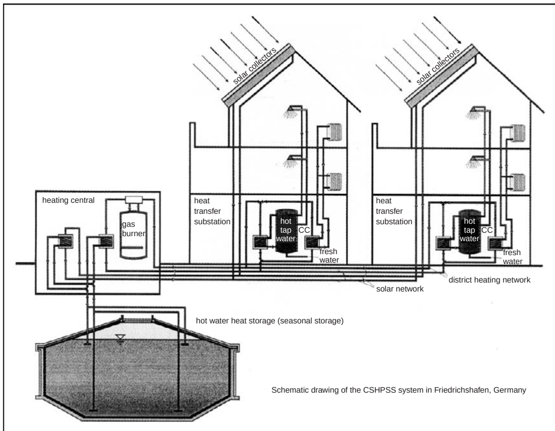
Figure 5.8 Diagram of CSHPSS system, Friedrichshafen (courtesy of Renewable Energy World (REW))
