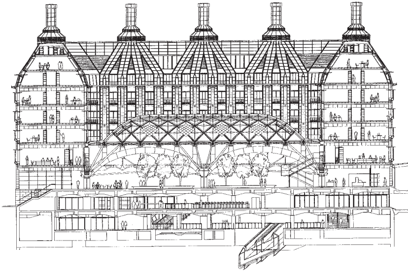
Figure 12.11 Portcullis House, section
