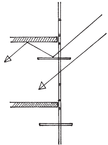
Figure 14.3 Basic principle of the light shelf
