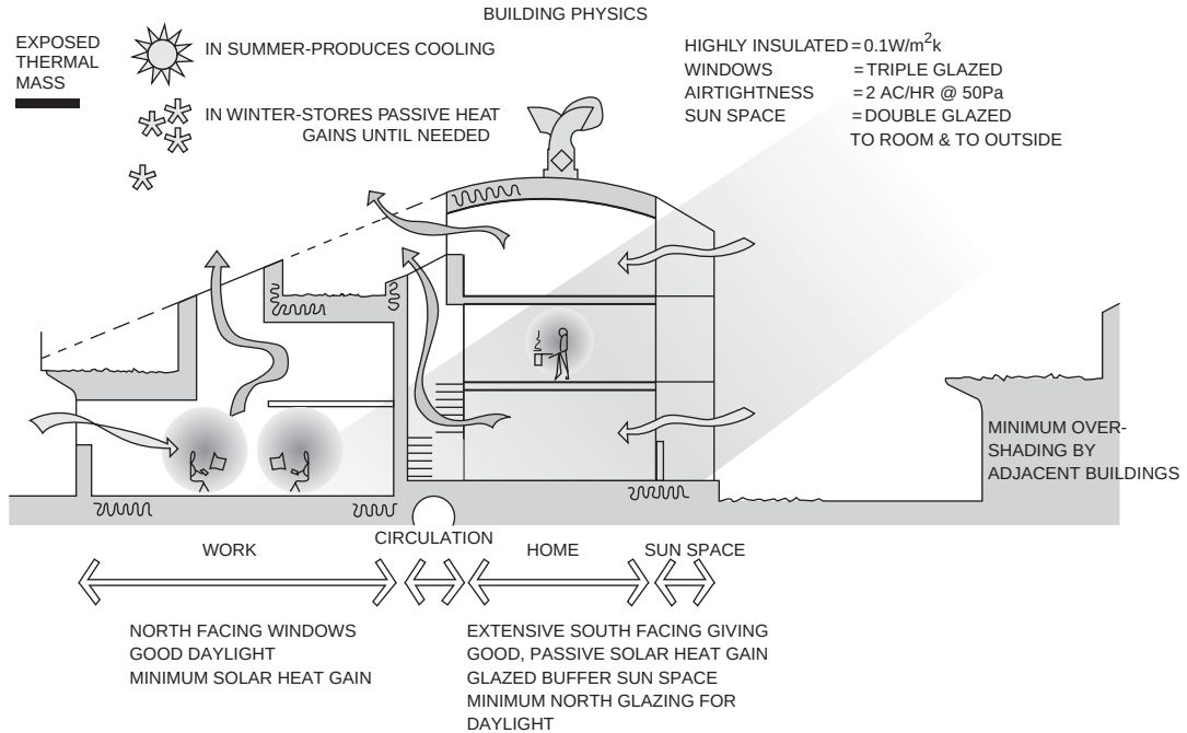
Figure 18.10 Section showing the passive features (courtesy of ARUP and BRE)
