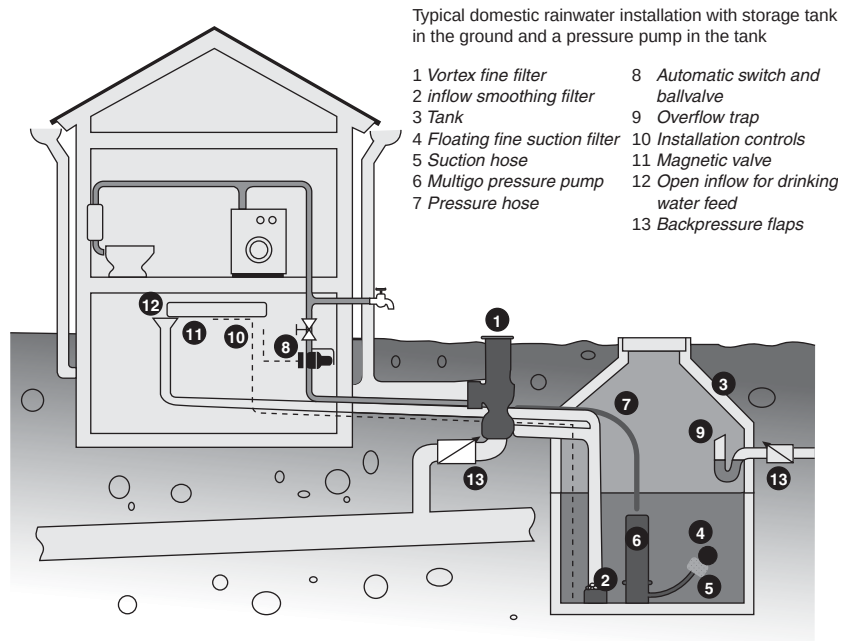
Figure 9.11 Rainwater storage system layout (courtesy of Construction Resources)
