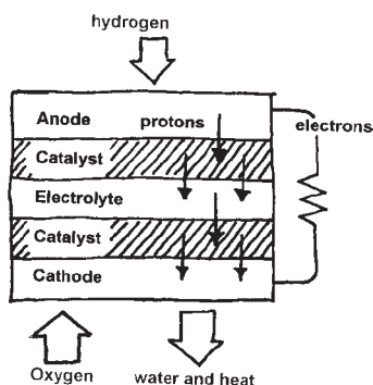
Figure 13.1 Basic structure and function of the proton exchange membrane fuel cell
