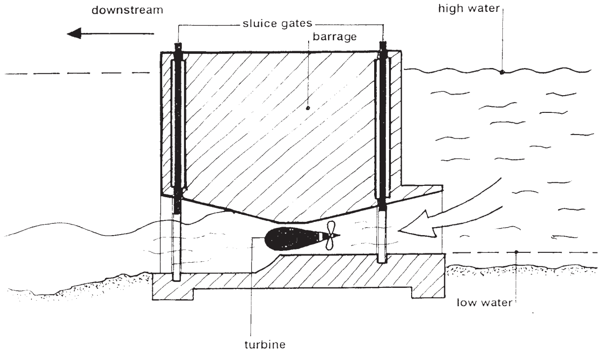
Figure 3.2 Basic tidal barrage
