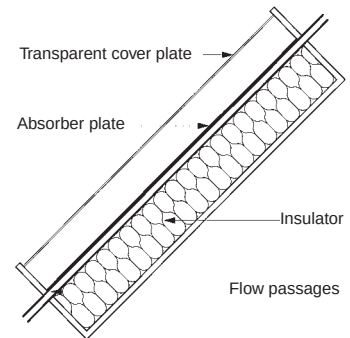
Figure 5.10 Flat plate collector
