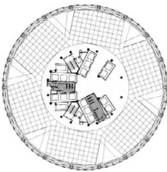
Figure 12.21 Upper floors with triangular atria
