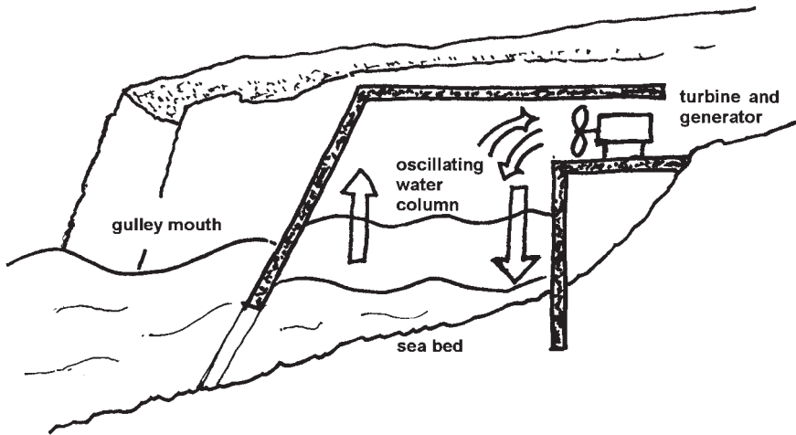
Figure 3.6 Principle of the Isle of Islay OWC wave generator
