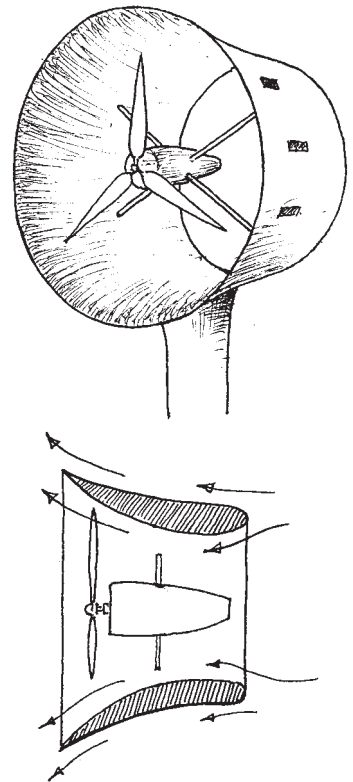
Figure 9.7 Wind turbine with cowling wind concentrator
