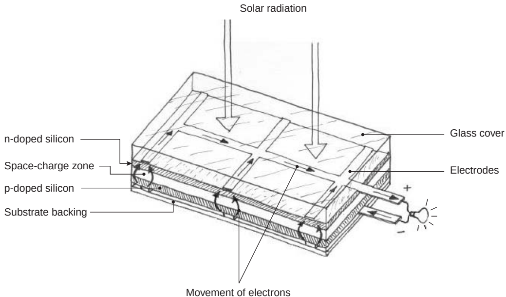
Figure 7.2 Photovoltaic cell structure and function
