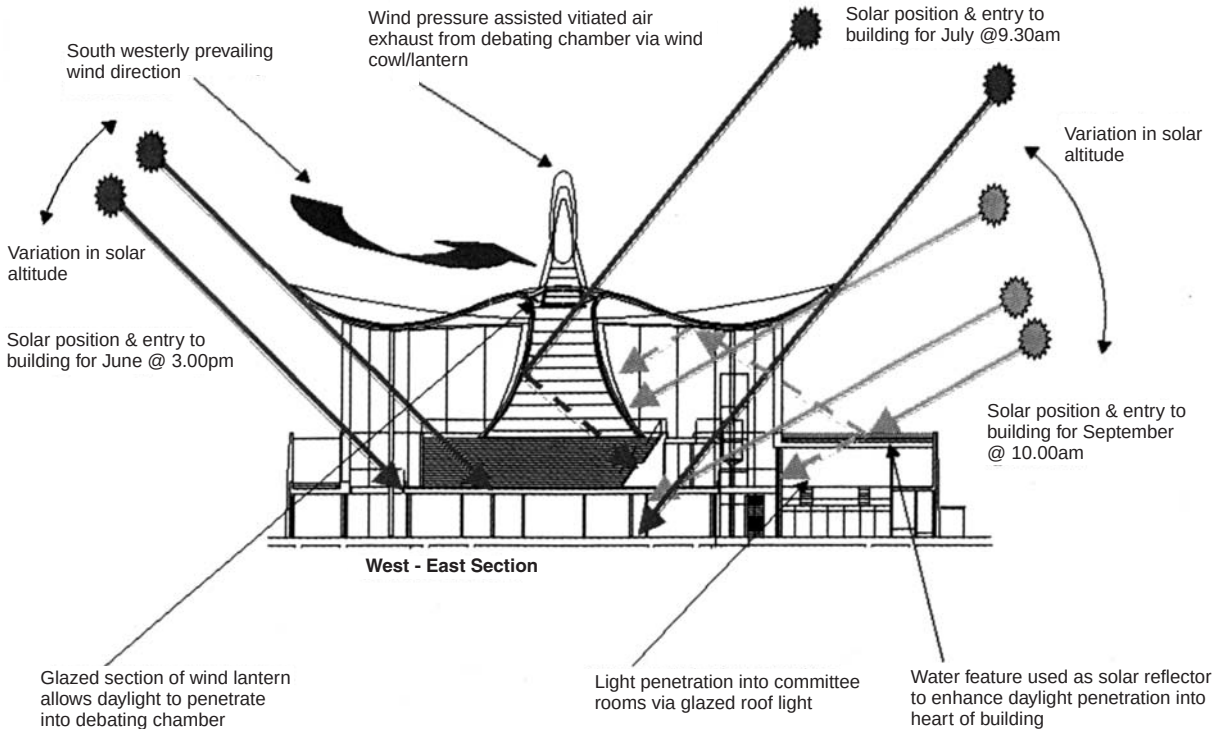
Figure 18.3 Welsh Assembly detail of natural light and ventilation
