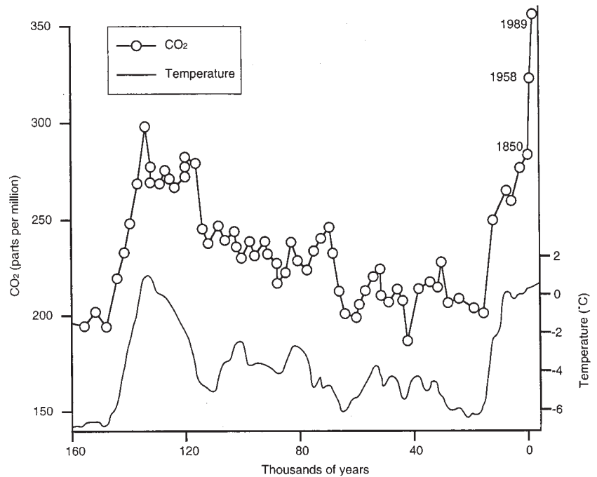
Figure 1.2 Correspondence between historic temperature and carbon dioxide
